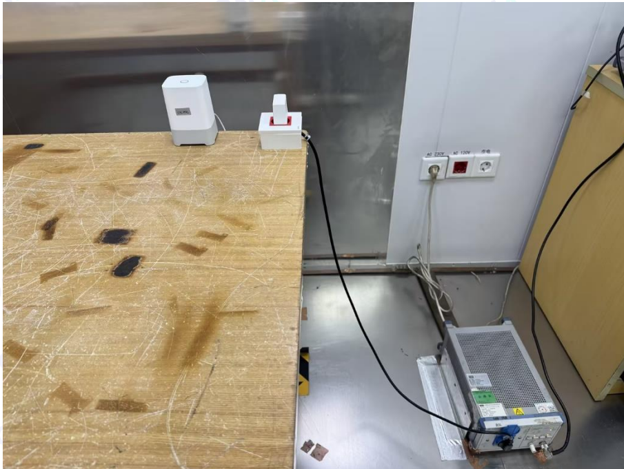
Conducted Emission Test Setup Adapter#2
