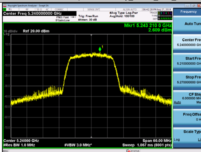
Maximum Power Spectral Density_TNVN_11A_5240
