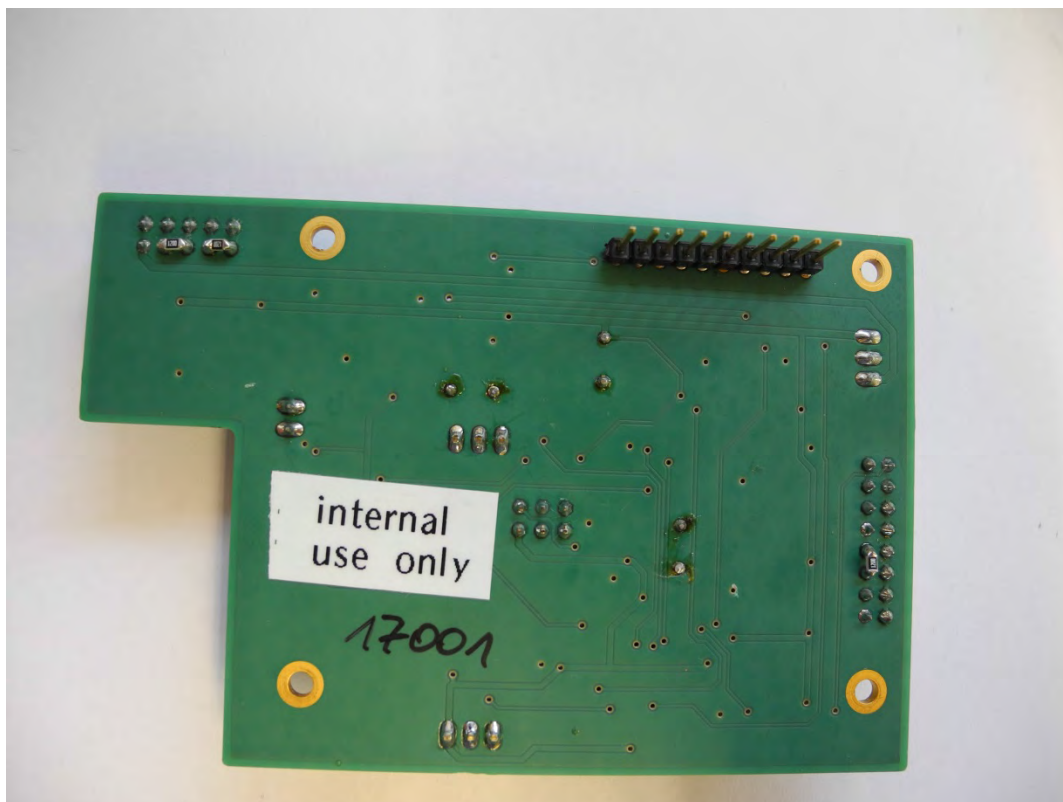
MTU-CONTROLLER – BOTTOM VIEW
