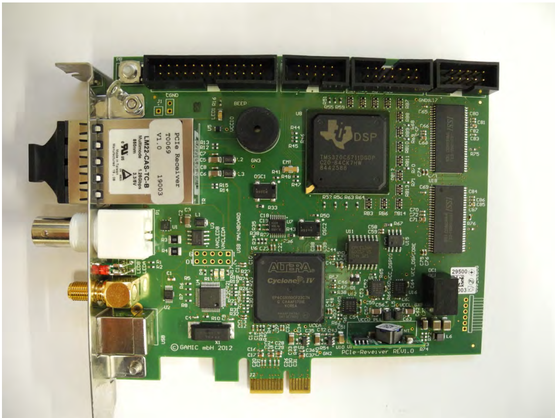
PCIE – RECEIVER – FRONT VIEW
