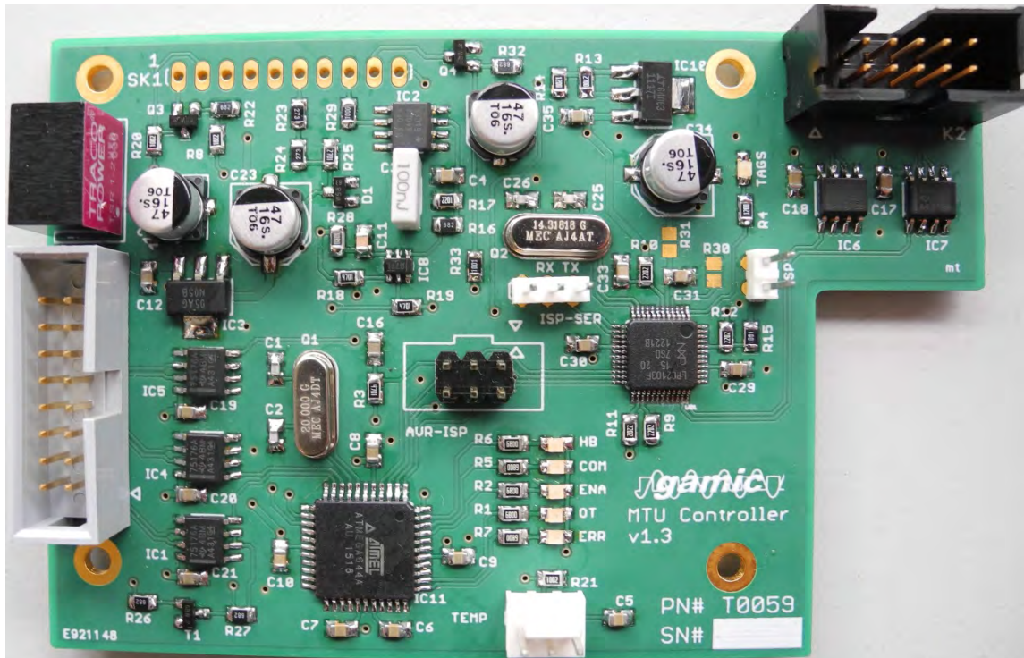
MTU – CONTROLLER – TOP VIEW
