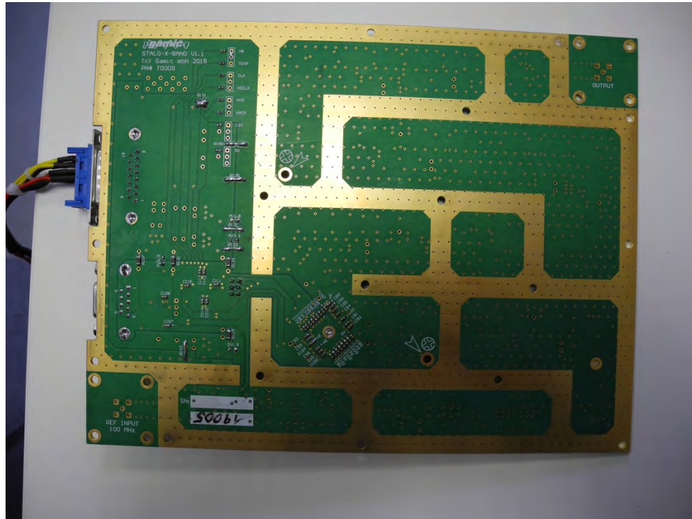
STALO – X-BAND – BACK VIEW
