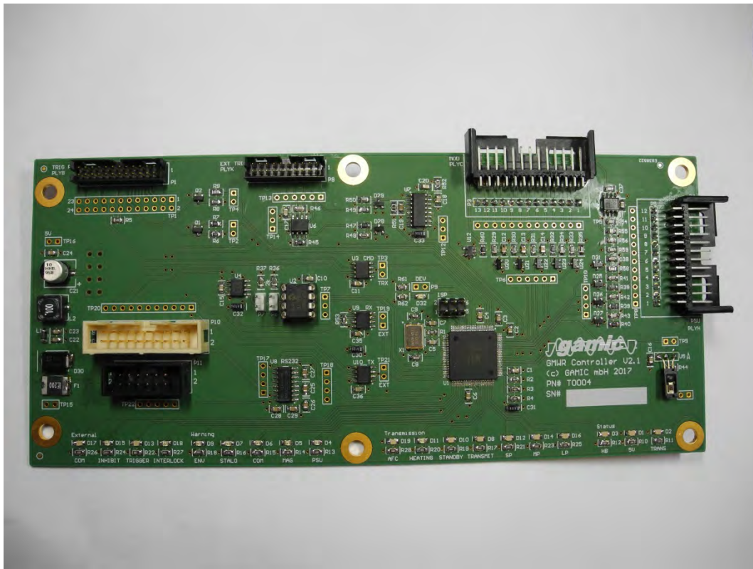
CONTROLLER – FRONT VIEW
