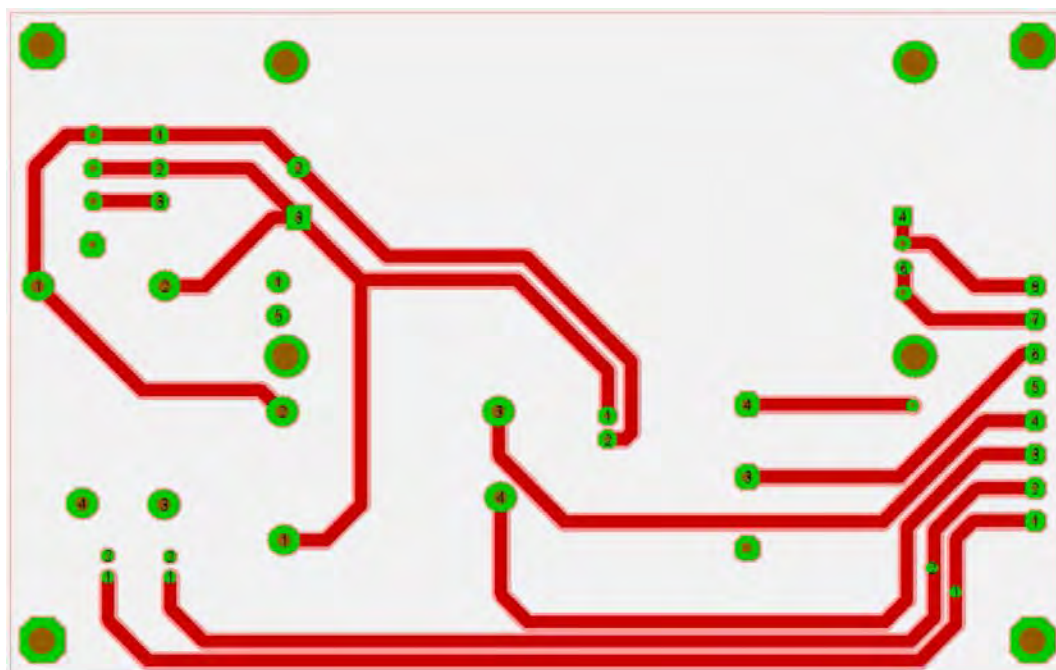
IFD-PSU – BACK VIEW
