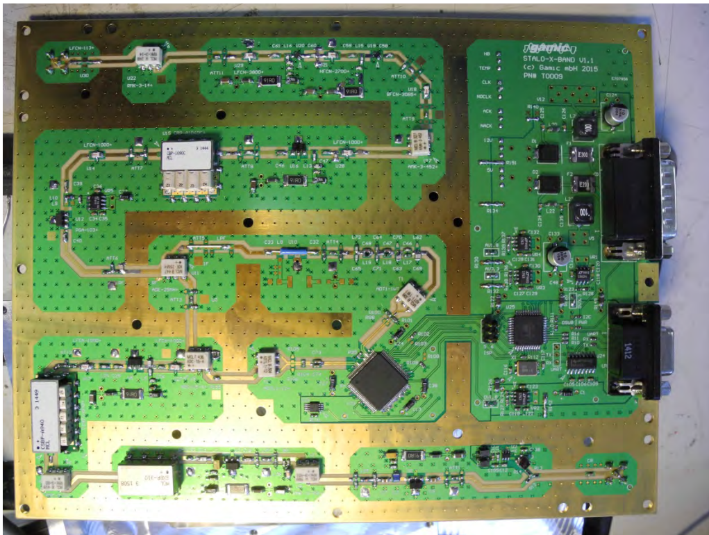
STALO – X-BAND – FRONT VIEW
