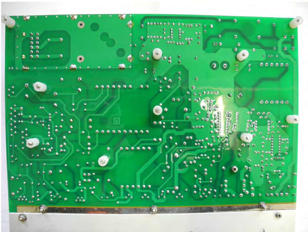
SPERRY- PSU BOARD –REAR VIEW
