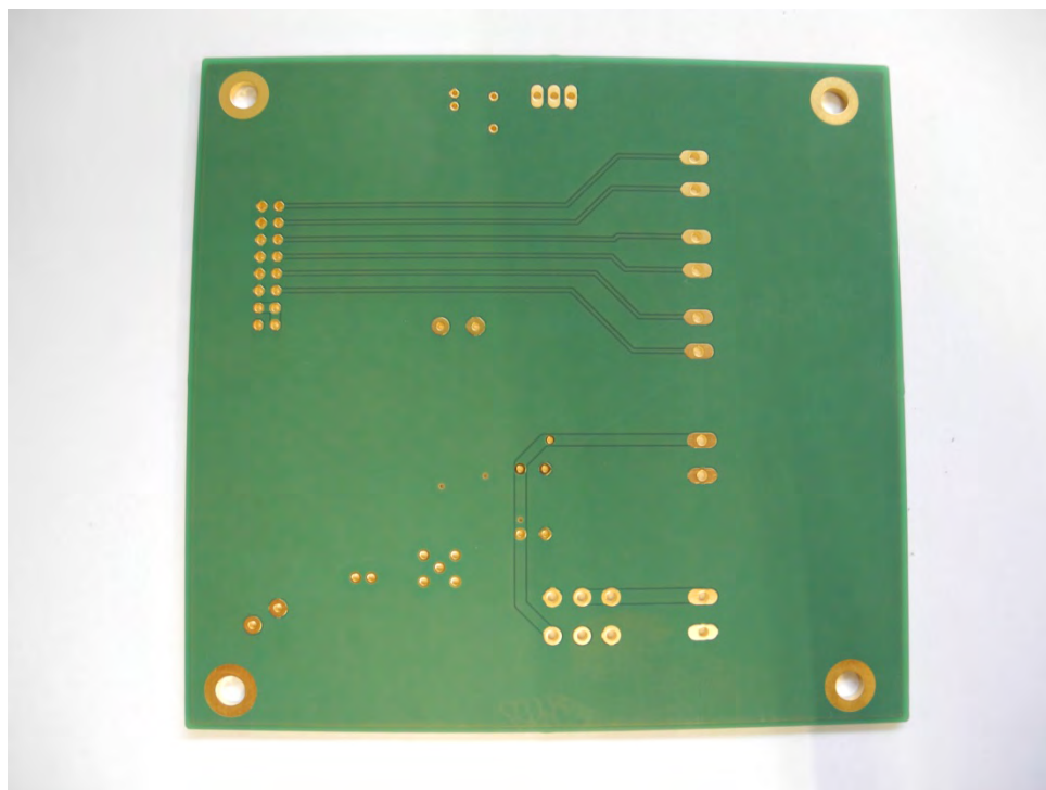
MTU – IO – BOTTOM VIEW
