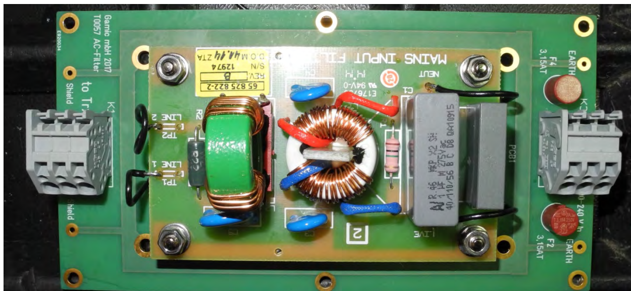
APS-AC-FILTER – TOP VIEW
