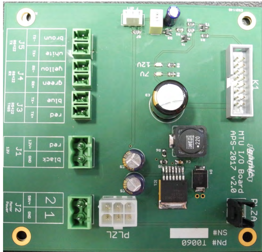
MTU – IO – FRONT VIEW
