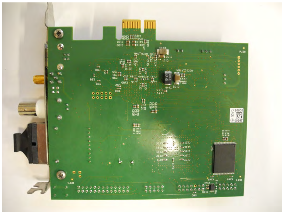
PCIE RECEIVER – BACK VIEW
