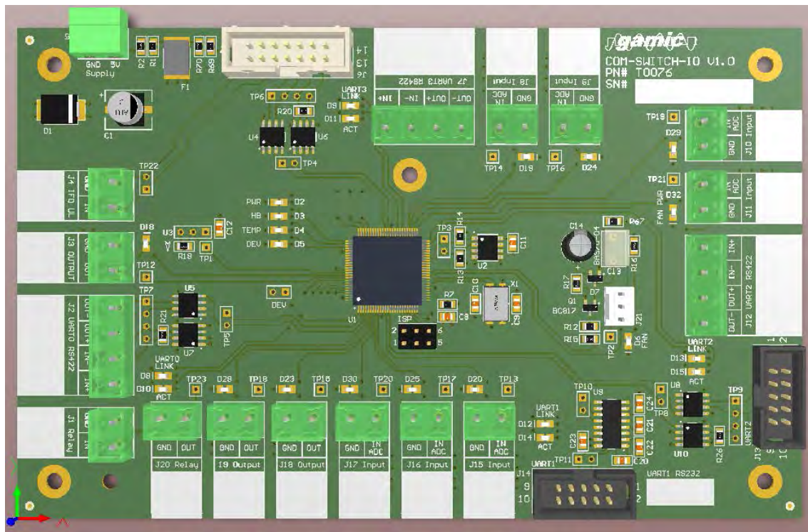
COM-SWITCH – IO – TOP VIEW
