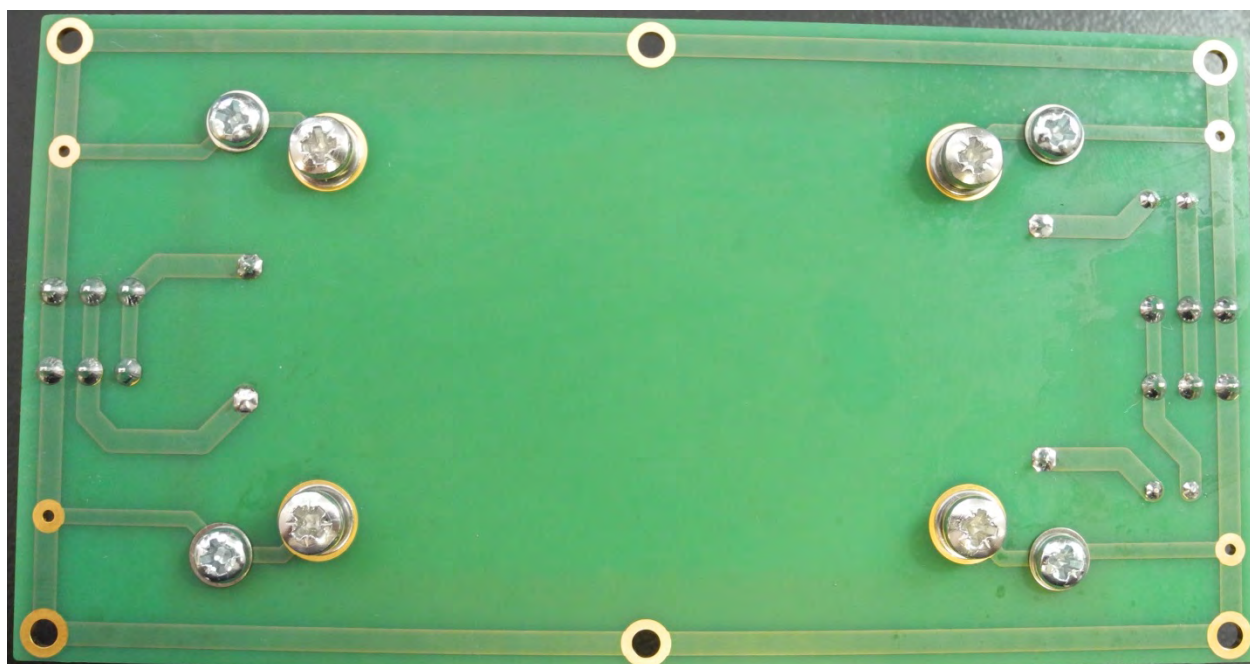
APS-AC-FILTER – BACK VIEW VIEW
