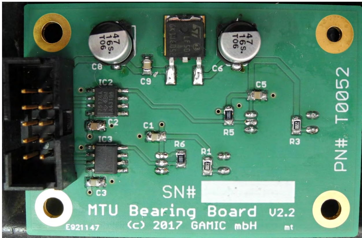
MTU – BEARING – TOP VIEW
