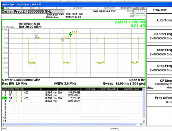
Dwell Time_GFSK_1M_DH5_2480MHz
