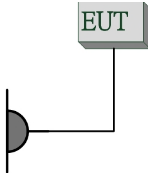
Fig. 2-2 Conduction test set up configuration
