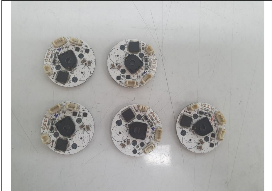
Top view of Sub PCB2_package
