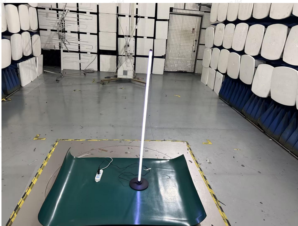
Test Setup Photo of Line Conducted Emissions Measurement
