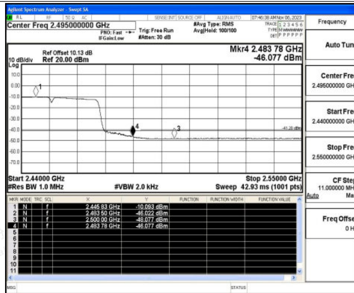
11N40ISO_Ant1_High_2452_Peak
