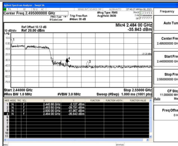
11N40ISO_Ant1_High_2452_Peak
