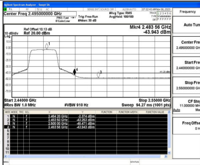
11N20ISO_Ant1_High_2462_Peak
