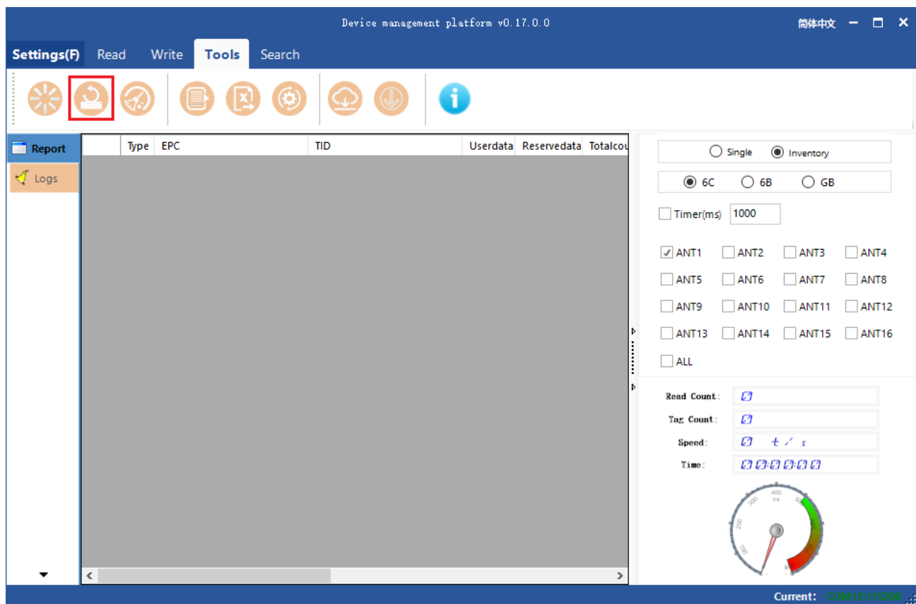
Figure 4.9.2.1 Factory Reset
