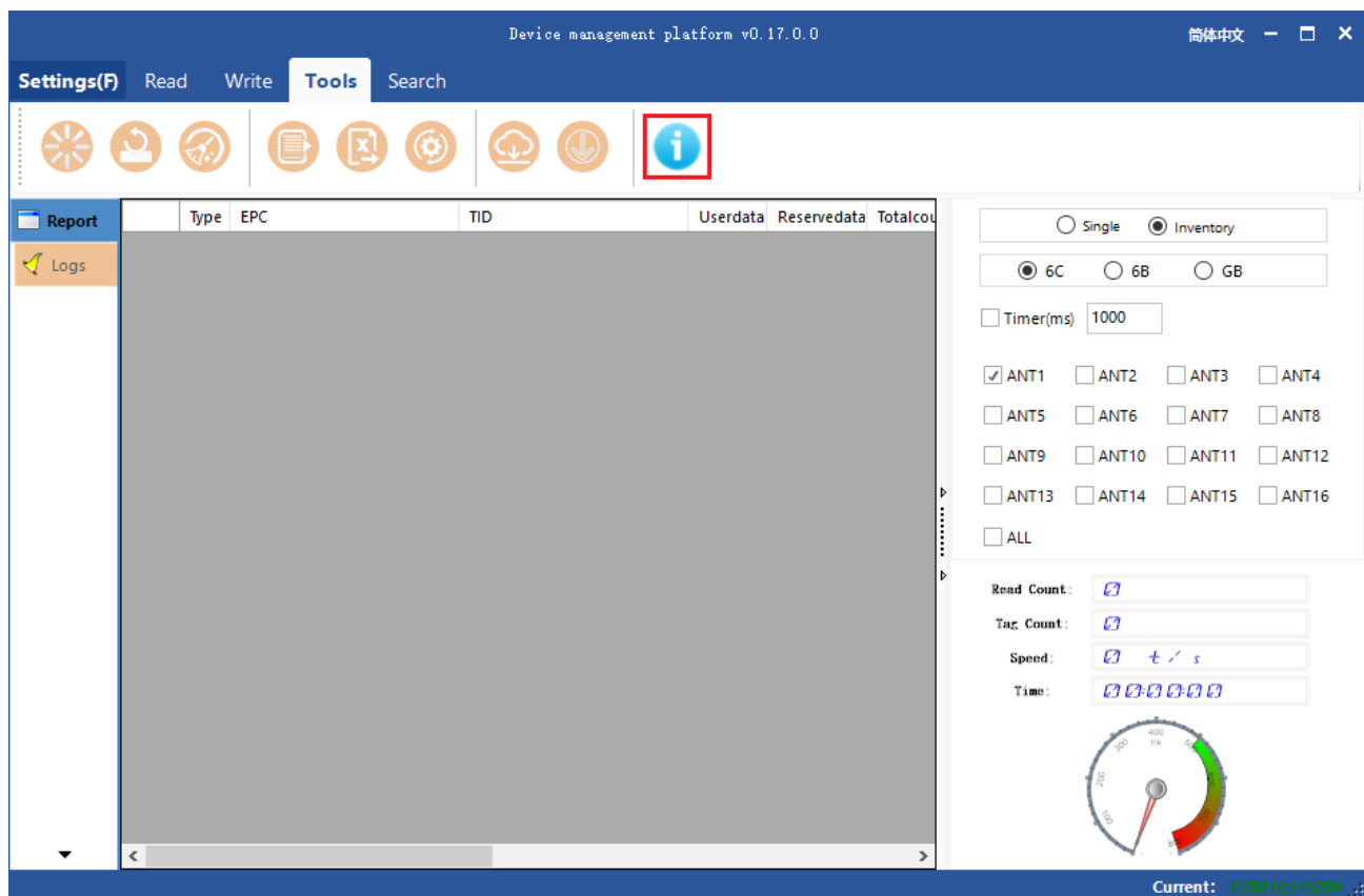
Figure 4.9.6.1 Device Info
