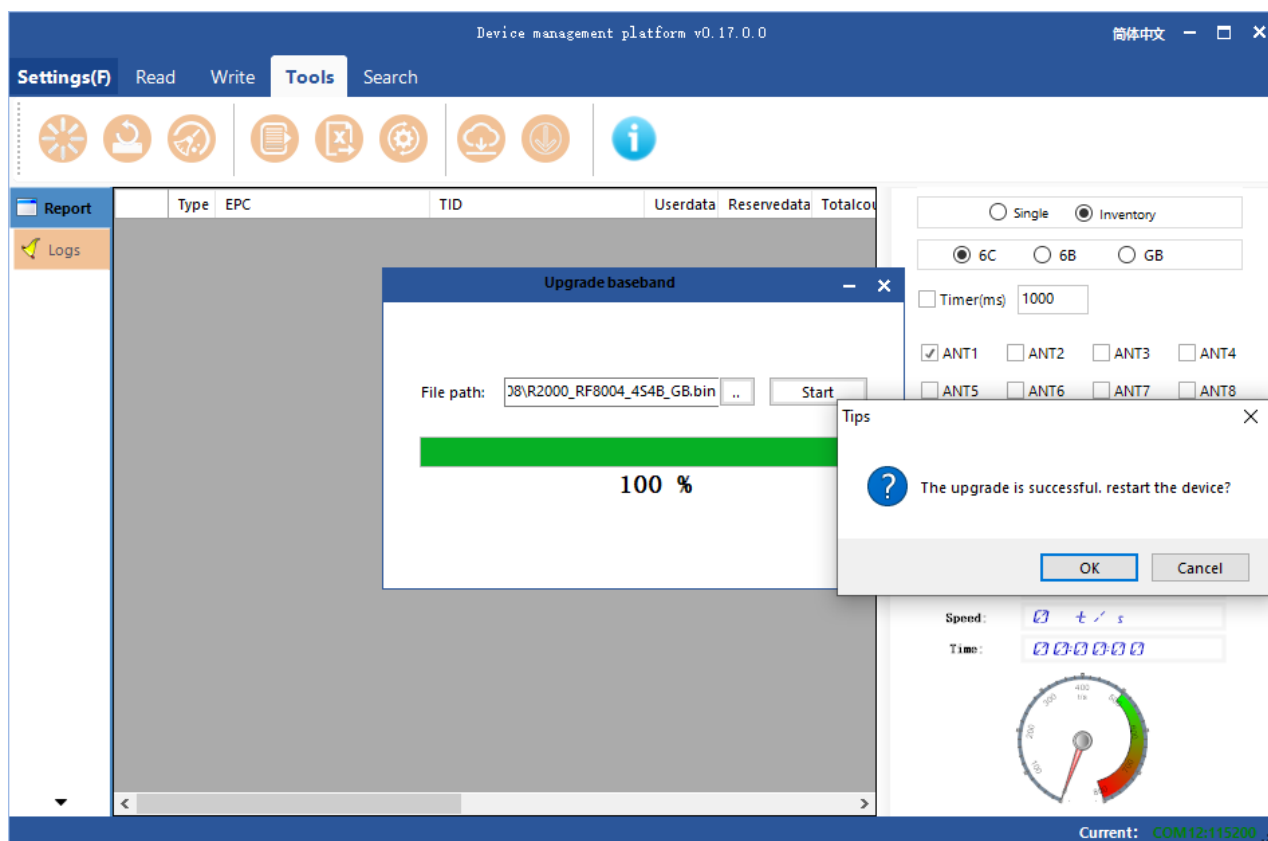
Figure 4.9.4.4 Restart Confirm
