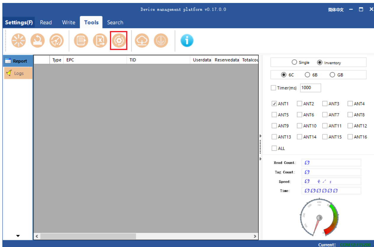
Figure 4.9.5.1 Custom Command
