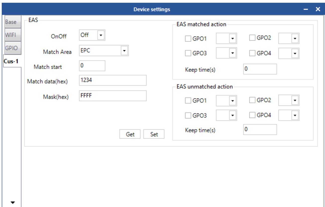
Figure 4.8.3 EAS Alarm
