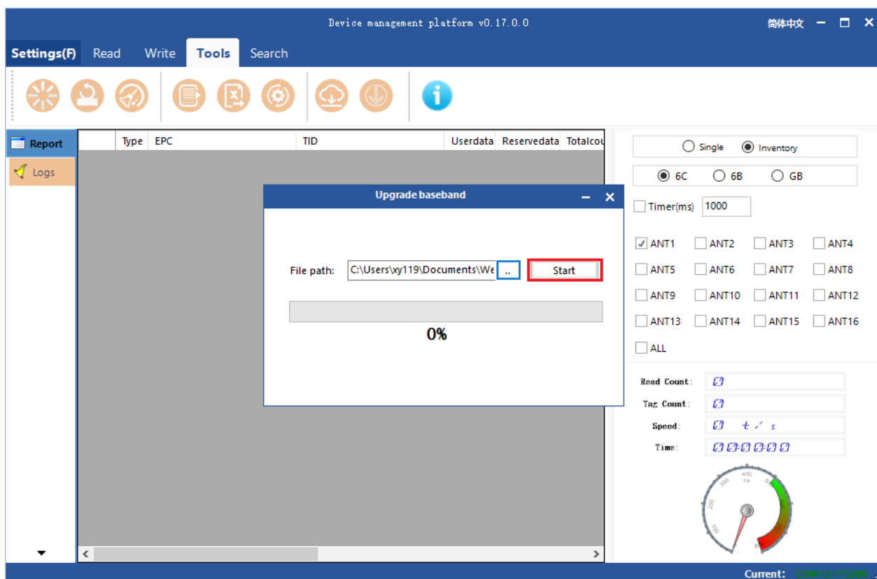
Figure 4.9.4.3 Upgrading baseband
