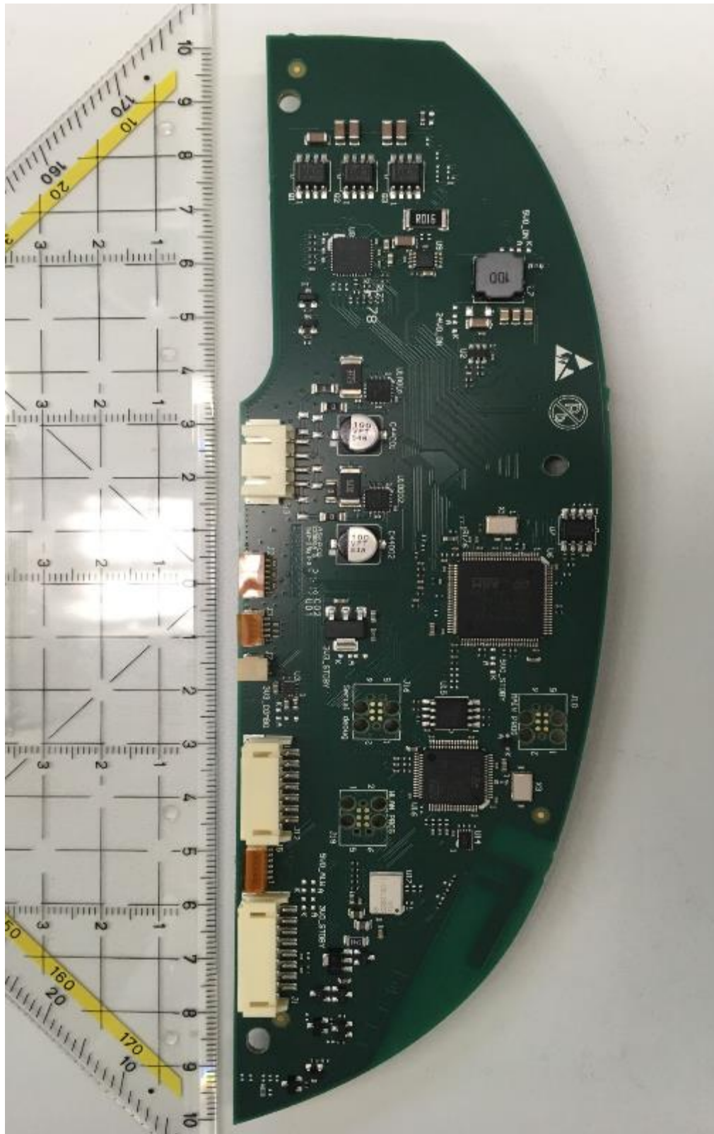
Main Board Top Side View
