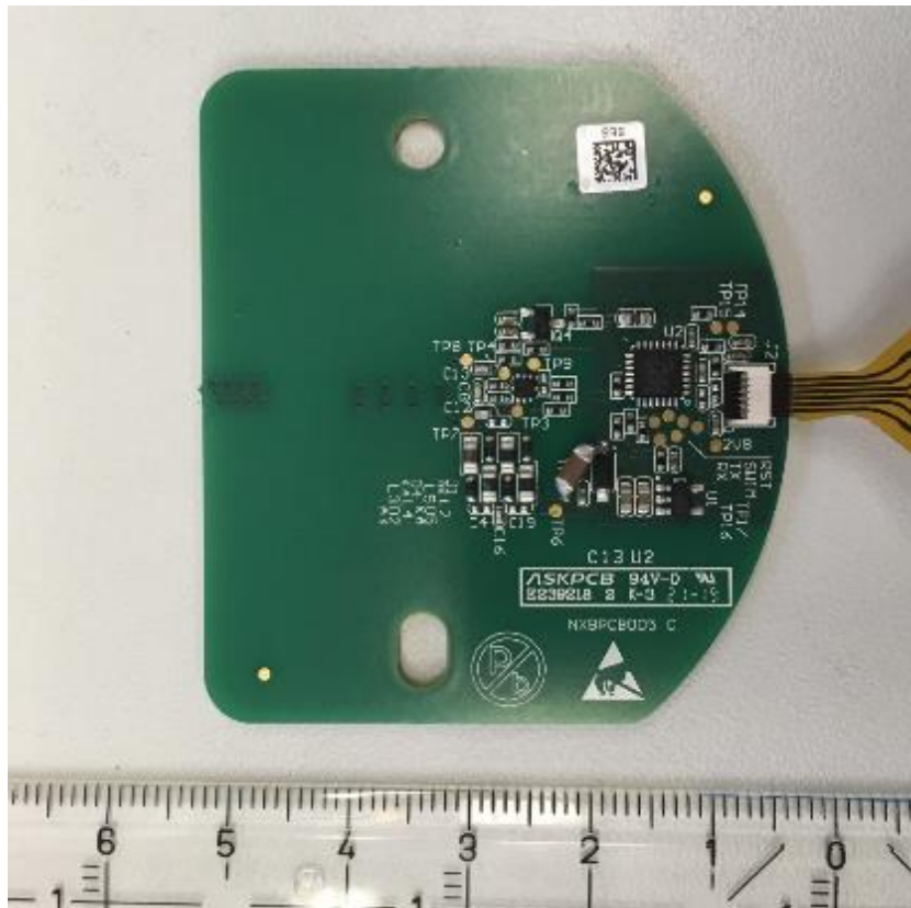
NFC: Sensor Station Board Top Side View
