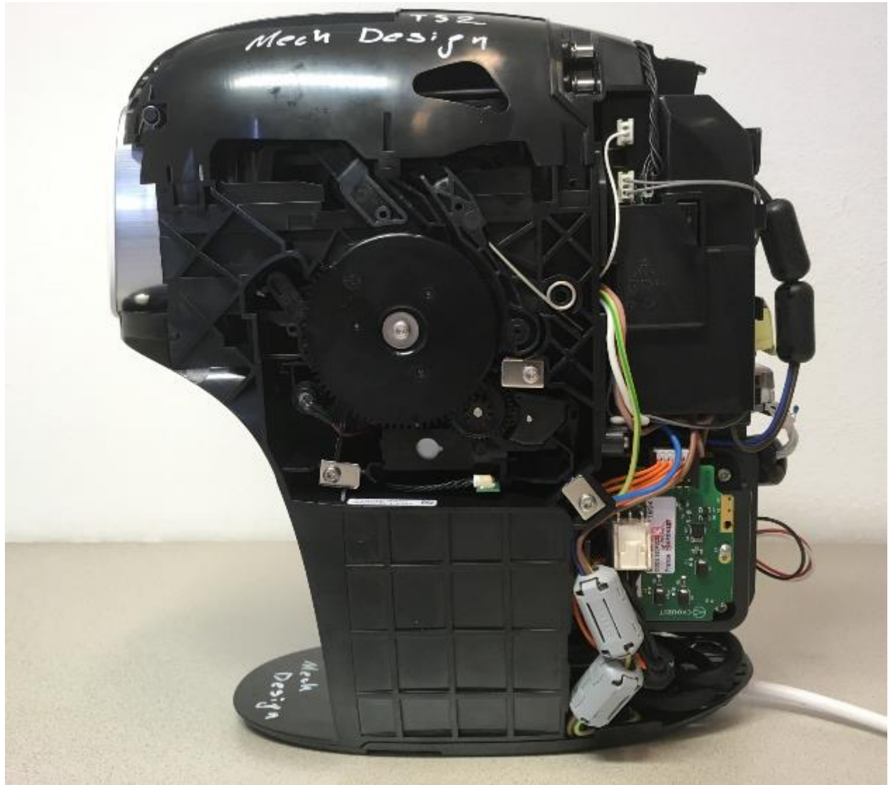
Right side view without cover
