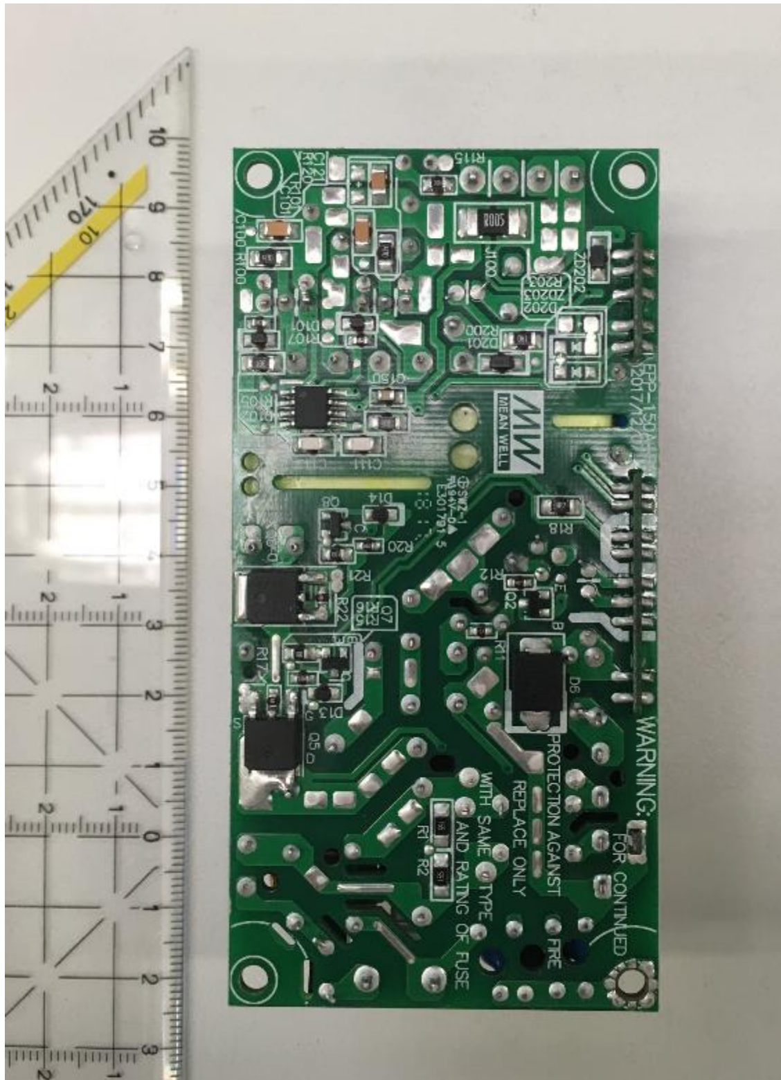
Power Supply Unit Bottom Side View
