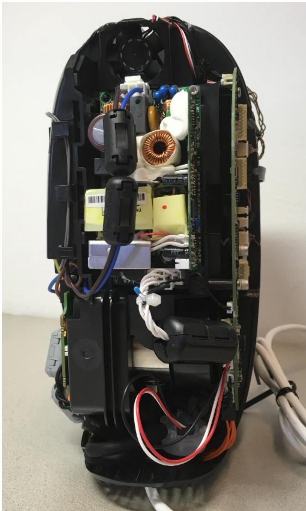
Rear side view without cover Nespresso, Type: O by Nespresso
