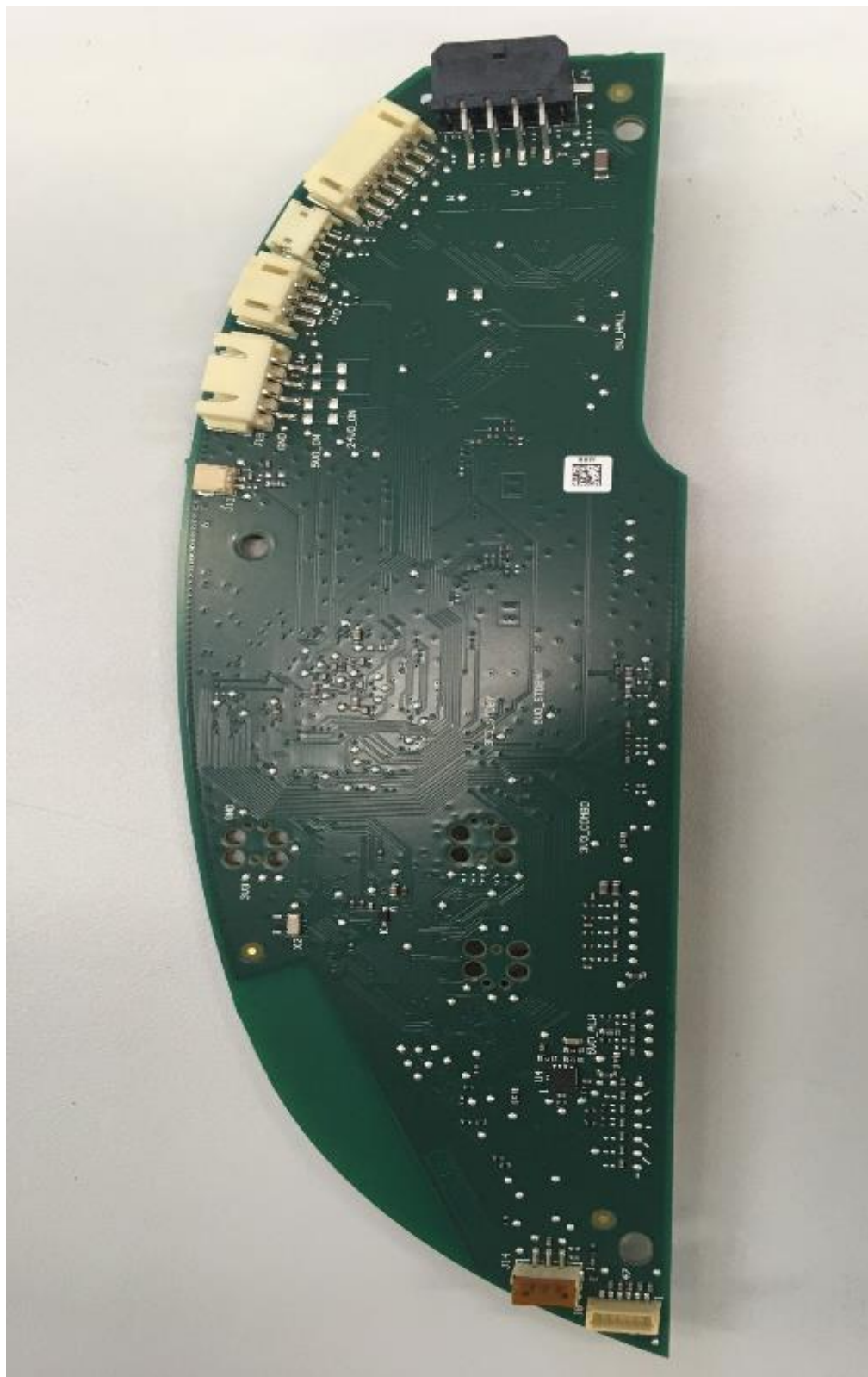
Main Board Bottom Side View
