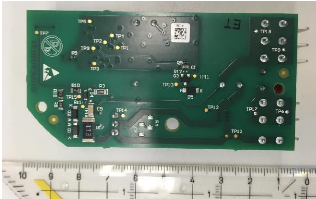
AC Main Board Bottom Side View
