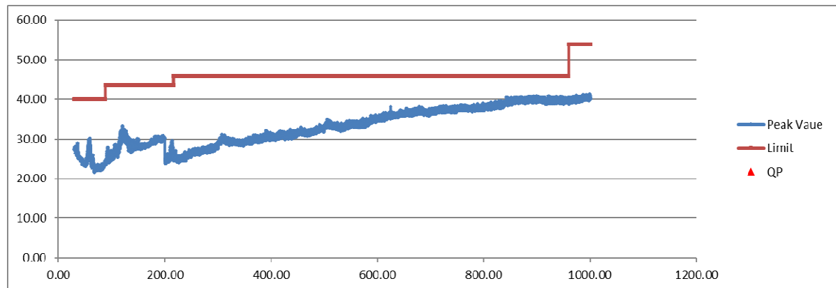
Figure 27. Radiated Emissions Graphical Data, TX, 30-1000 MHz – Vertical
