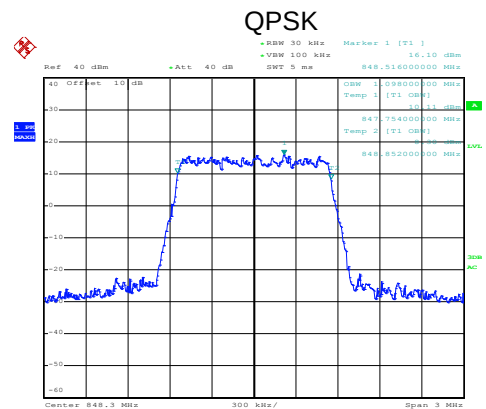
LTE Band 5: 99% Occupy bandwidth BW: 1.4MHz
