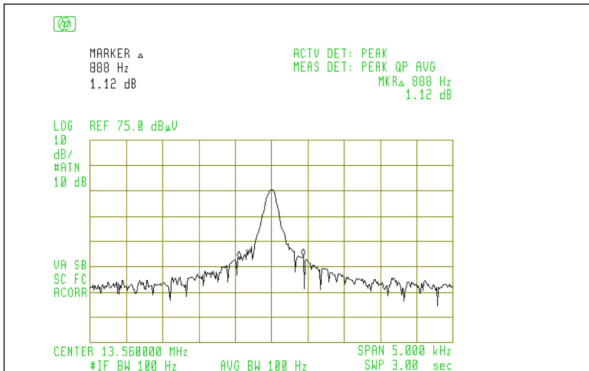
Figure 6.1 Occupied Bandwidth
