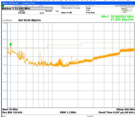
Plot # 8. Emissions scan 30 - 900 MHz.
