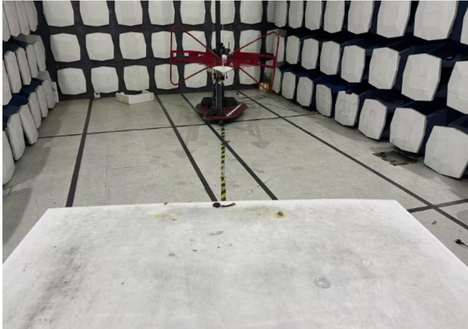
Radiated Disturbance (Up to 1GHz)
