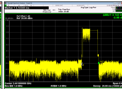
2441MHzDH5
