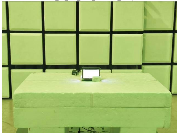
FCC_15_225_NFC_Radiated_Setup
