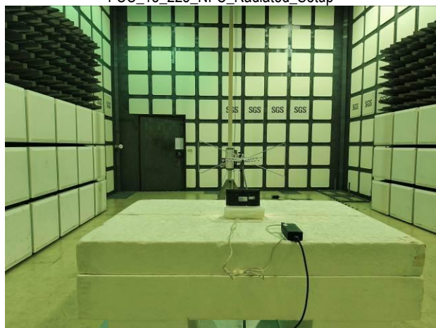
FCC_15_225_NFC_Radiated_Setup
