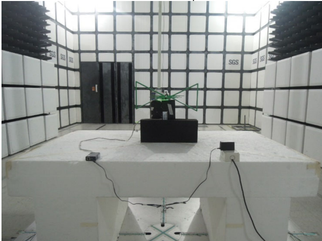
Radiated_Setup
