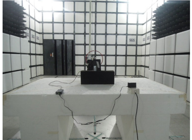
Radiated_Setup
