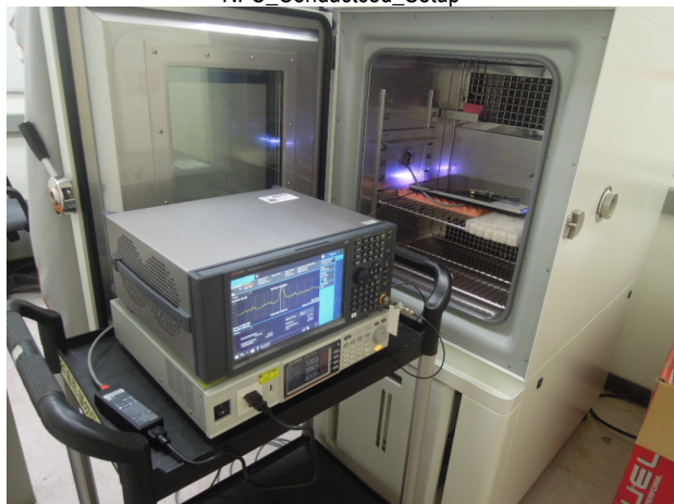
NFC_Conducted_Setup
