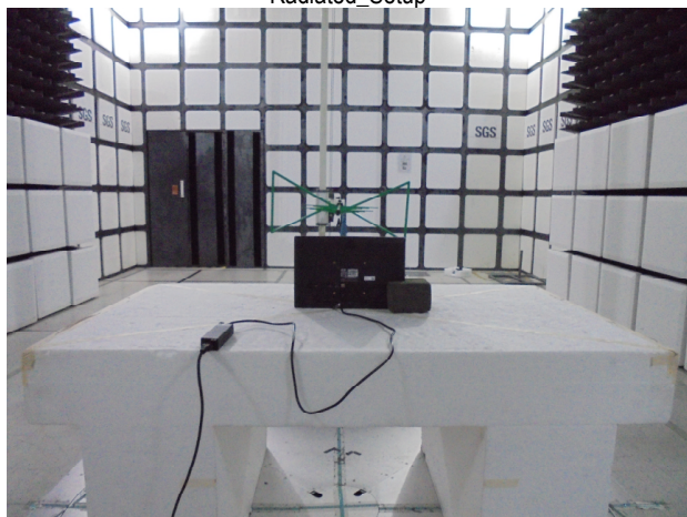
Radiated_Setup
