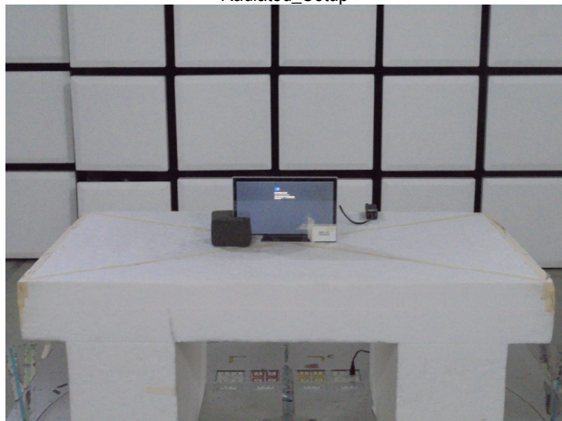
Radiated_Setup
