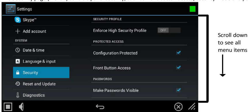
FIG. 94 Security page
