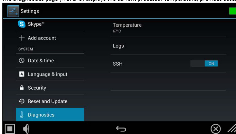
FIG. 143 Diagnostics page
