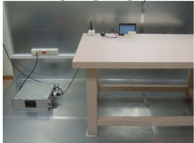
FCC_Part15.225_Conduction_Setup
