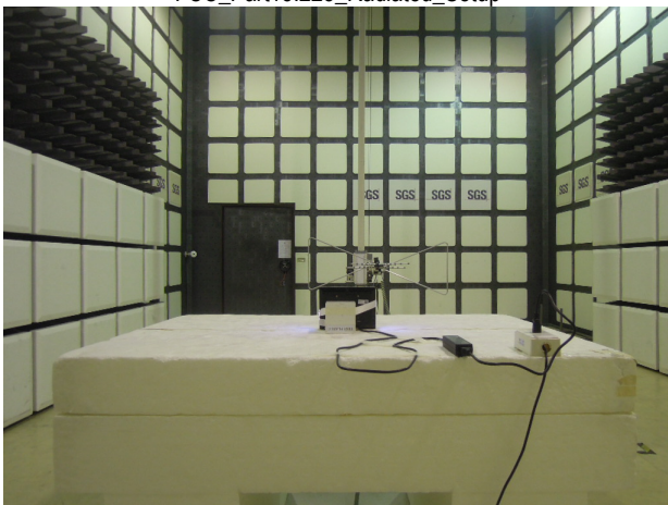
FCC_Part15.225_Radiated_Setup
