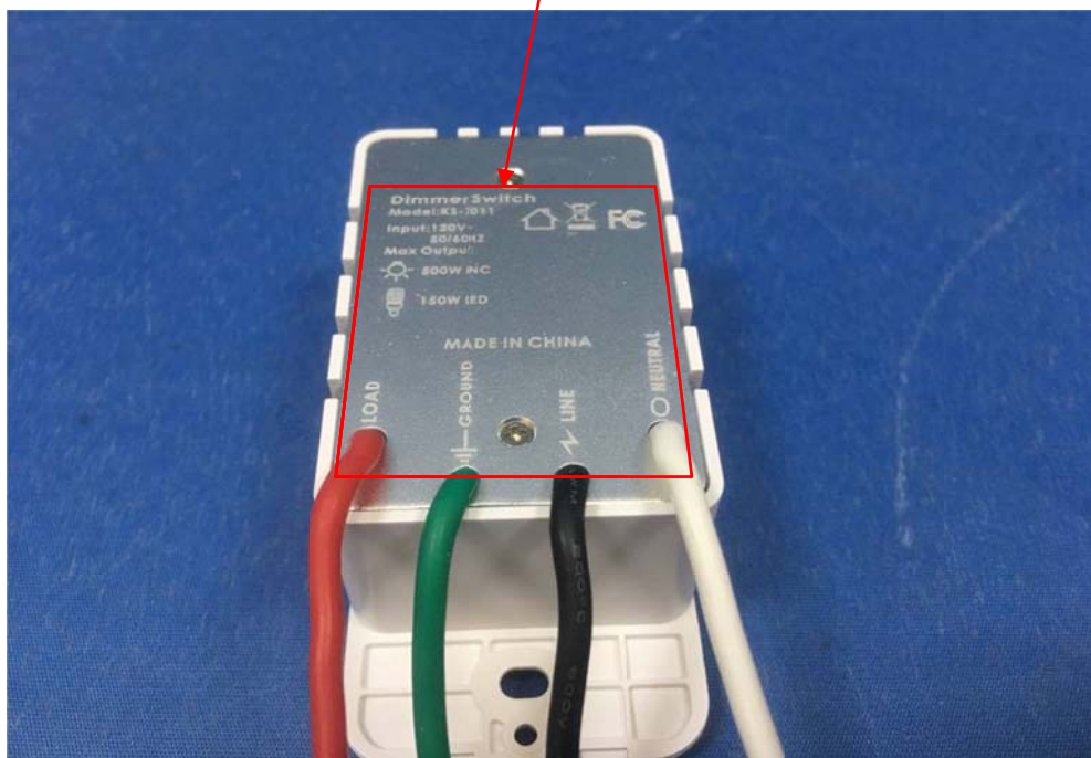
FCC ID Label Location
