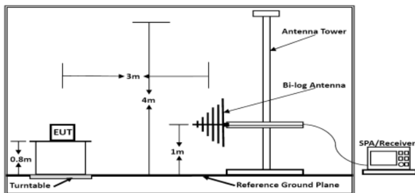
Below 1GHz
