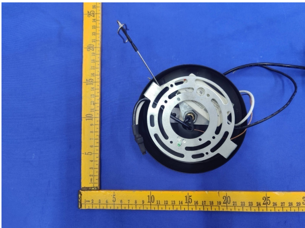
Fig.4(Model: PDT-DAC)
