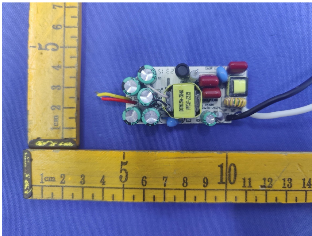
Fig.9(Model: PDT-DAC )
