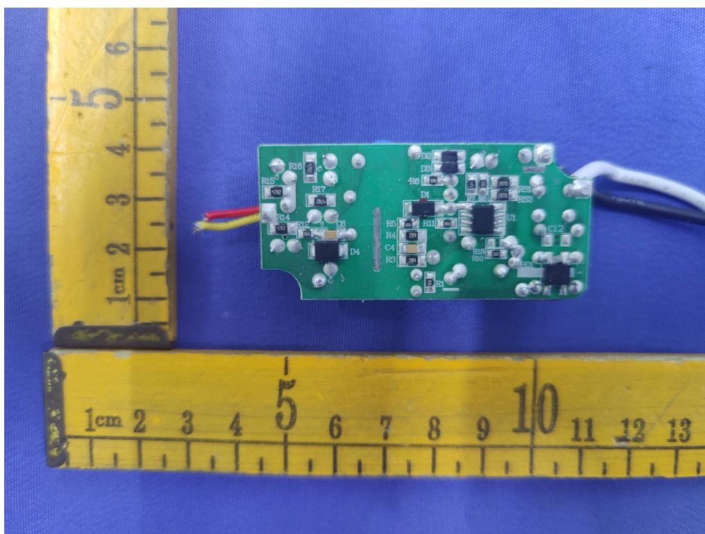
Fig.10(Model: PDT-DAC )
