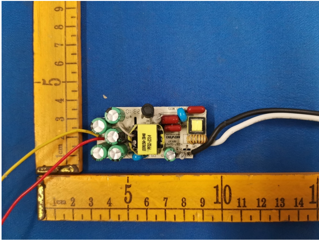
Fig.5(Model: PDT-PL )
