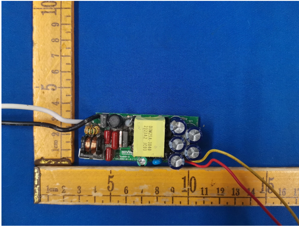
Fig.5(Model: PDT4-VI5C )
