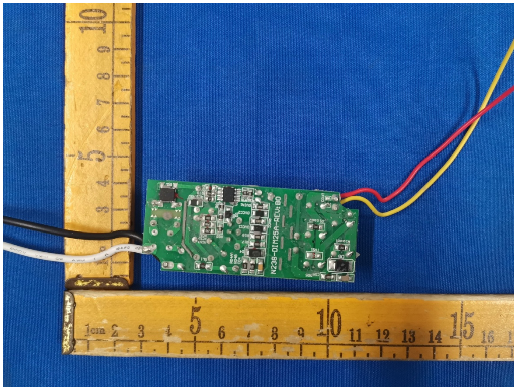
Fig.6(Model: PDT4-VI5C )
