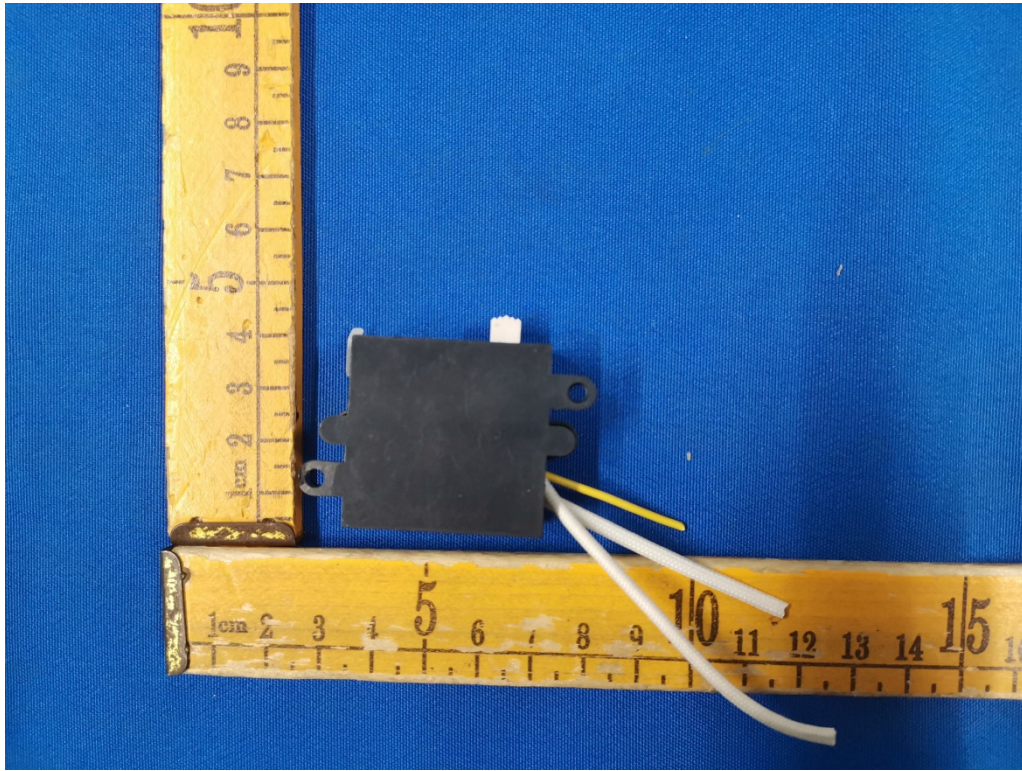
Fig.9(Model: PDT4-VI5C )
