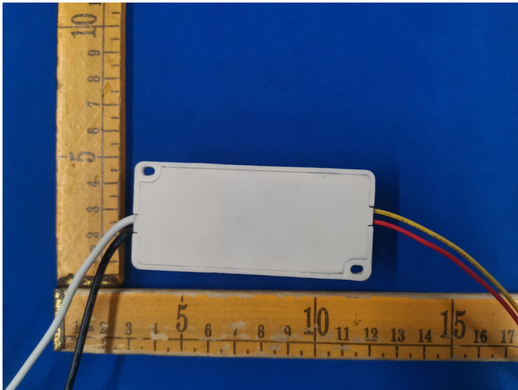
Fig.4(Model: PDT4-VI5C)
