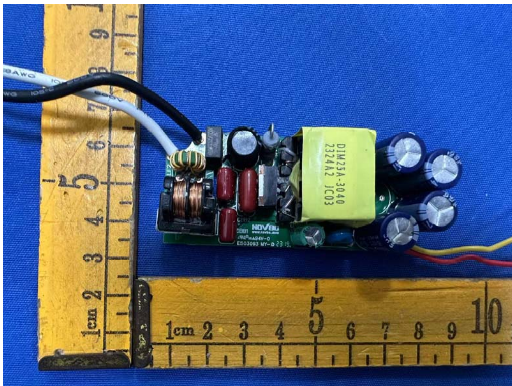
Fig.5(Model: PDT-DL )
