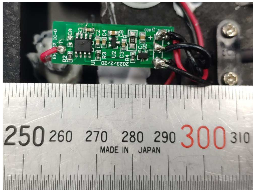
PCB View
