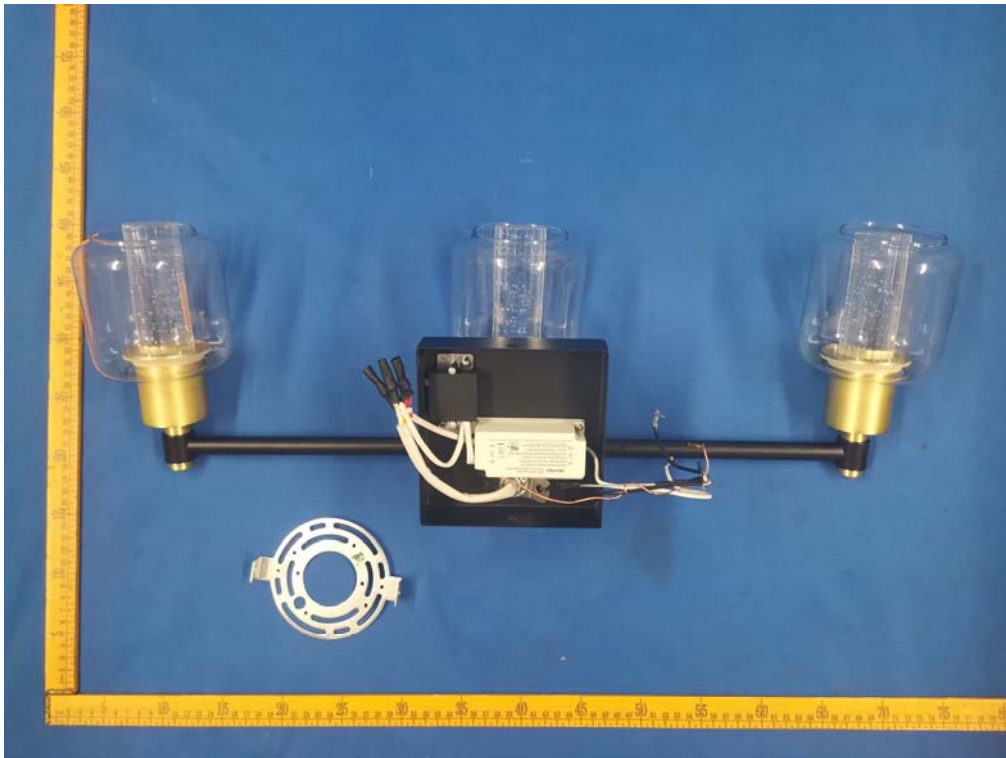
Fig.5 (Model: VAN3-CG5C)
