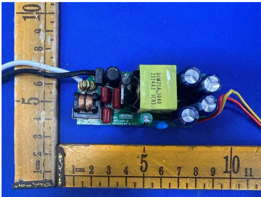
Fig.4(Model: VAN-SWR )
