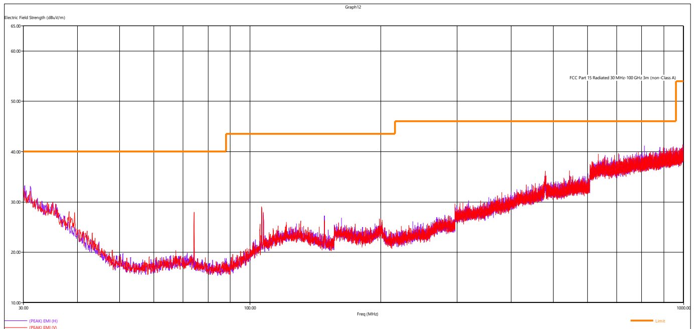
Figure 8 - Radiated Emissions Plot, Transmitter Off, 30 MHz-1GHz
