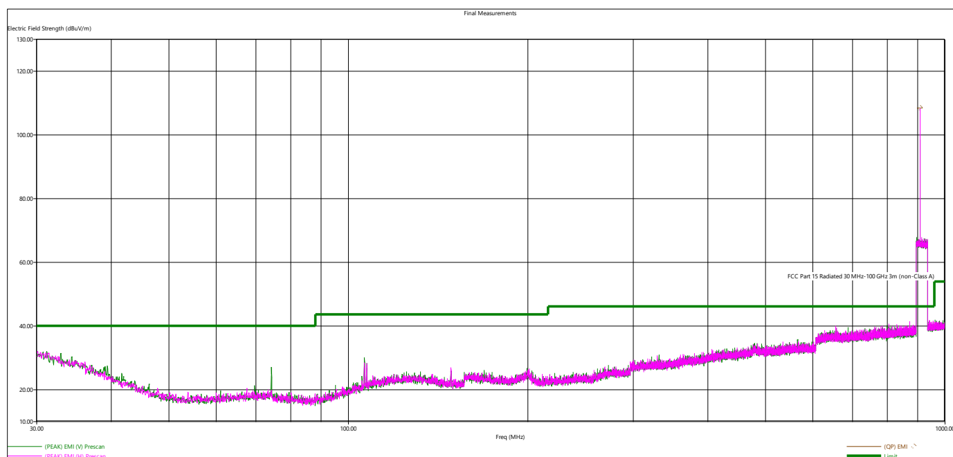
Figure 6 - Radiated Emissions Plot, Mid Channel, 30 MHz-1GHz
