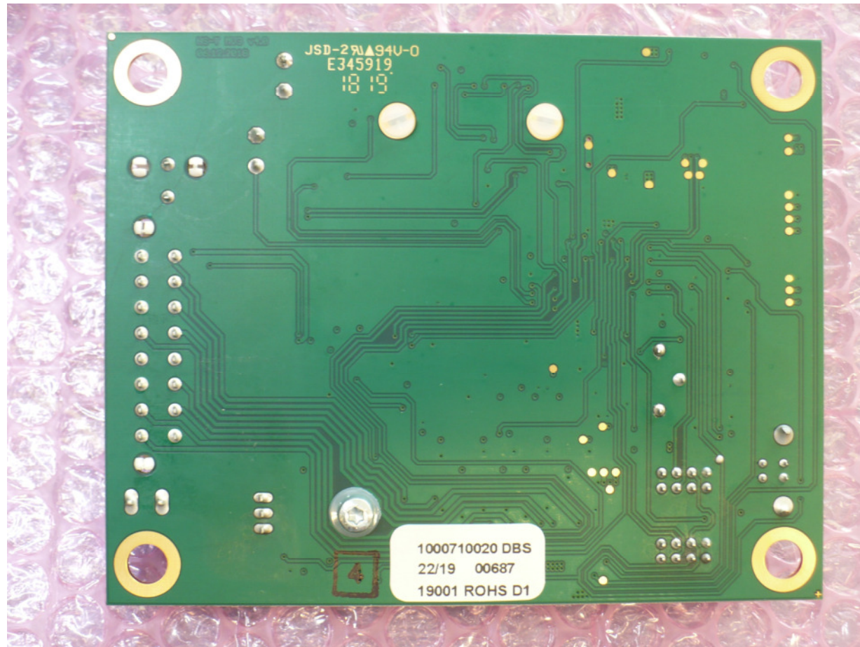
HST-MV3-04W-US PCB bottom view
