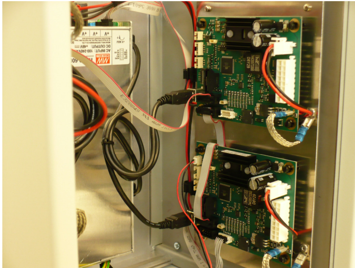
HST-MV3-04W-US side view right
