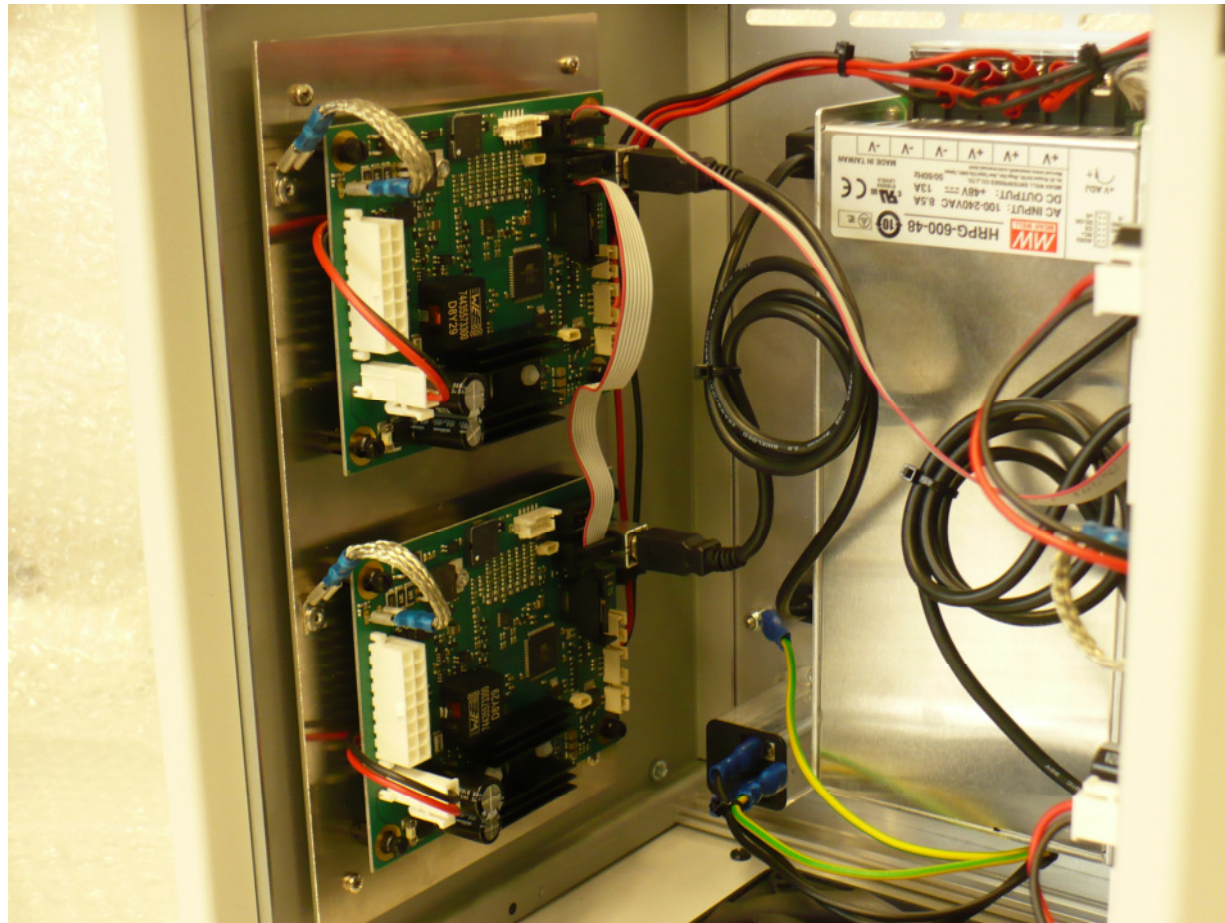
HST-MV3-04W-US side view left
