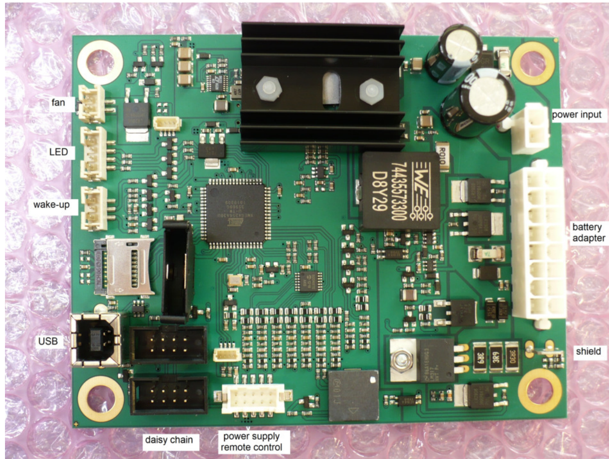
HST-MV3-04W-US PCB top view
