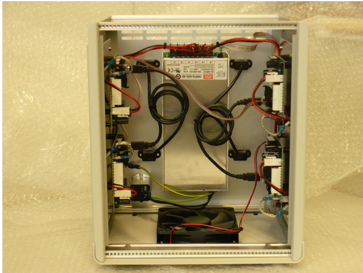
HST-MV3-04W-US rear plate view
