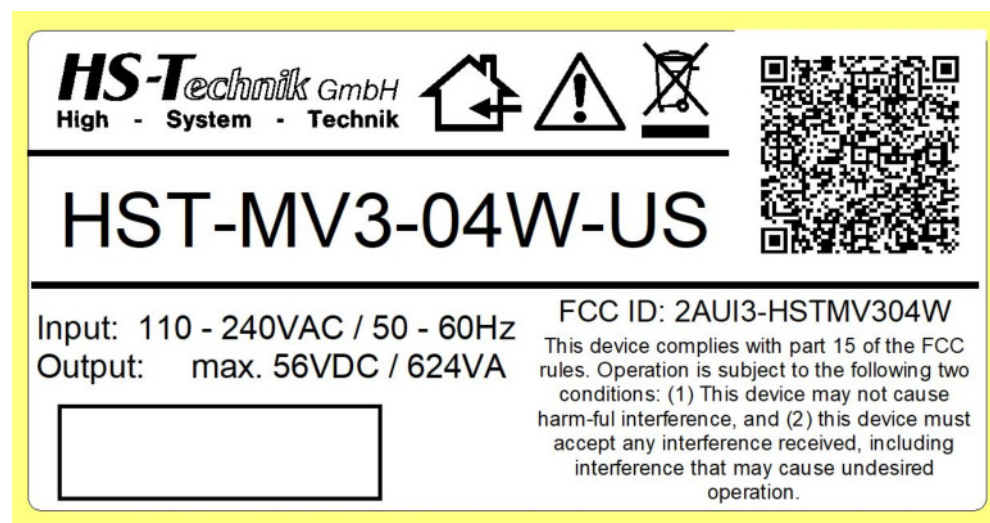
HST-MV3-04W-US name plate with FCC ID
