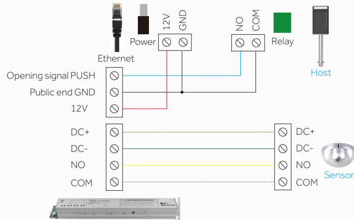
Controller of auto-door (only used terminals will be listed)
