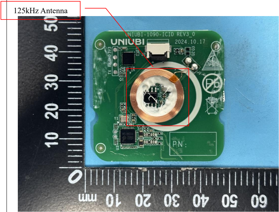
Antenna View 2
