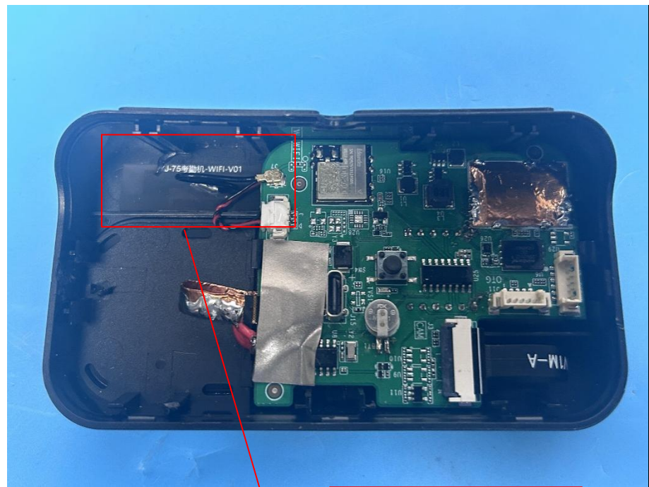
WIFI/Bluetooth Antenna
