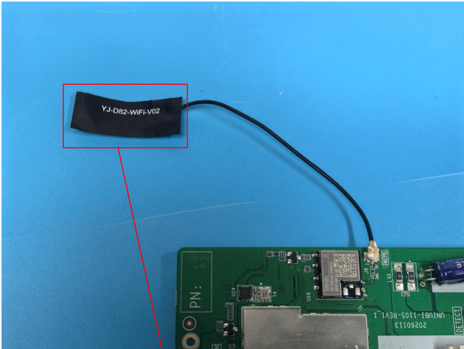
WIFI/Bluetooth Antenna
