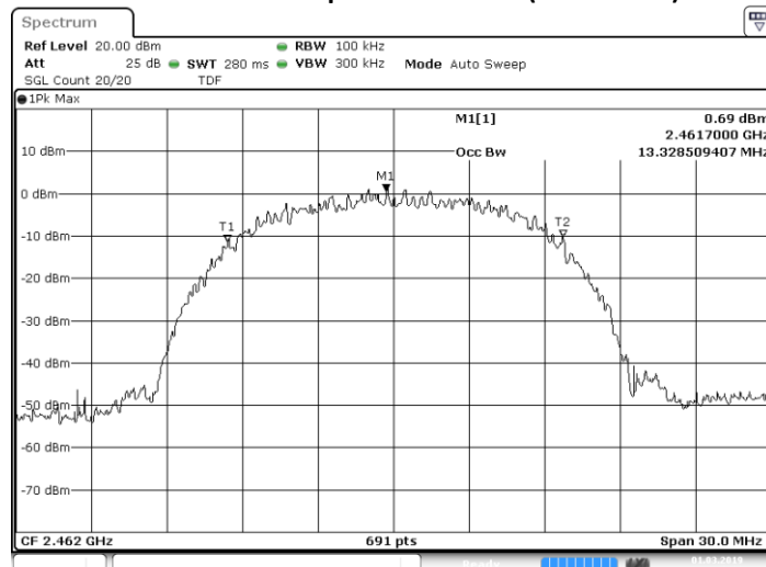
802.11b 99% Occupied Bandwidth (Channel 11)
