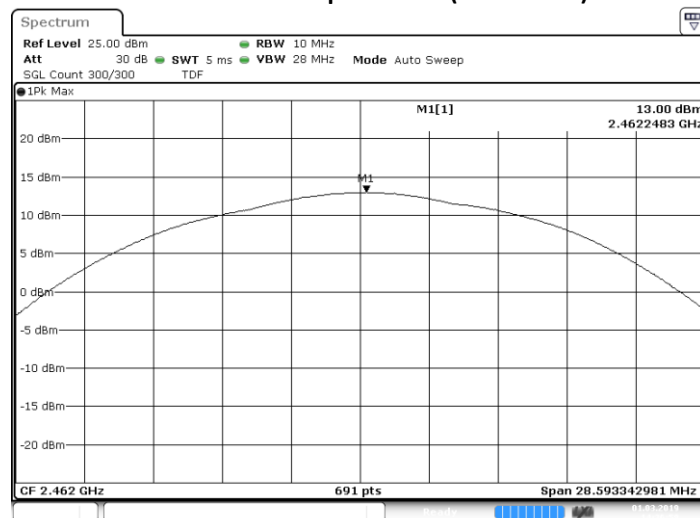
802.11b Peak Output Power (Channel 11)
