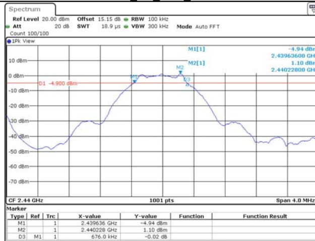
BLE_1M_Ant1_2440
