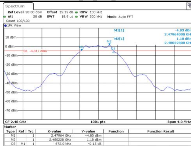
BLE_1M_Ant1_2480
