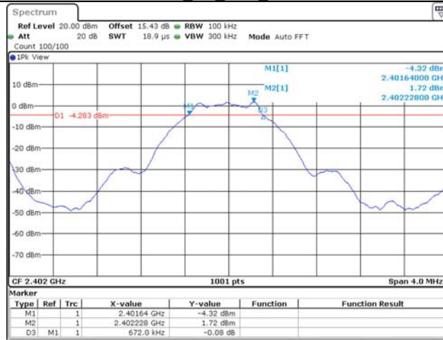
BLE_1M_Ant1_2402
