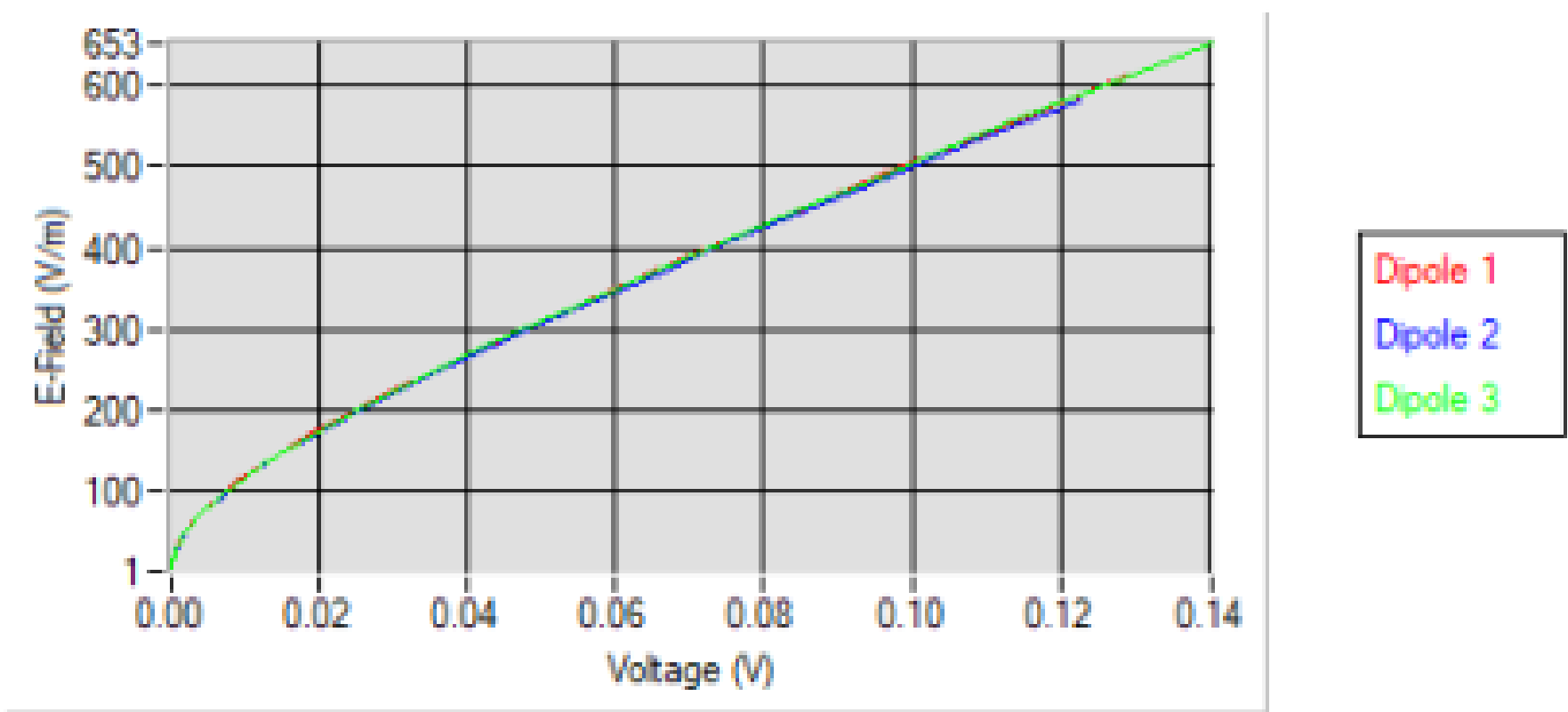
Calibration curves
