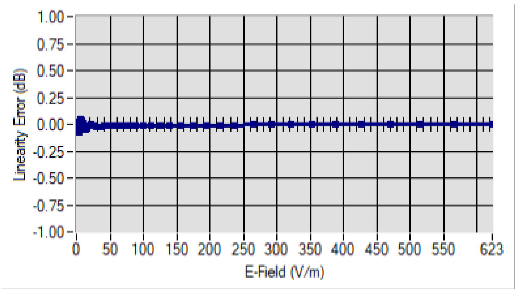
Linearity
