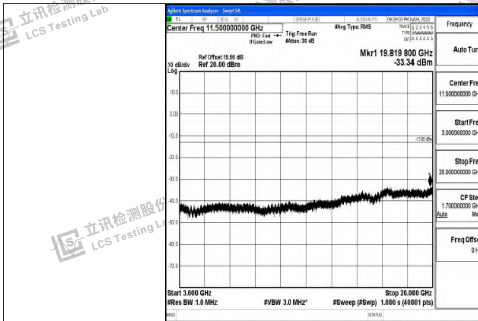
Band2_1.4MHz_16QAM_18900_1RB#0_3000~20000_3000~20000
