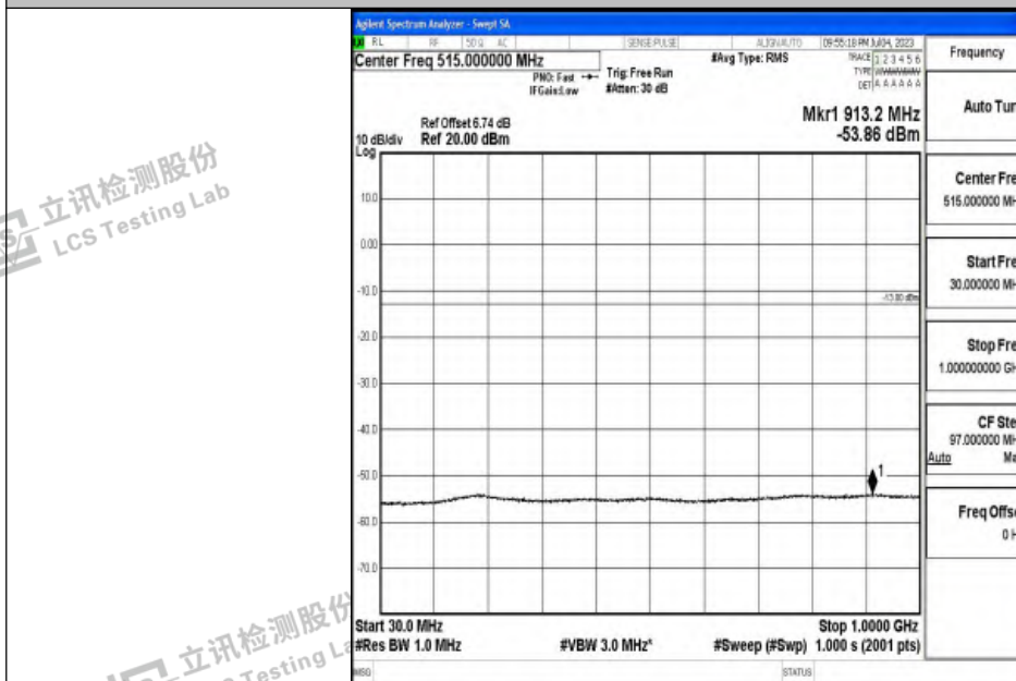
Band2_5MHz_QPSK_18625_1RB#0_30~1000_30~1000
