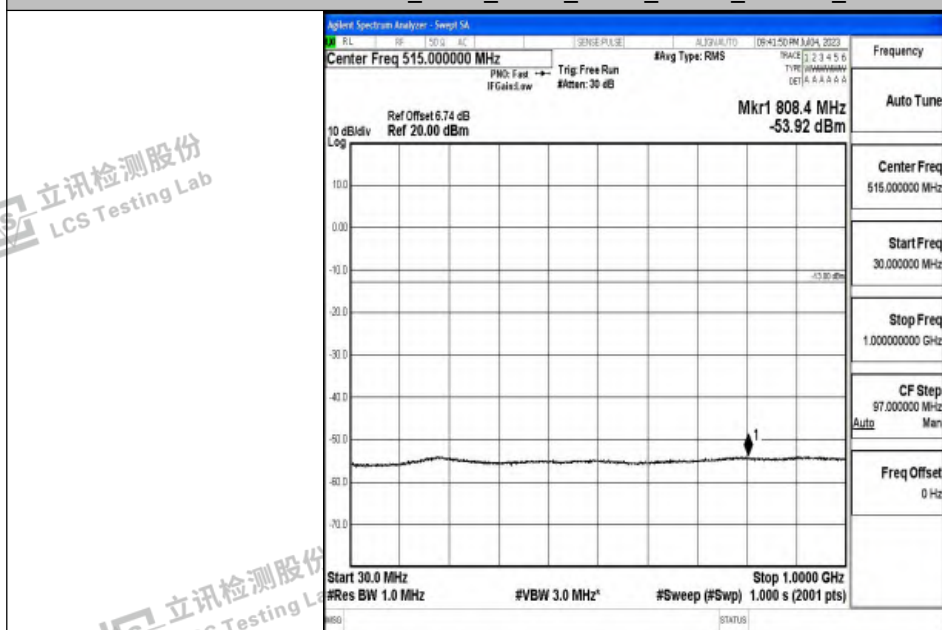
Band2_3MHz_QPSK_18900_1RB#0_30~1000_30~1000
