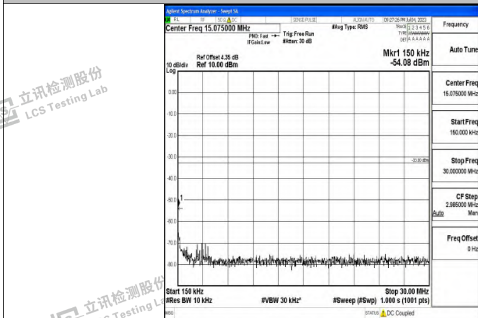
Band2_1.4MHz_16QAM_18607_1RB#0_0.15~30_0.15~30
