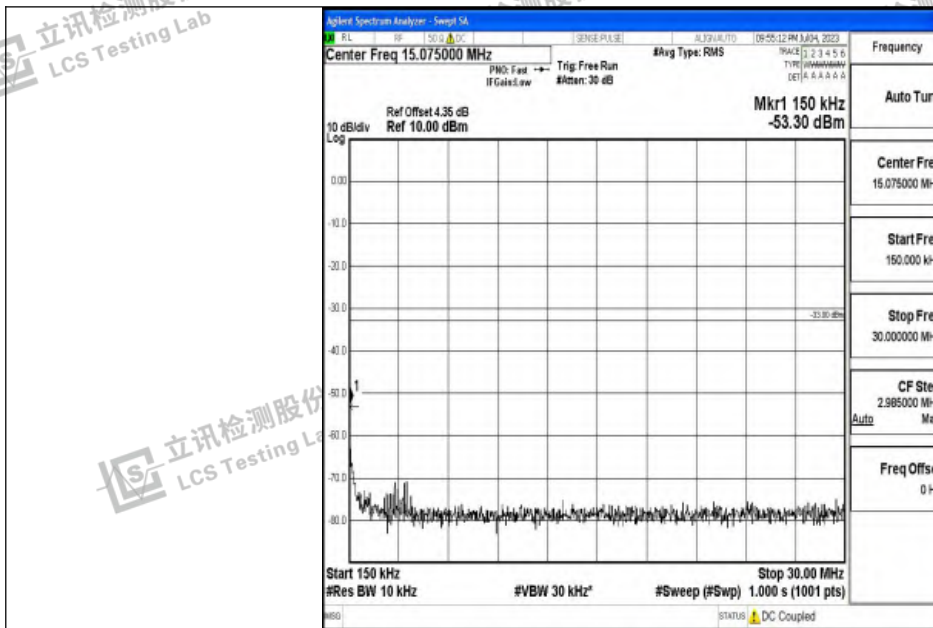
Band2_5MHz_QPSK_18625_1RB#0_0.15~30_0.15~30
