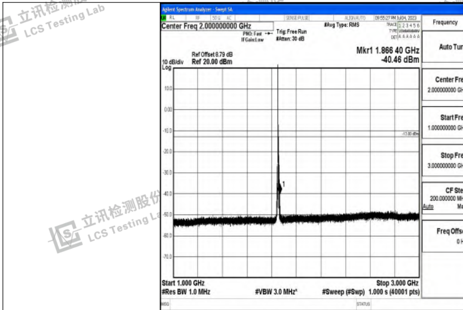
Band2_5MHz_QPSK_18625_1RB#0_1000~3000_1000~3000
