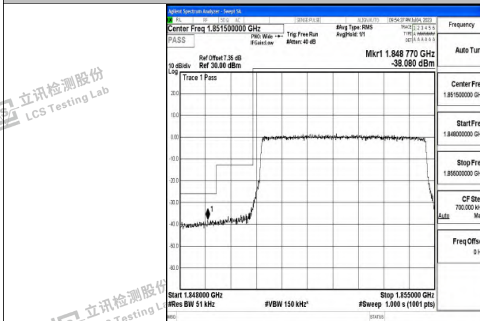
Band2_5MHz_16QAM_18625_25RB#0
