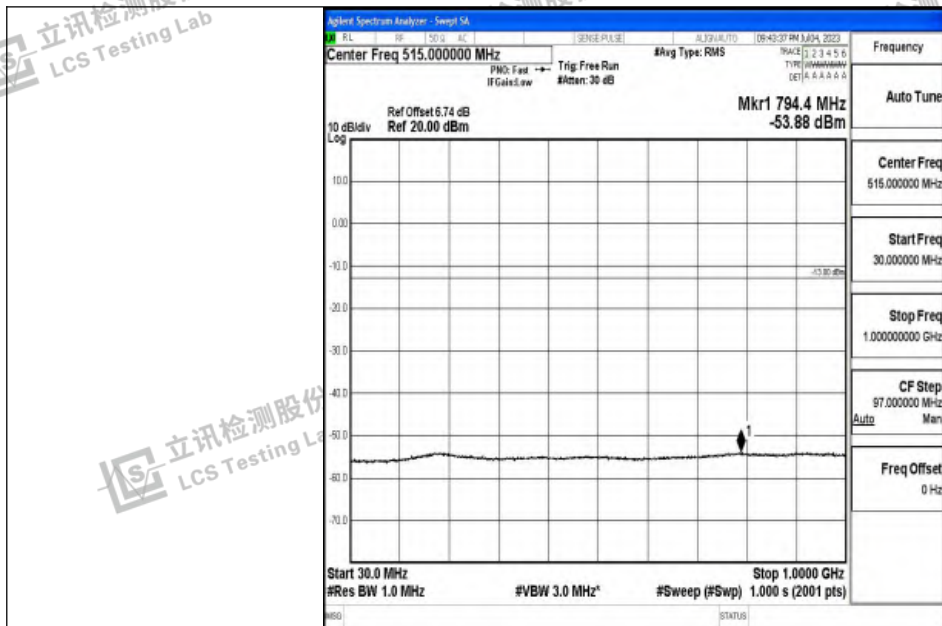
Band2_3MHz_16QAM_19185_1RB#0_30~1000_30~1000
