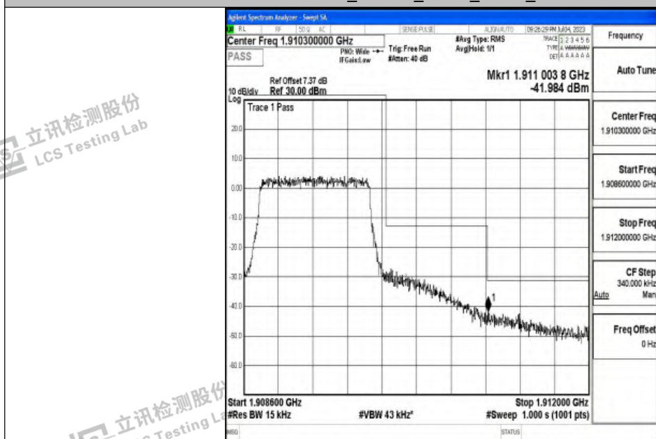
Band2_1.4MHz_16QAM_19193_6RB#0
