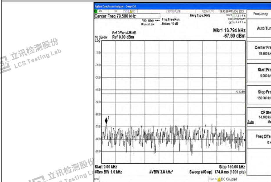
Band2_3MHz_QPSK_18615_1RB#0_0.009~0.15_0.009~0.15
