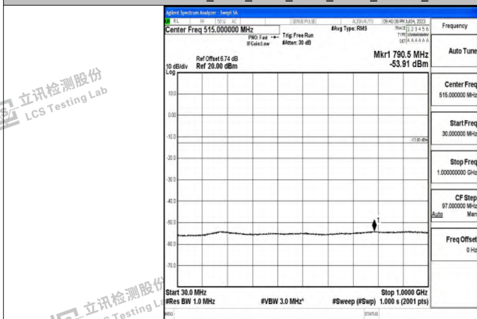
Band2_3MHz_QPSK_18615_1RB#0_30~1000_30~1000
