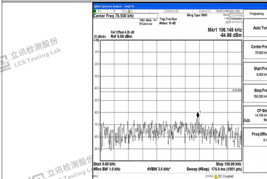
Band2_1.4MHz_QPSK_19193_1RB#0_0.009~0.15_0.009~0.15
