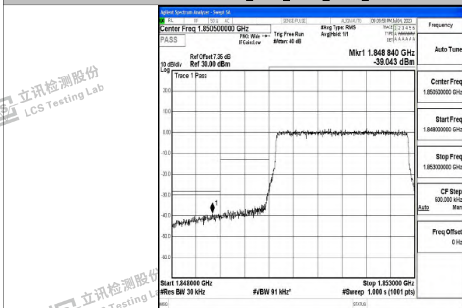
Band2_3MHz_16QAM_18615_15RB#0
