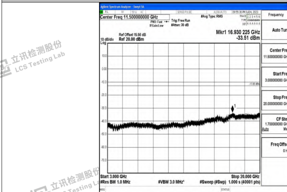
Band2_5MHz_QPSK_18625_1RB#0_3000~20000_3000~20000
