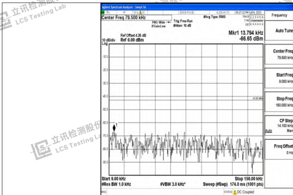
Band2_1.4MHz_16QAM_18607_1RB#0_0.009~0.15_0.009~0.15
