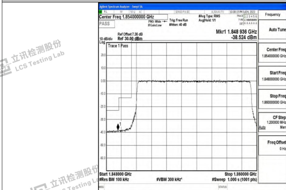
Band2_10MHz_16QAM_18650_50RB#0
