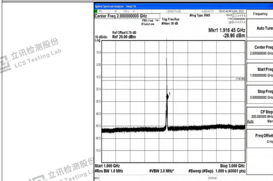
Band2_3MHz_16QAM_19185_1RB#0_1000~3000_1000~3000
