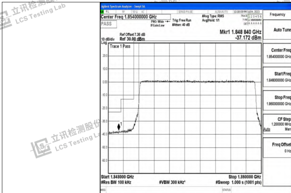
Band2_10MHz_QPSK_18650_50RB#0
