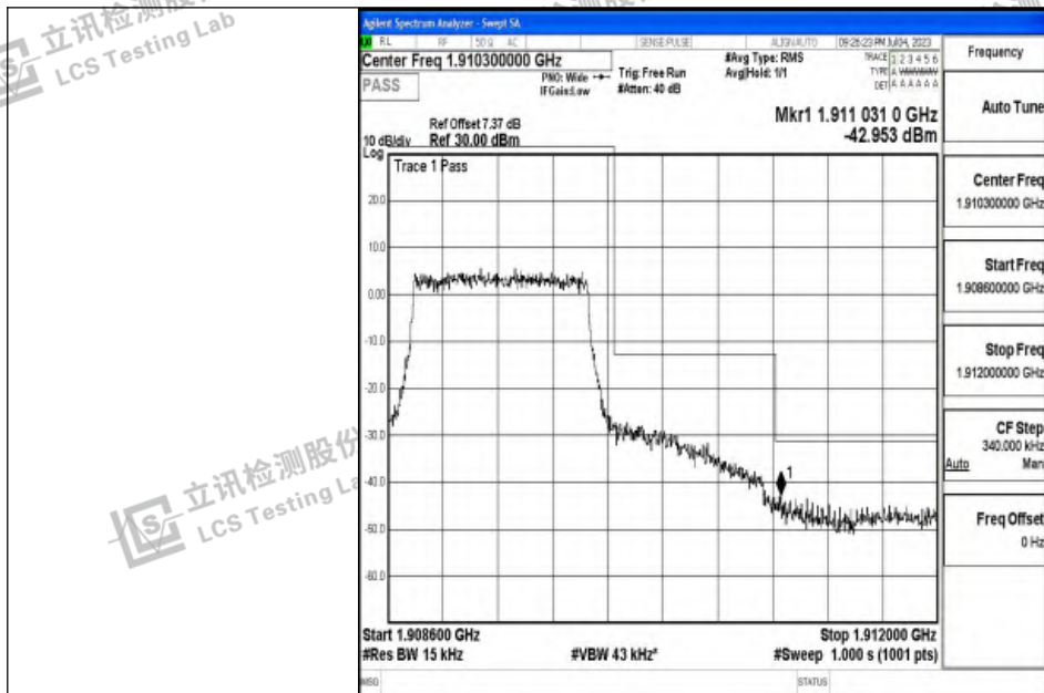
Band2_1.4MHz_QPSK_19193_6RB#0
