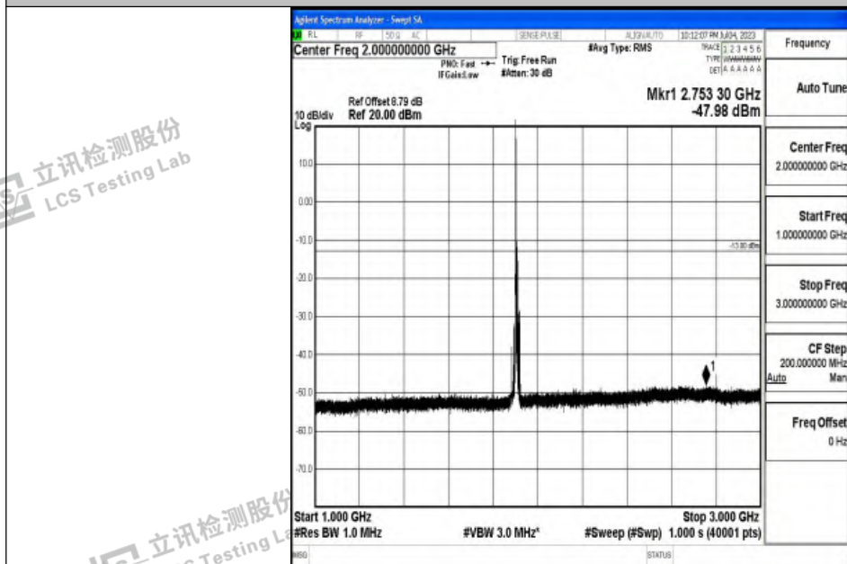
Band2_10MHz_16QAM_19150_1RB#0_1000~3000_1000~3000
