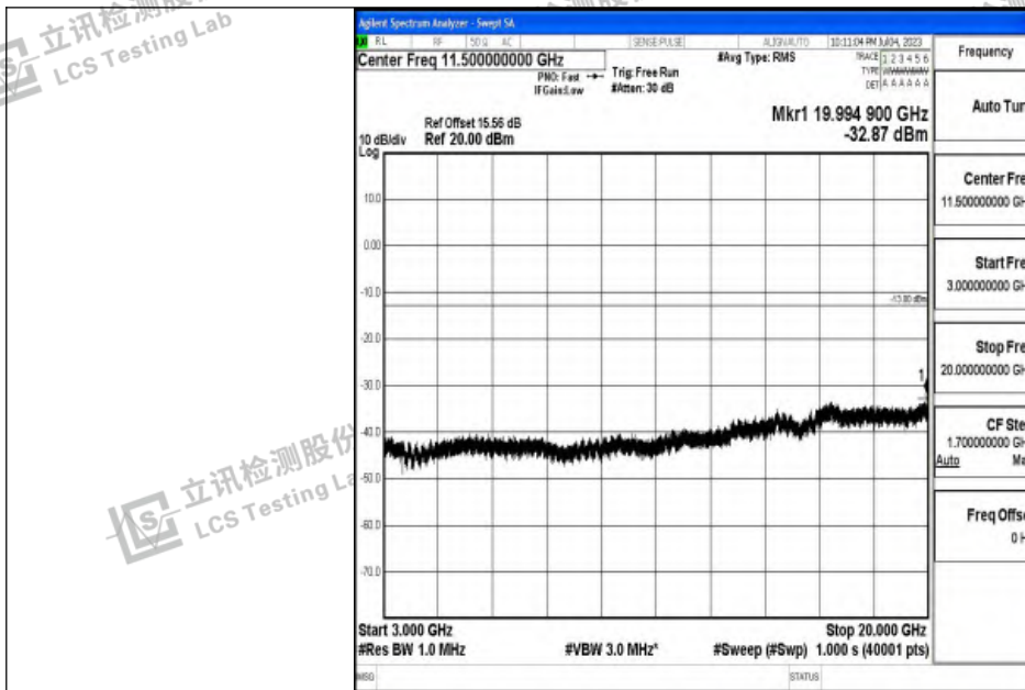
Band2_10MHz_16QAM_18900_1RB#0_3000~20000_3000~20000
