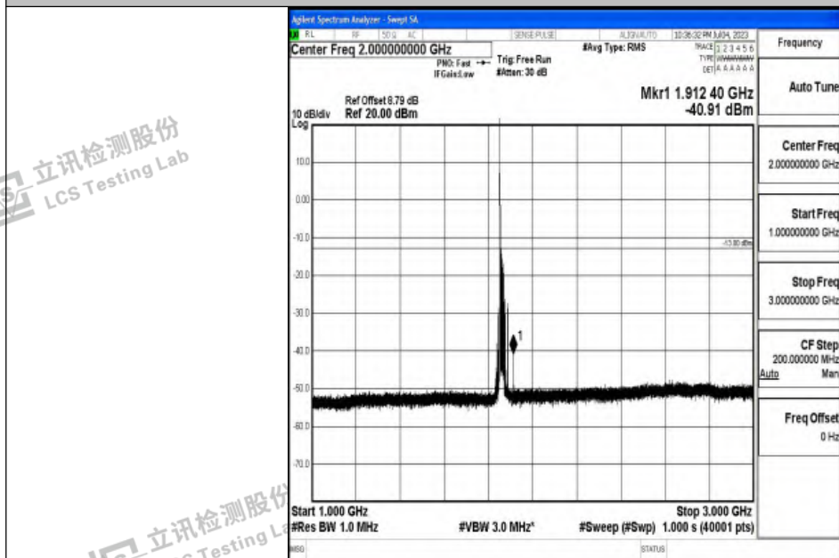
Band2_20MHz_16QAM_18700_1RB#0_1000~3000_1000~3000
