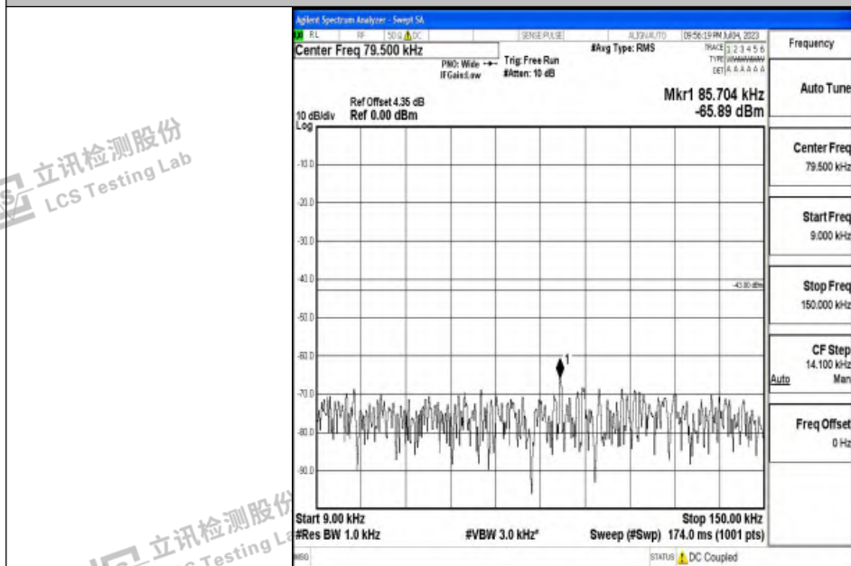
Band2_5MHz_QPSK_18900_1RB#0_0.009~0.15_0.009~0.15
