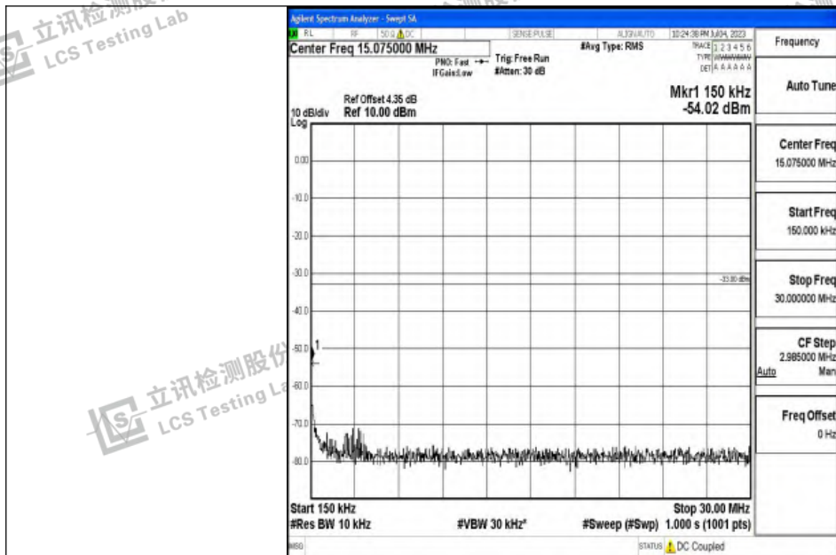
Band2_15MHz_QPSK_19125_1RB#0_0.15~30_0.15~30
