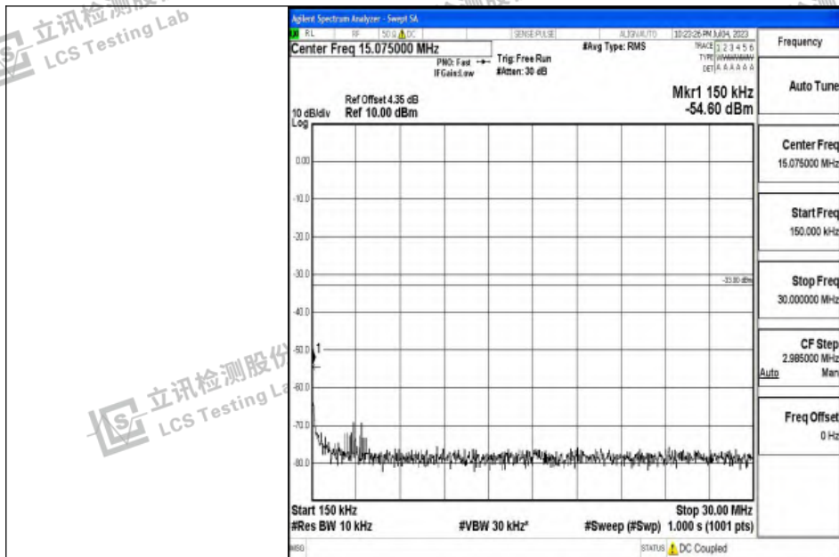
Band2_15MHz_QPSK_18900_1RB#0_0.15~30_0.15~30
