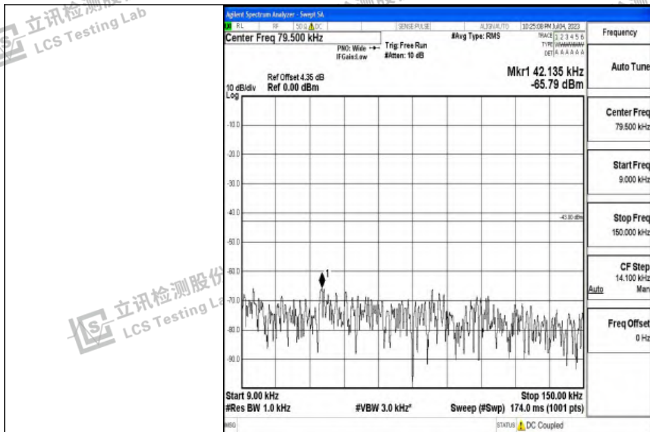
Band2_15MHz_16QAM_19125_1RB#0_0.009~0.15_0.009~0.15
