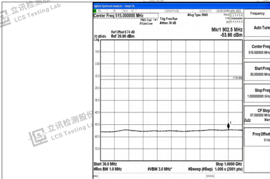
Band2_15MHz_16QAM_19125_1RB#0_30~1000_30~1000
