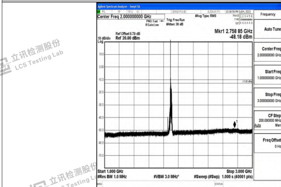
Band2_20MHz_16QAM_19100_1RB#0_1000~3000_1000~3000
