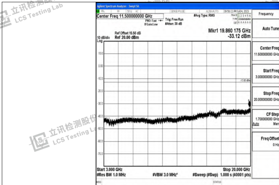
Band2_5MHz_16QAM_18625_1RB#0_3000~20000_3000~20000
