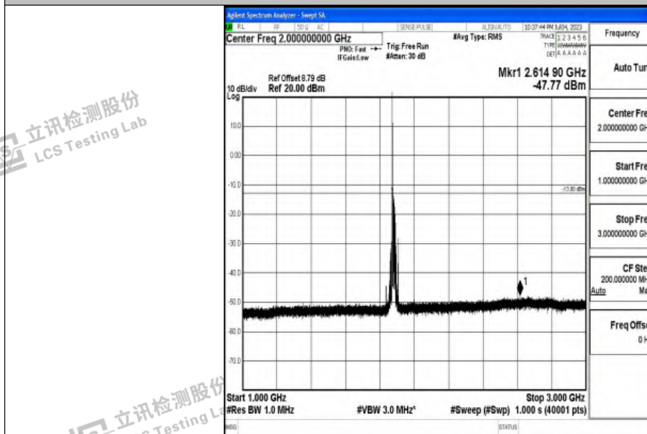
Band2_20MHz_16QAM_18900_1RB#0_1000~3000_1000~3000
