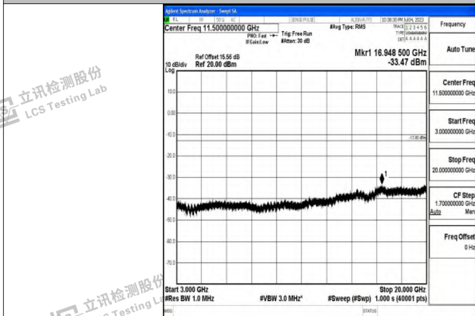
Band2_20MHz_QPSK_19100_1RB#0_3000~20000_3000~20000
