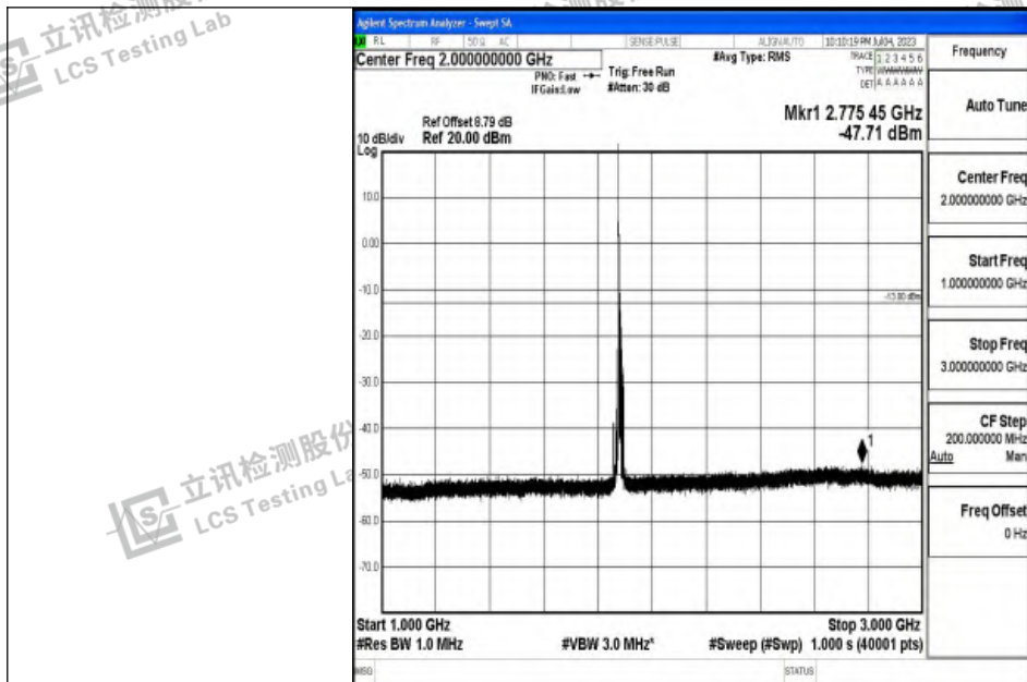
Band2_10MHz_QPSK_18900_1RB#0_1000~3000_1000~3000
