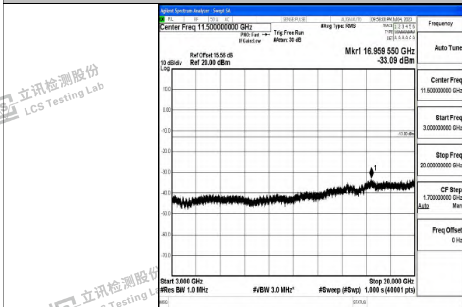
Band2_5MHz_QPSK_19175_1RB#0_3000~20000_3000~20000
