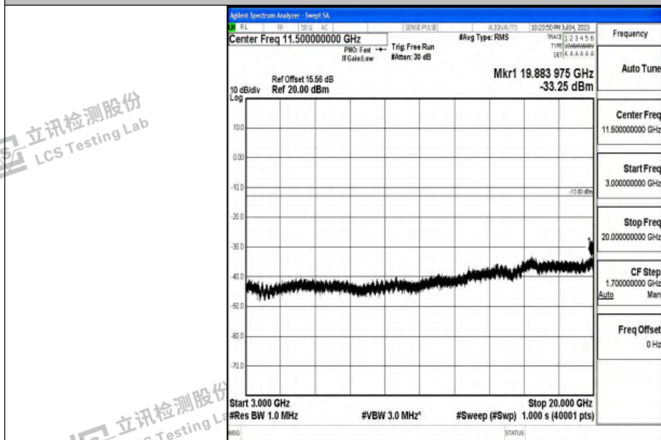
Band2_15MHz_QPSK_18900_1RB#0_3000~20000_3000~20000
