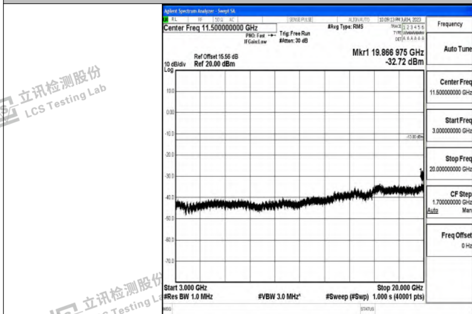
Band2_10MHz_QPSK_18650_1RB#0_3000~20000_3000~20000
