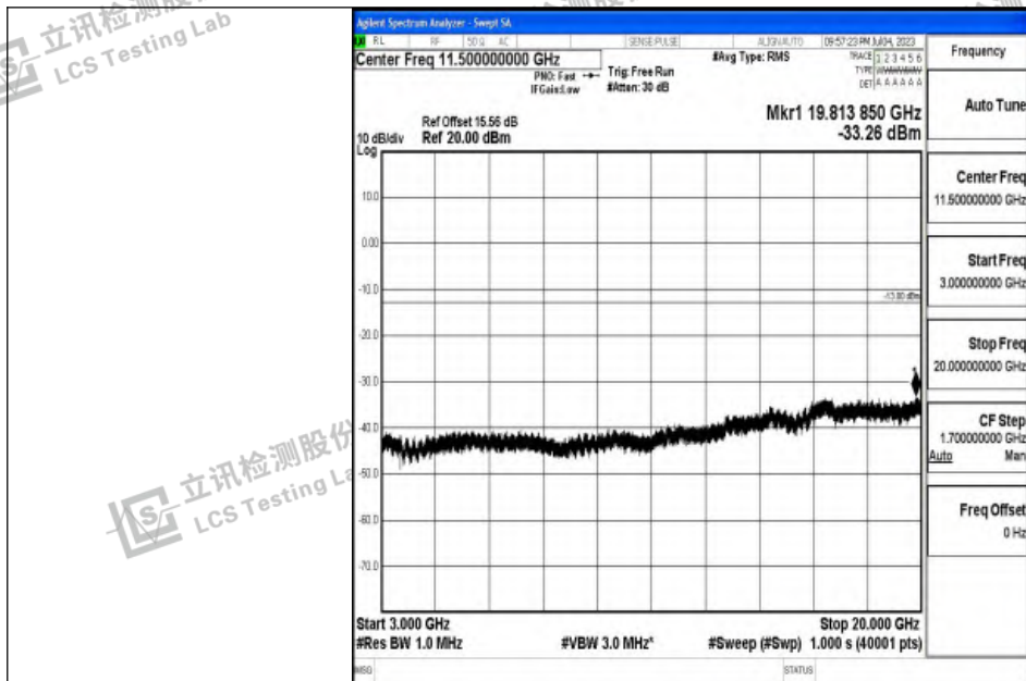
Band2_5MHz_16QAM_18900_1RB#0_3000~20000_3000~20000
