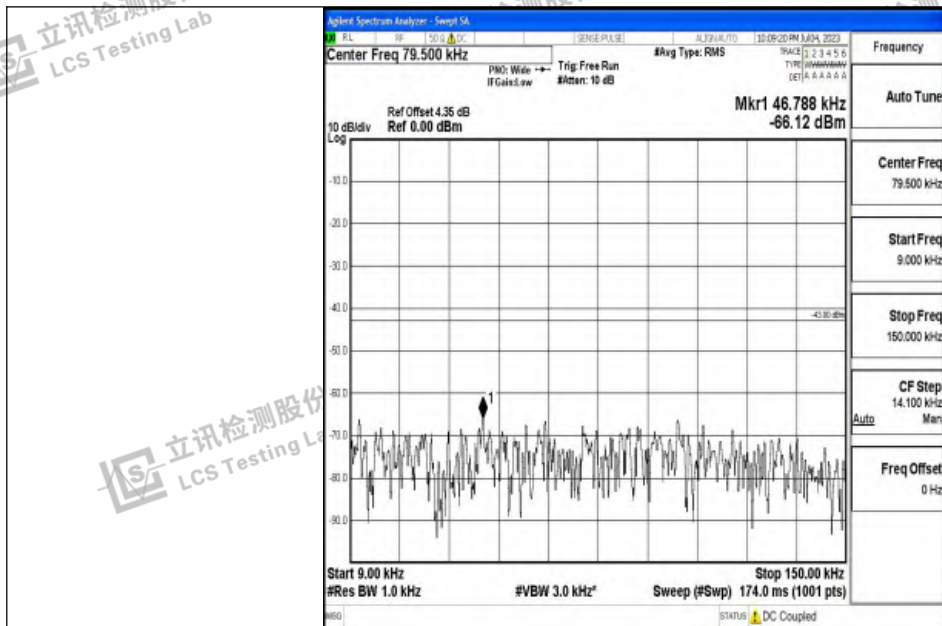
Band2_10MHz_16QAM_18650_1RB#0_0.009~0.15_0.009~0.15
