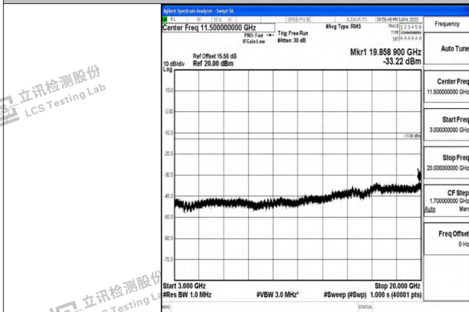
Band2_5MHz_QPSK_18900_1RB#0_3000~20000_3000~20000
