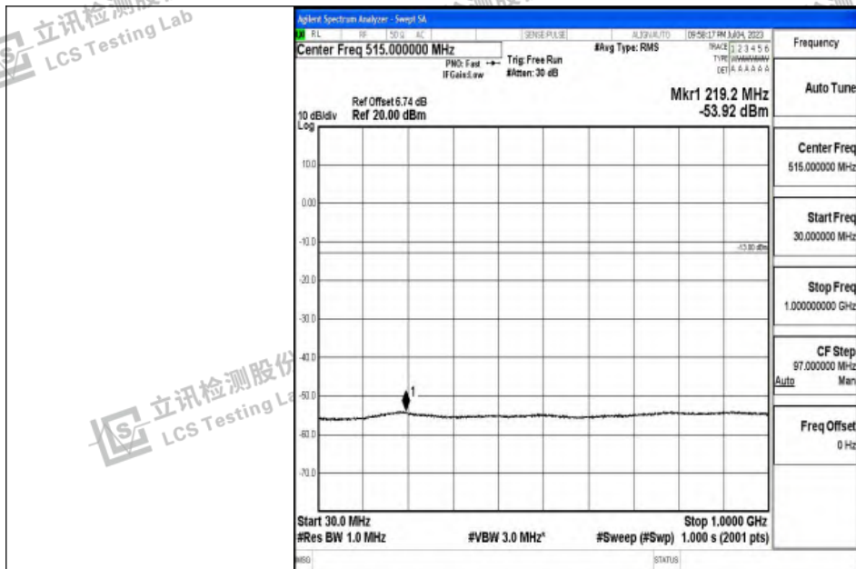
Band2_5MHz_16QAM_19175_1RB#0_30~1000_30~1000
