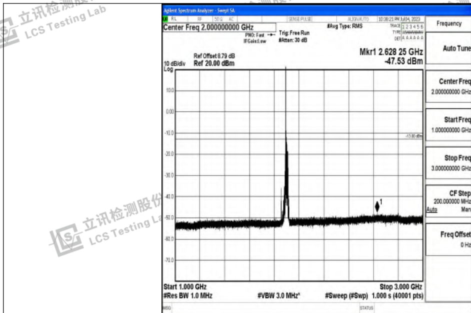
Band2_20MHz_QPSK_19100_1RB#0_1000~3000_1000~3000
