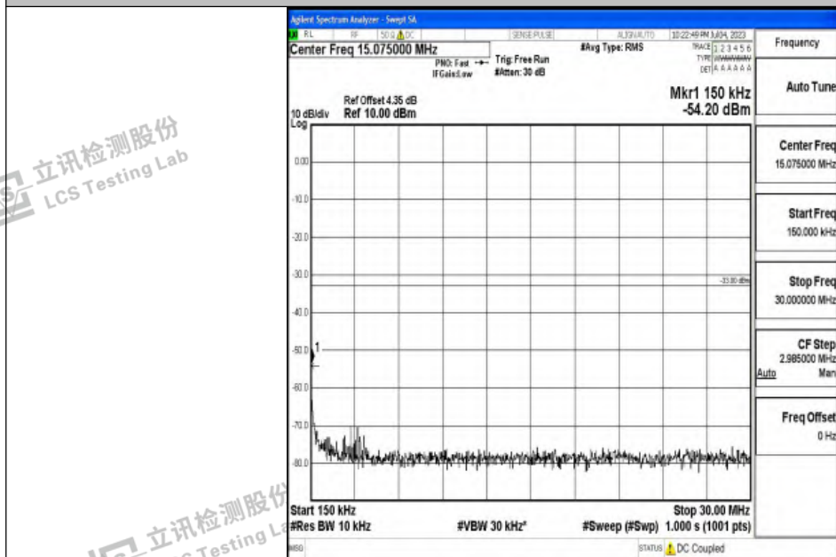
Band2_15MHz_16QAM_18675_1RB#0_0.15~30_0.15~30
