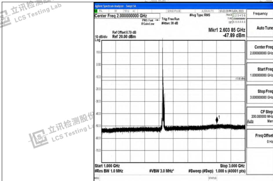
Band2_15MHz_QPSK_18675_1RB#0_1000~3000_1000~3000
