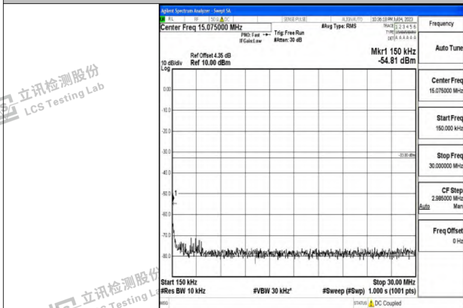
Band2_20MHz_16QAM_18700_1RB#0_0.15~30_0.15~30
