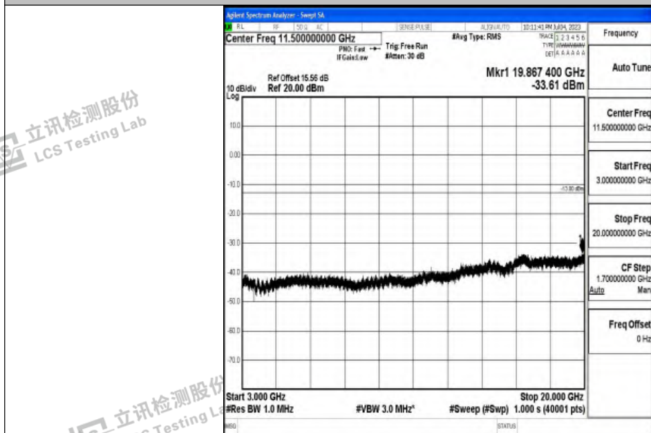
Band2_10MHz_QPSK_19150_1RB#0_3000~20000_3000~20000
