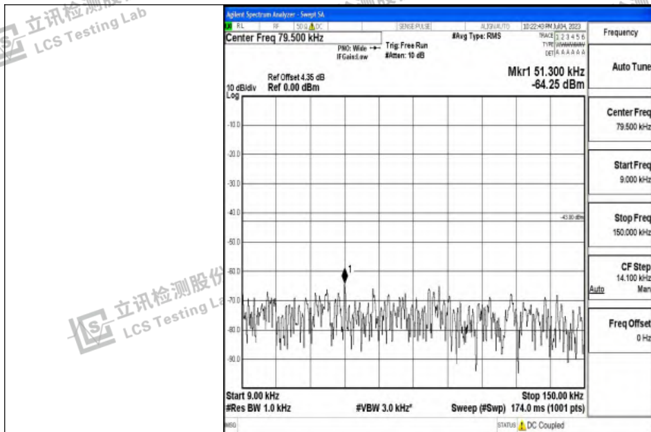
Band2_15MHz_16QAM_18675_1RB#0_0.009~0.15_0.009~0.15
