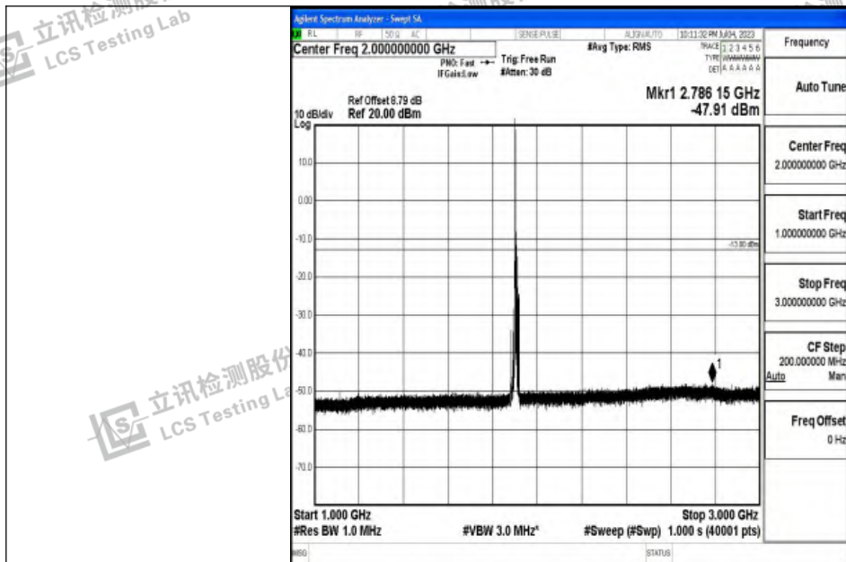
Band2_10MHz_QPSK_19150_1RB#0_1000~3000_1000~3000
