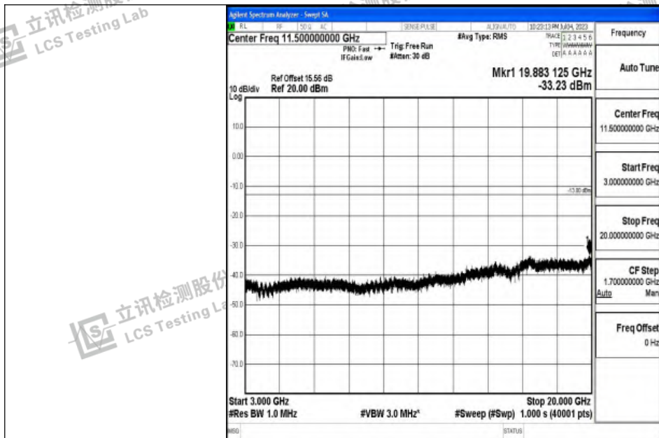
Band2_15MHz_16QAM_18675_1RB#0_3000~20000_3000~20000
