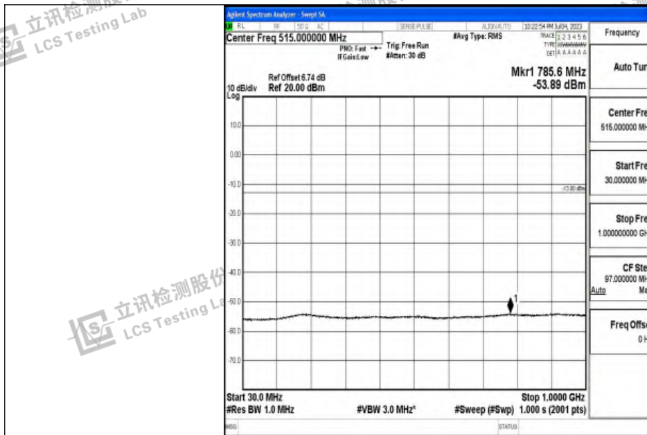
Band2_15MHz_16QAM_18675_1RB#0_30~1000_30~1000
