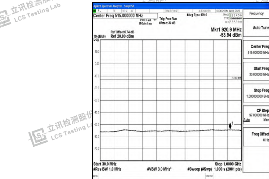
Band2_20MHz_16QAM_18700_1RB#0_30~1000_30~1000
