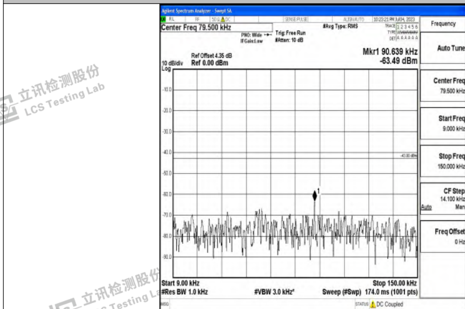
Band2_15MHz_QPSK_18900_1RB#0_0.009~0.15_0.009~0.15
