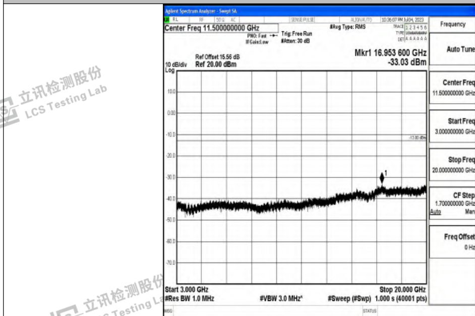
Band2_20MHz_QPSK_18700_1RB#0_3000~20000_3000~20000
