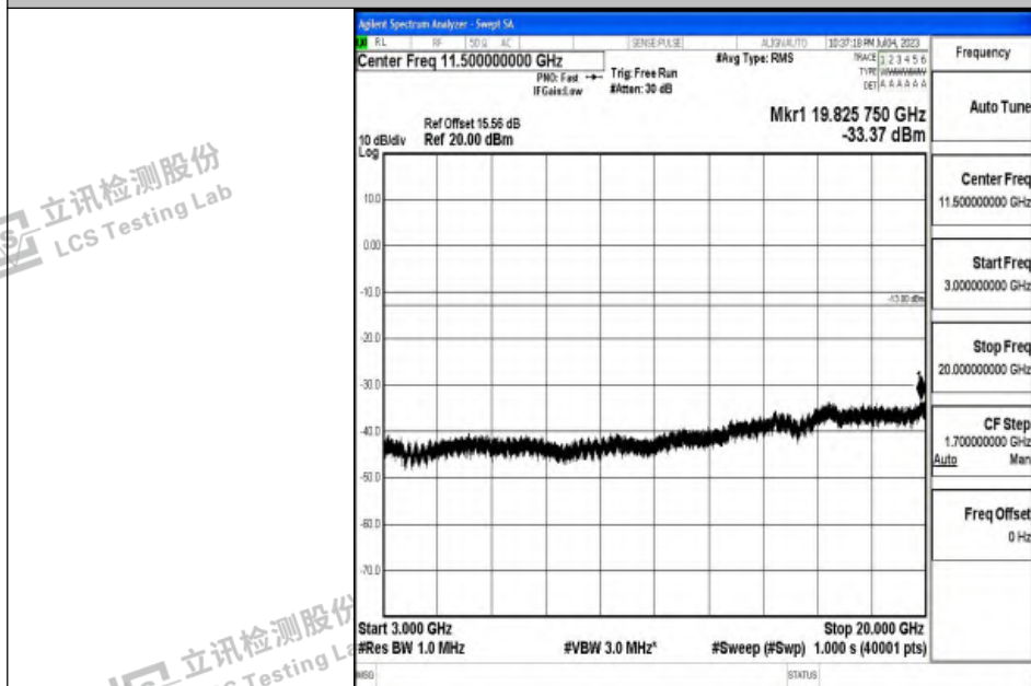
Band2_20MHz_QPSK_18900_1RB#0_3000~20000_3000~20000
