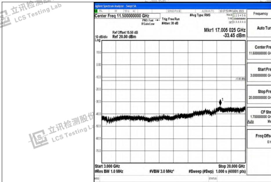
Band2_20MHz_16QAM_18900_1RB#0_3000~20000_3000~20000
