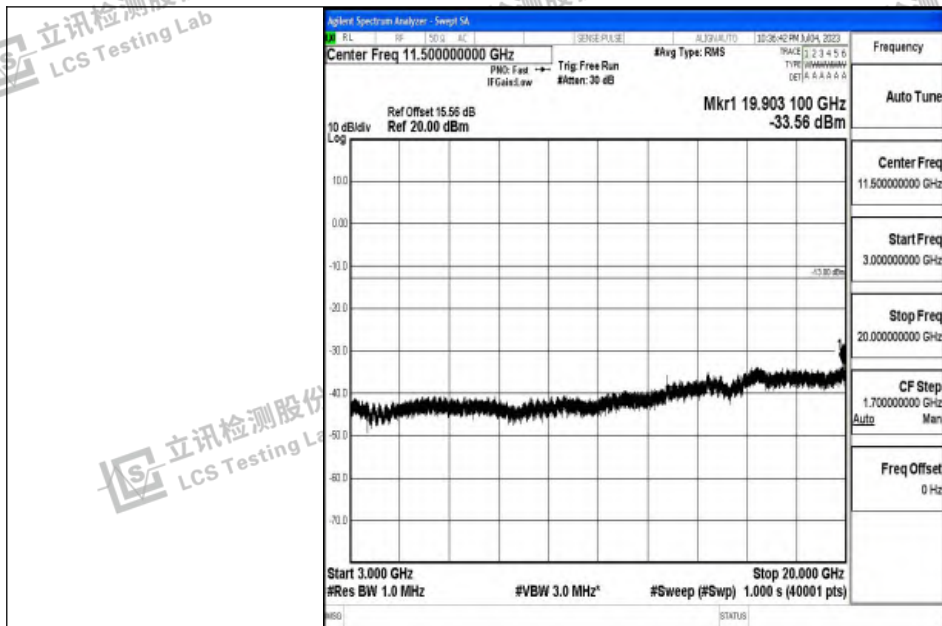
Band2_20MHz_16QAM_18700_1RB#0_3000~20000_3000~20000
