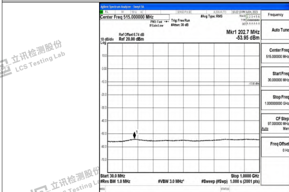
Band2_15MHz_QPSK_18675_1RB#0_30~1000_30~1000
