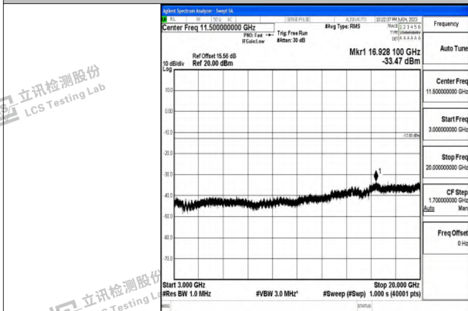
Band2_15MHz_QPSK_18675_1RB#0_3000~20000_3000~20000
