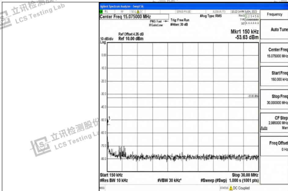
Band2_15MHz_QPSK_18675_1RB#0_0.15~30_0.15~30
