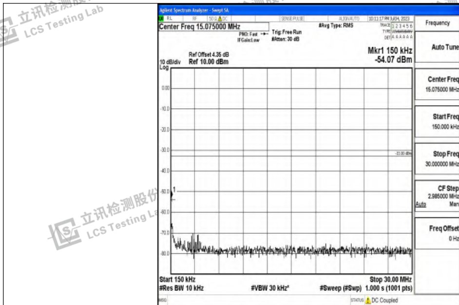
Band2_10MHz_QPSK_19150_1RB#0_0.15~30_0.15~30
