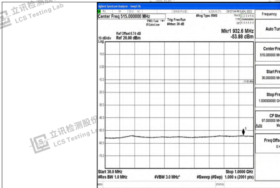
Band2_5MHz_16QAM_18900_1RB#0_30~1000_30~1000
