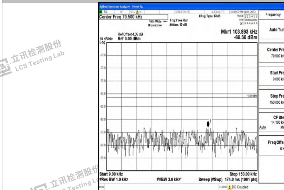
Band2_20MHz_QPSK_19100_1RB#0_0.009~0.15_0.009~0.15
