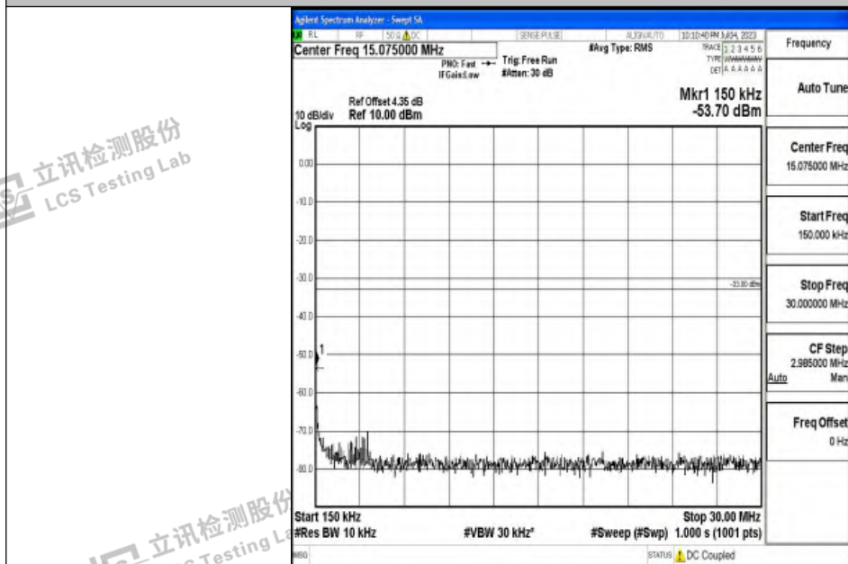
Band2_10MHz_16QAM_18900_1RB#0_0.15~30_0.15~30
