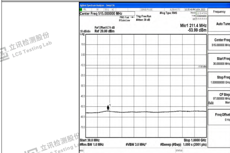
Band2_20MHz_QPSK_18700_1RB#0_30~1000_30~1000
