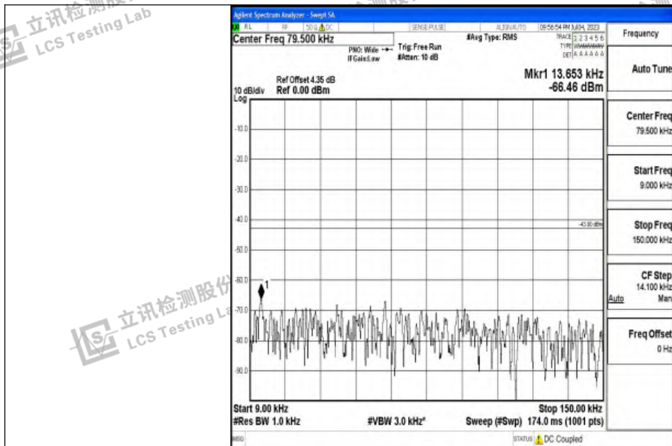
Band2_5MHz_16QAM_18900_1RB#0_0.009~0.15_0.009~0.15
