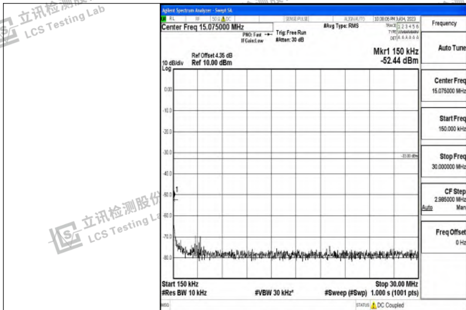
Band2_20MHz_QPSK_19100_1RB#0_0.15~30_0.15~30
