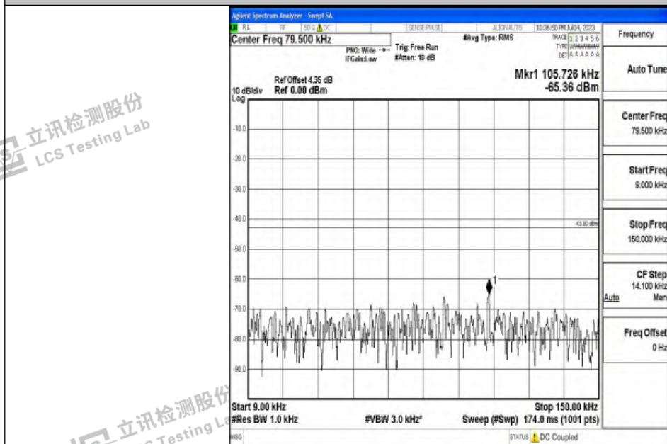
Band2_20MHz_QPSK_18900_1RB#0_0.009~0.15_0.009~0.15
