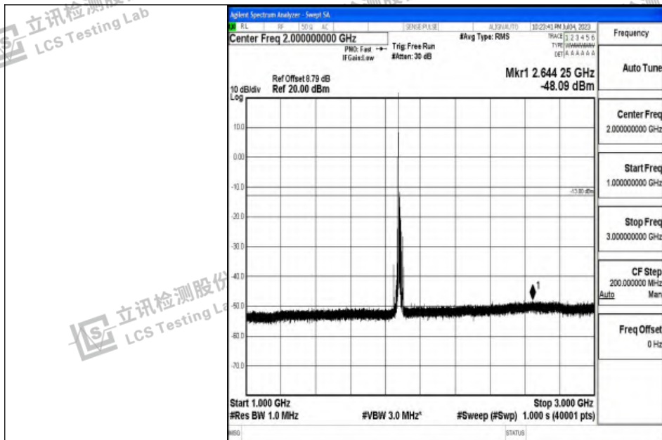
Band2_15MHz_QPSK_18900_1RB#0_1000~3000_1000~3000
