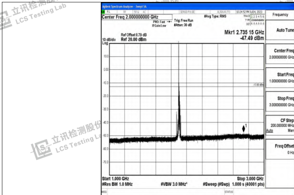
Band2_15MHz_QPSK_19125_1RB#0_1000~3000_1000~3000
