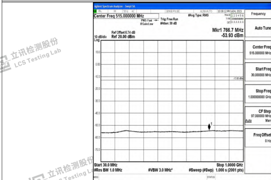
Band2_20MHz_QPSK_19100_1RB#0_30~1000_30~1000
