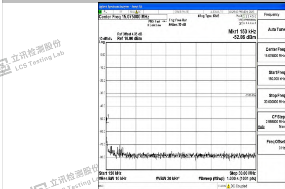
Band2_15MHz_16QAM_19125_1RB#0_0.15~30_0.15~30
