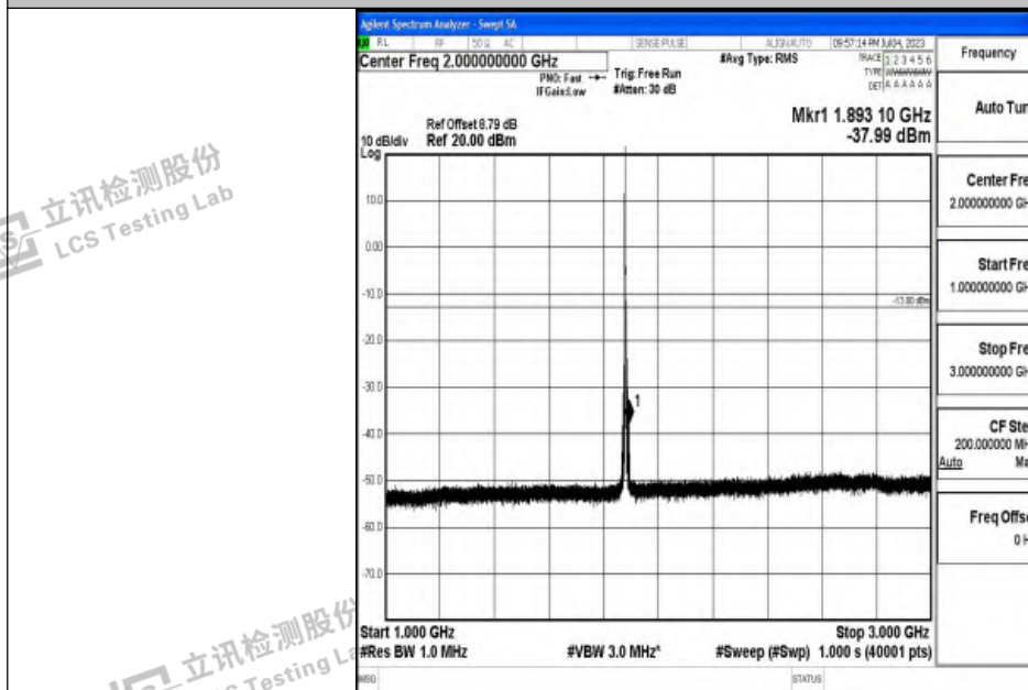
Band2_5MHz_16QAM_18900_1RB#0_1000~3000_1000~3000
