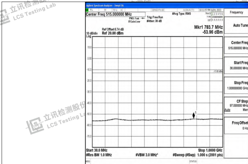
Band2_10MHz_16QAM_19150_1RB#0_30~1000_30~1000
