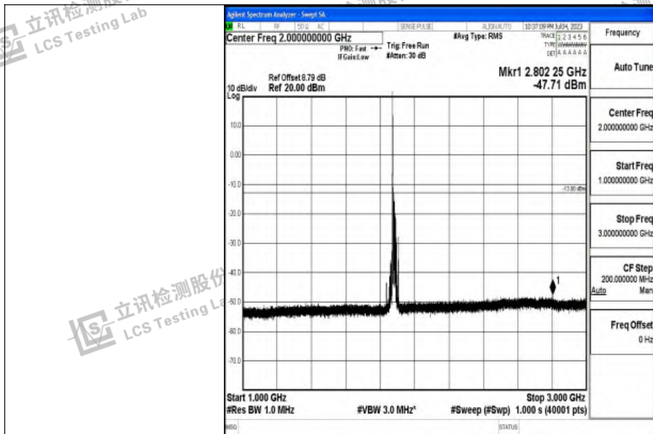
Band2_20MHz_QPSK_18900_1RB#0_1000~3000_1000~3000
