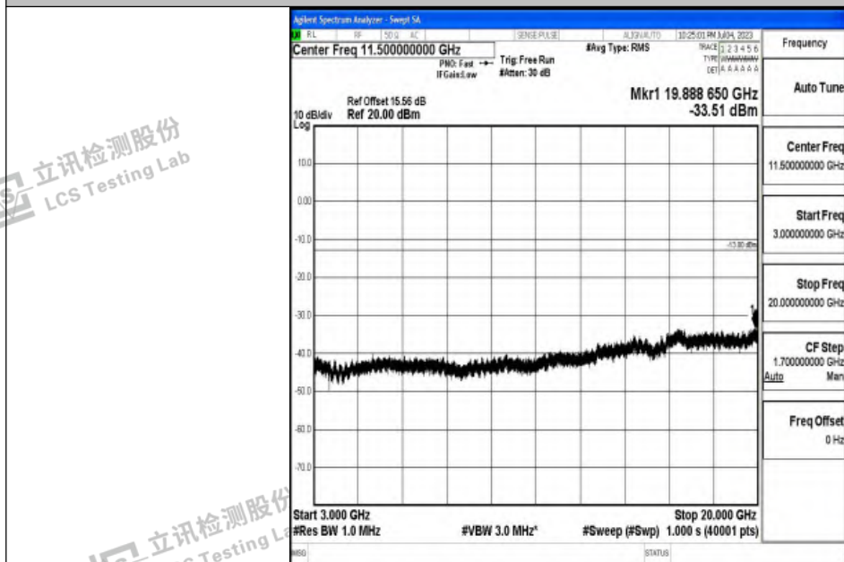
Band2_15MHz_QPSK_19125_1RB#0_3000~20000_3000~20000
