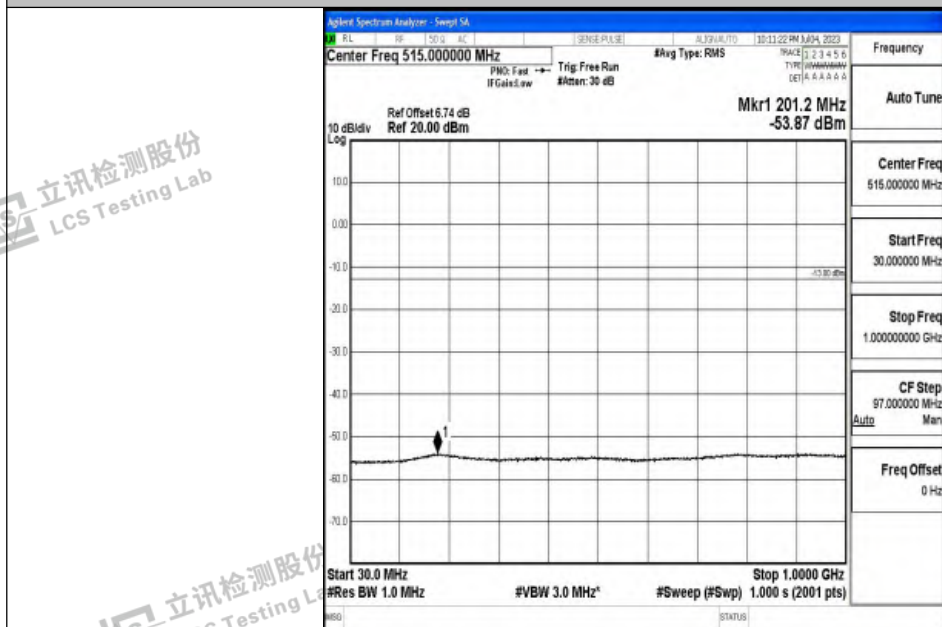
Band2_10MHz_QPSK_19150_1RB#0_30~1000_30~1000
