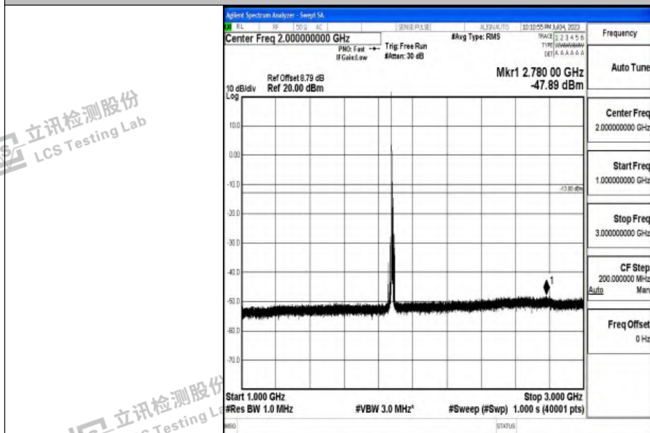
Band2_10MHz_16QAM_18900_1RB#0_1000~3000_1000~3000
