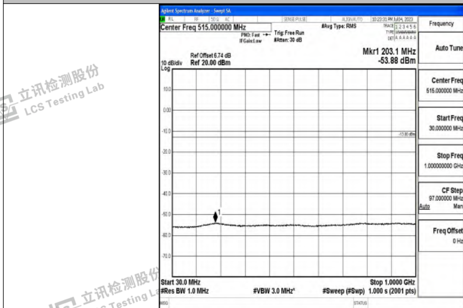
Band2_15MHz_QPSK_18900_1RB#0_30~1000_30~1000
