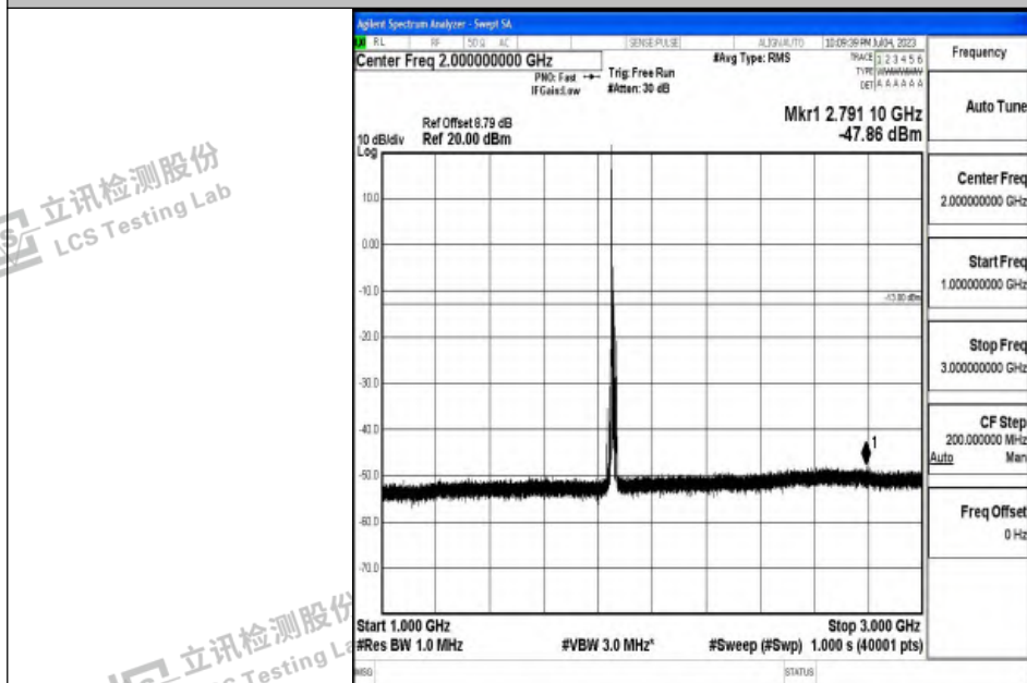
Band2_10MHz_16QAM_18650_1RB#0_1000~3000_1000~3000
