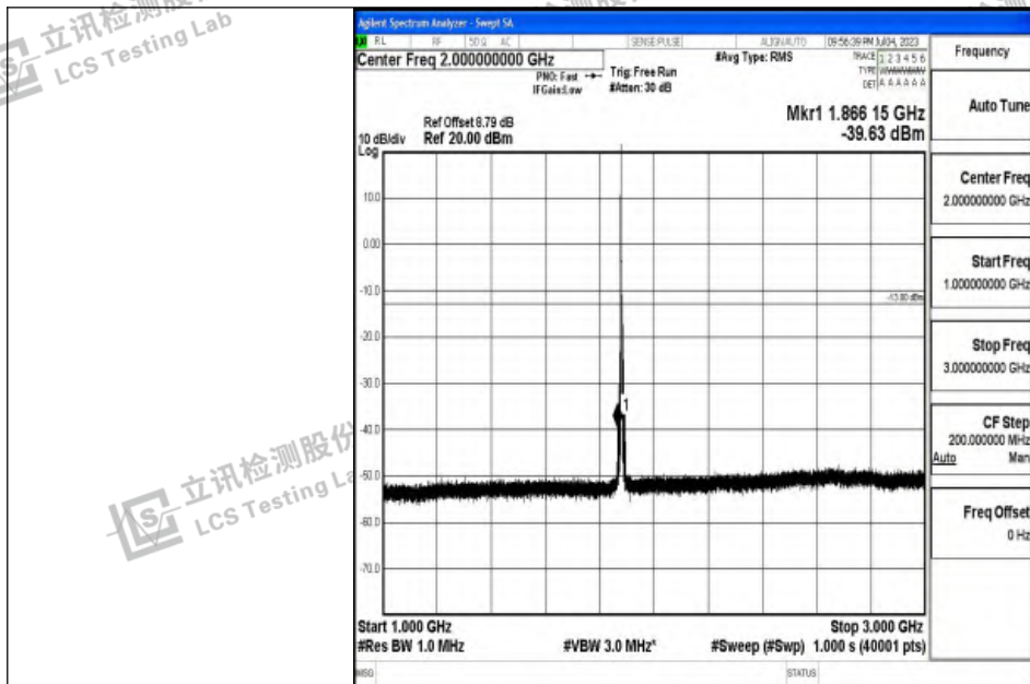
Band2_5MHz_QPSK_18900_1RB#0_1000~3000_1000~3000
