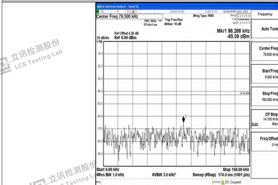
Band2_10MHz_QPSK_18650_1RB#0_0.009~0.15_0.009~0.15
