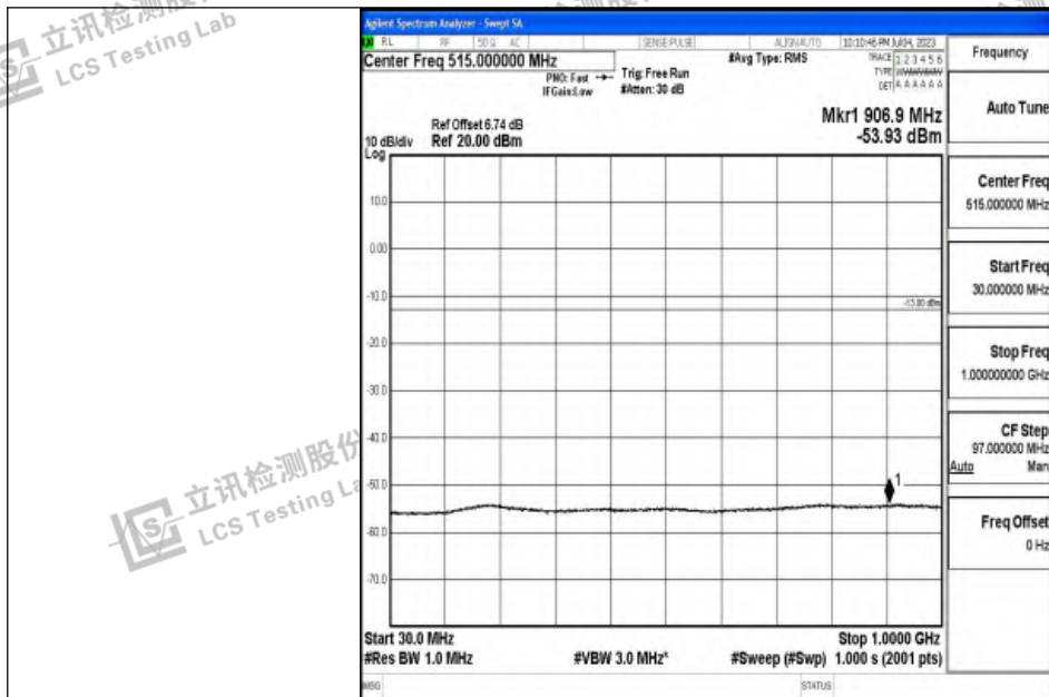
Band2_10MHz_16QAM_18900_1RB#0_30~1000_30~1000
