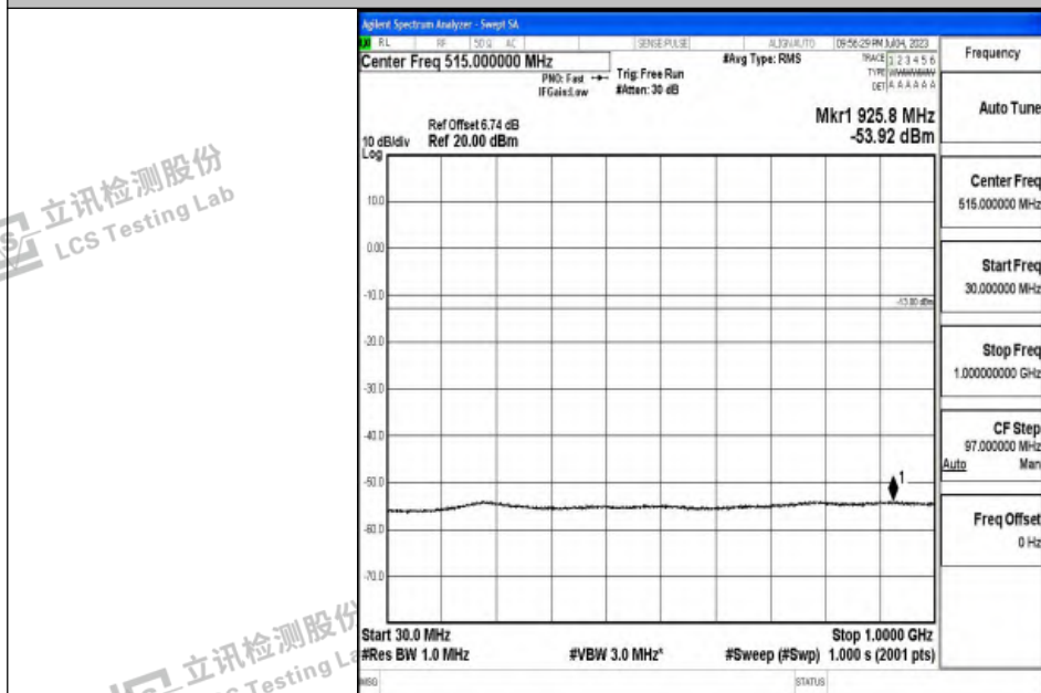
Band2_5MHz_QPSK_18900_1RB#0_30~1000_30~1000
