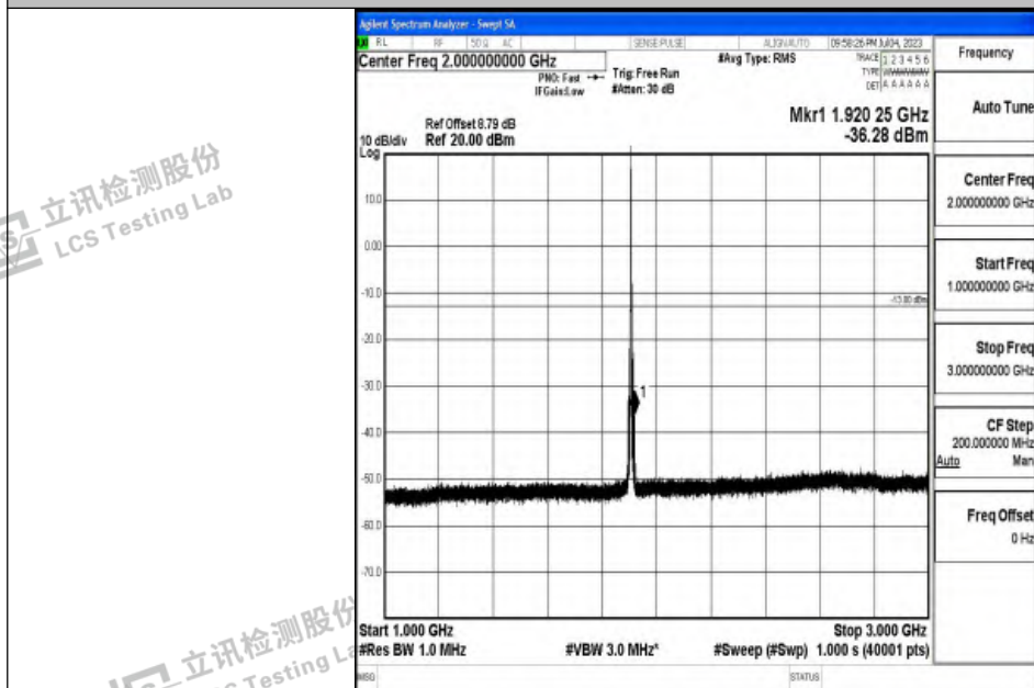
Band2_5MHz_16QAM_19175_1RB#0_1000~3000_1000~3000
