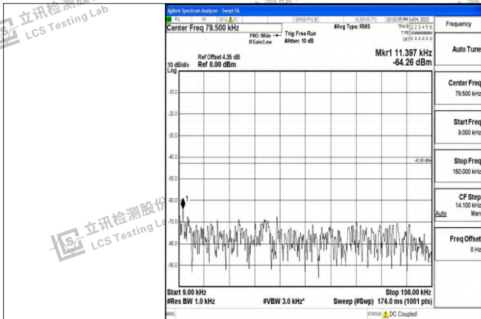
Band2_10MHz_16QAM_18900_1RB#0_0.009~0.15_0.009~0.15
