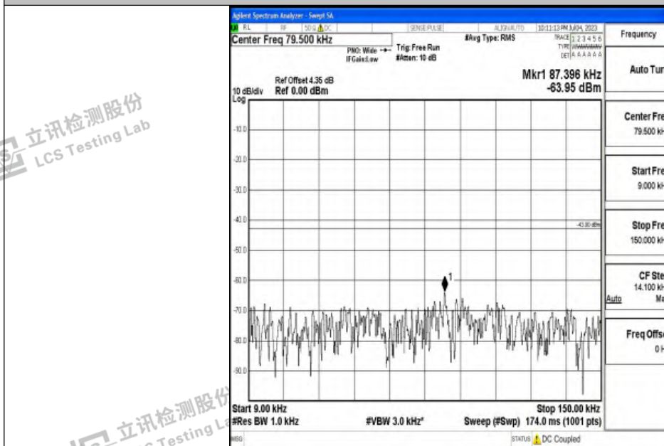
Band2_10MHz_QPSK_19150_1RB#0_0.009~0.15_0.009~0.15
