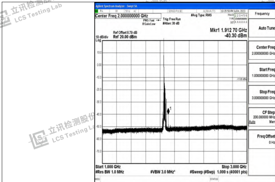
Band2_20MHz_QPSK_18700_1RB#0_1000~3000_1000~3000
