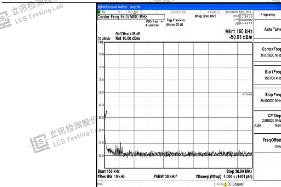
Band2_10MHz_QPSK_18900_1RB#0_0.15~30_0.15~30
