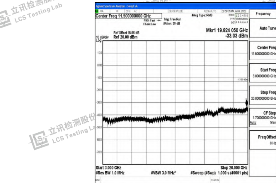
Band2_5MHz_16QAM_19175_1RB#0_3000~20000_3000~20000
