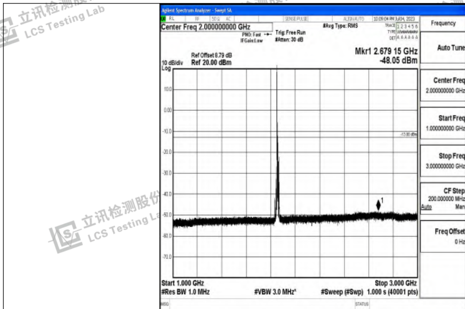
Band2_10MHz_QPSK_18650_1RB#0_1000~3000_1000~3000
