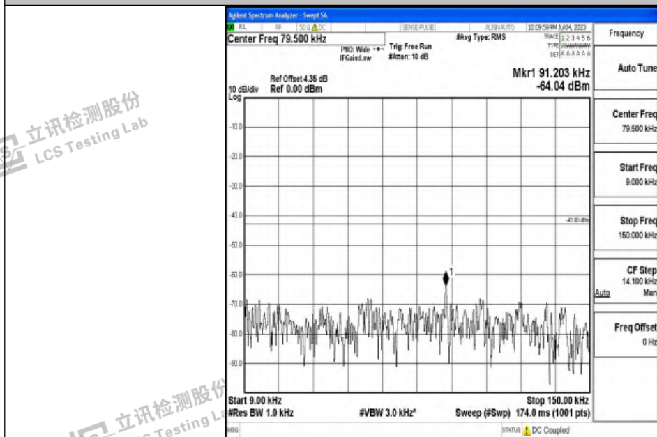
Band2_10MHz_QPSK_18900_1RB#0_0.009~0.15_0.009~0.15
