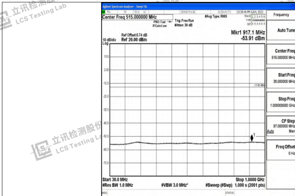
Band2_20MHz_16QAM_19100_1RB#0_30~1000_30~1000
