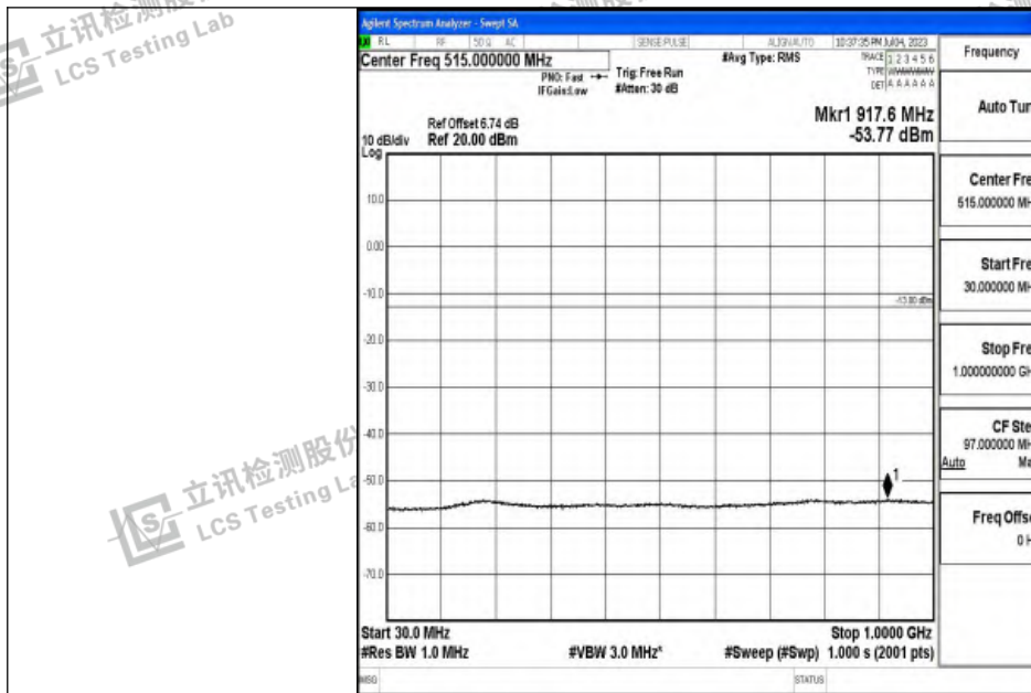
Band2_20MHz_16QAM_18900_1RB#0_30~1000_30~1000
