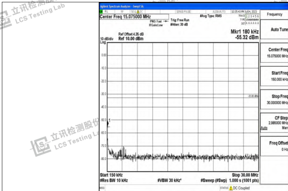
Band2_20MHz_QPSK_18700_1RB#0_0.15~30_0.15~30
