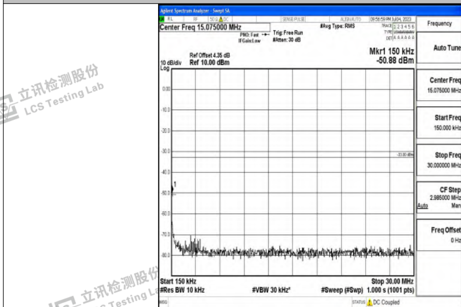
Band2_5MHz_16QAM_18900_1RB#0_0.15~30_0.15~30
