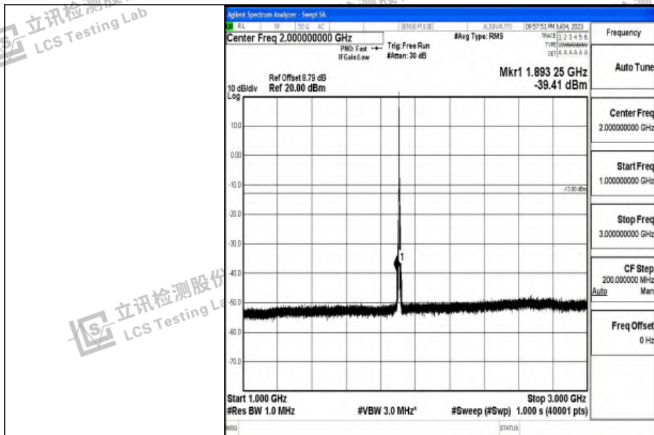
Band2_5MHz_QPSK_19175_1RB#0_1000~3000_1000~3000
