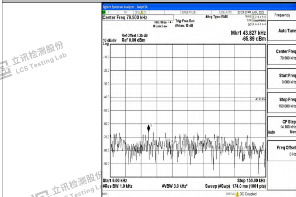
Band2_15MHz_QPSK_19125_1RB#0_0.009~0.15_0.009~0.15
