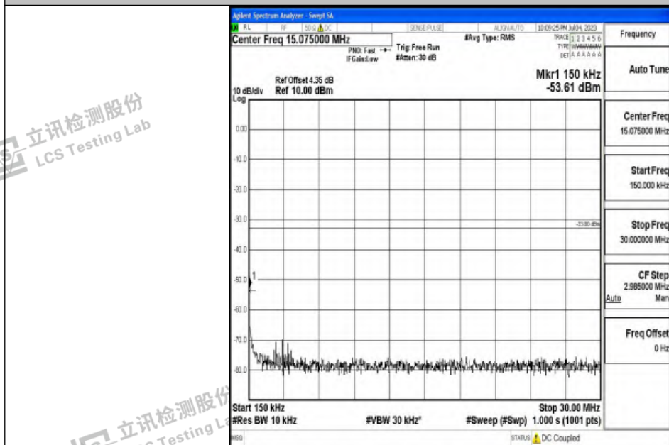
Band2_10MHz_16QAM_18650_1RB#0_0.15~30_0.15~30
