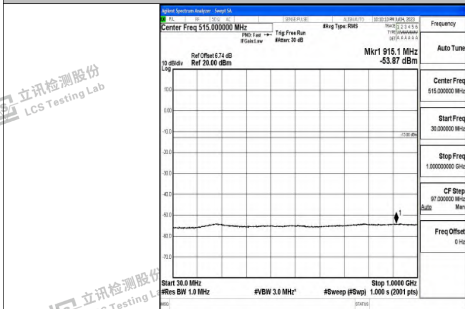
Band2_10MHz_QPSK_18900_1RB#0_30~1000_30~1000
