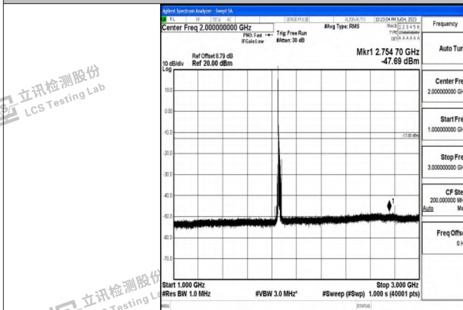
Band2_15MHz_16QAM_18675_1RB#0_1000~3000_1000~3000
