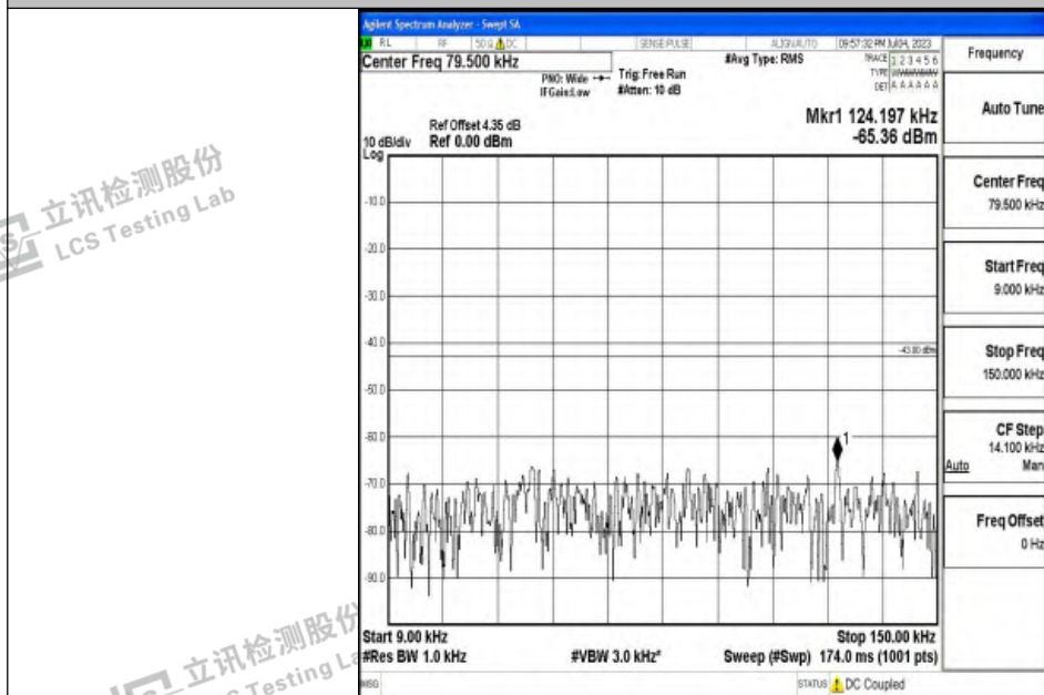
Band2_5MHz_QPSK_19175_1RB#0_0.009~0.15_0.009~0.15
