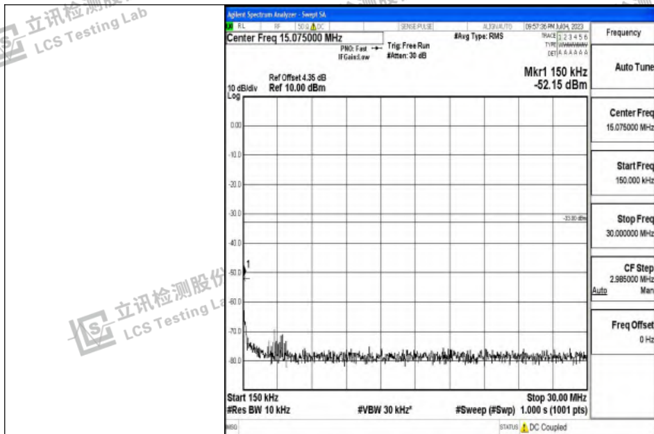
Band2_5MHz_QPSK_19175_1RB#0_0.15~30_0.15~30
