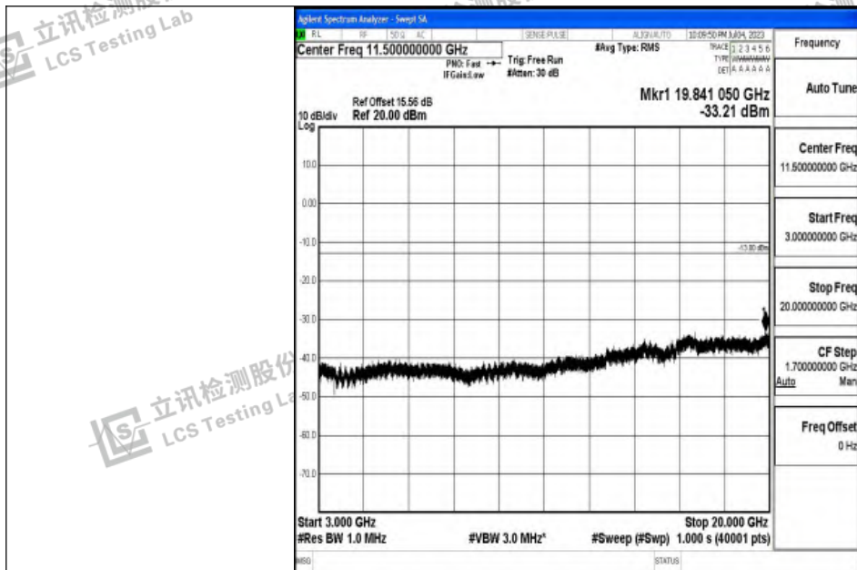
Band2_10MHz_16QAM_18650_1RB#0_3000~20000_3000~20000
