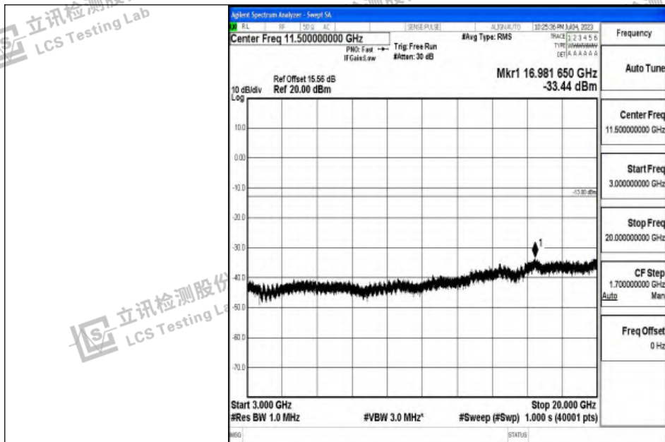
Band2_15MHz_16QAM_19125_1RB#0_3000~20000_3000~20000
