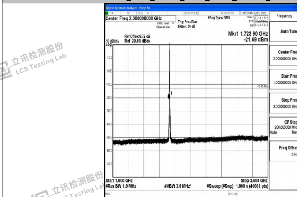
Band4_3MHz_16QAM_20175_1RB#0_1000~3000_1000~3000
