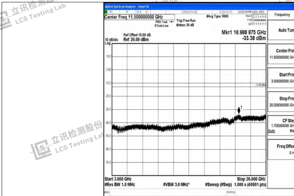
Band4_1.4MHz_16QAM_20393_1RB#0_3000~20000_3000~20000
