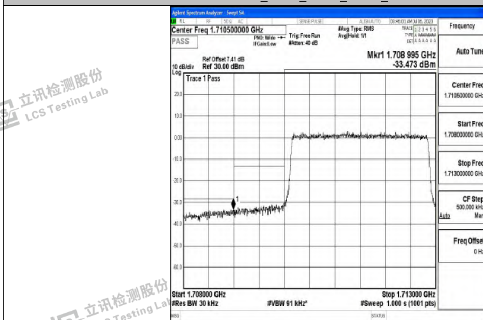
Band4_3MHz_16QAM_19965_15RB#0
