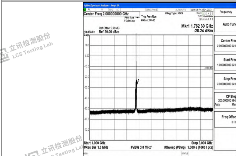
Band4_3MHz_16QAM_20385_1RB#0_1000~3000_1000~3000
