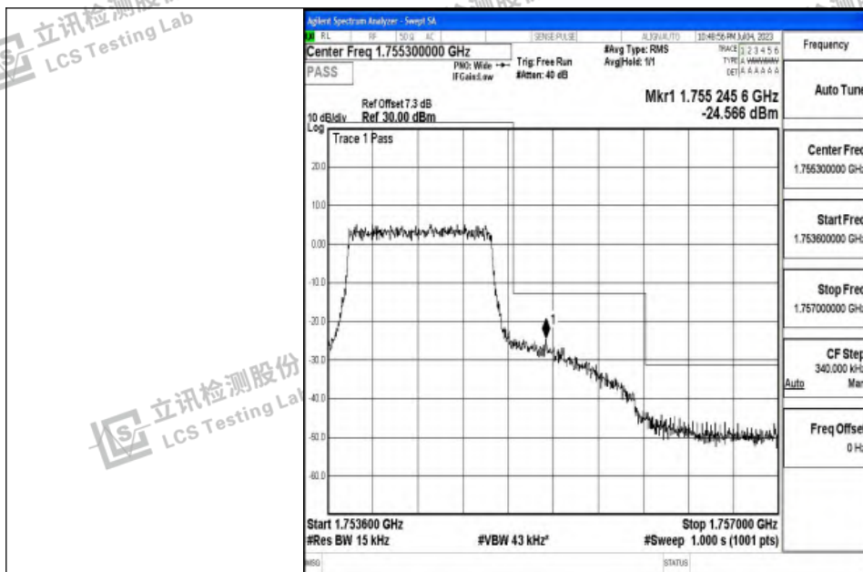
Band4_1.4MHz_QPSK_20393_6RB#0
