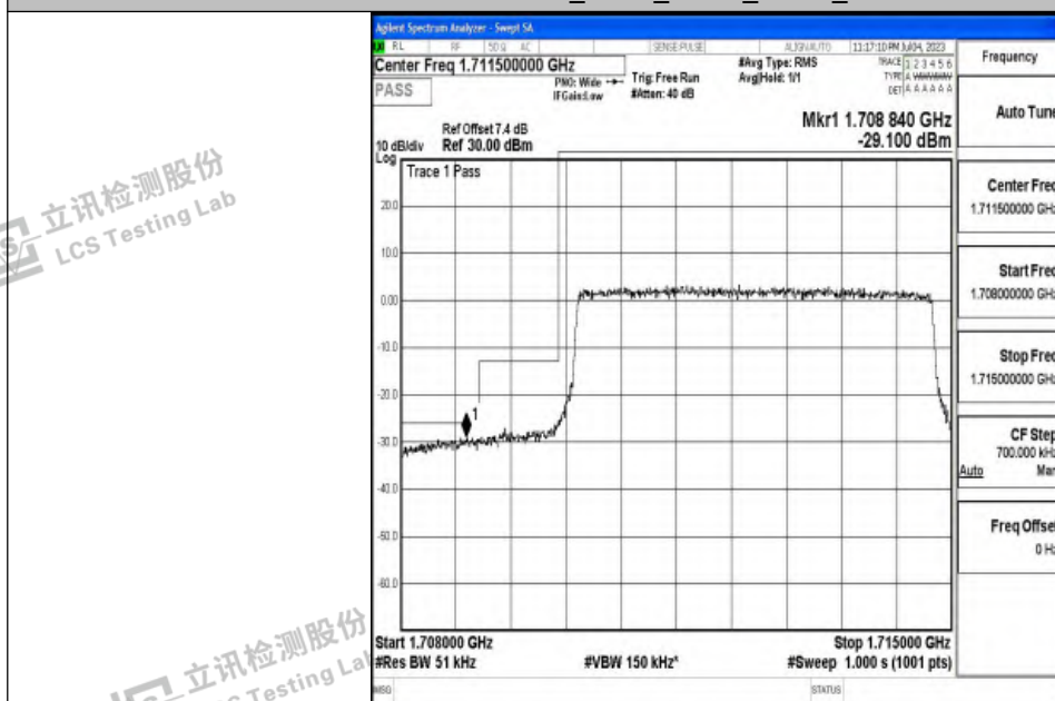
Band4_5MHz_16QAM_19975_25RB#0
