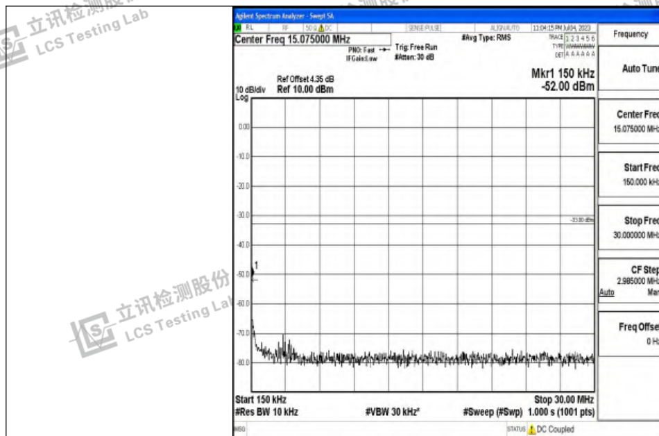
Band4_3MHz_QPSK_20175_1RB#0_0.15~30_0.15~30
