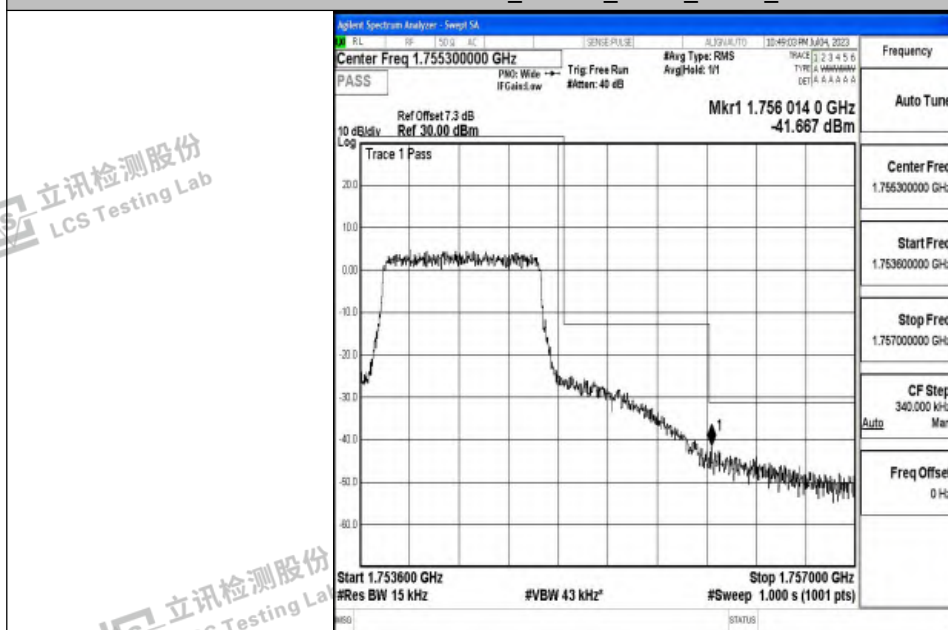
Band4_1.4MHz_16QAM_20393_6RB#0
