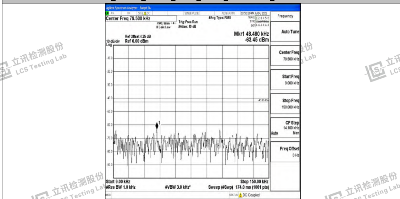
Band4_1.4MHz_QPSK_20175_1RB#0_0.009~0.15_0.009~0.15
