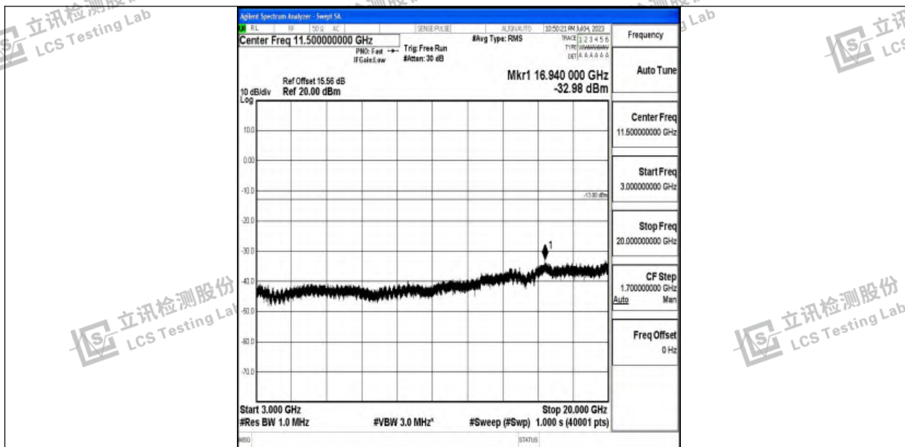
Band4_1.4MHz_16QAM_19957_1RB#0_3000~20000_3000~20000
