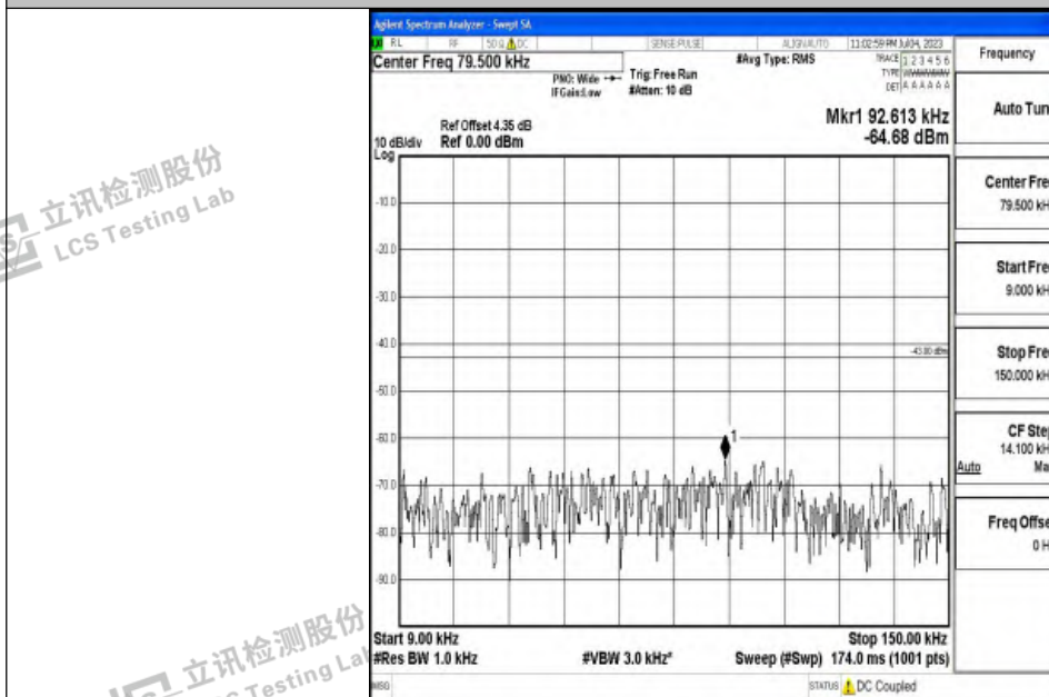
Band4_3MHz_QPSK_19965_1RB#0_0.009~0.15_0.009~0.15
