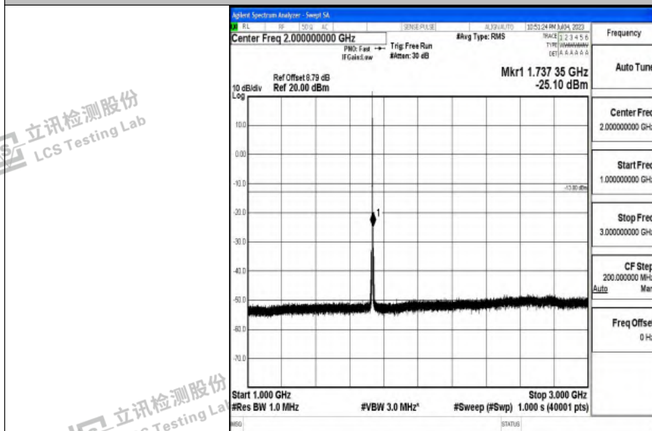
Band4_1.4MHz_16QAM_20175_1RB#0_1000~3000_1000~3000
