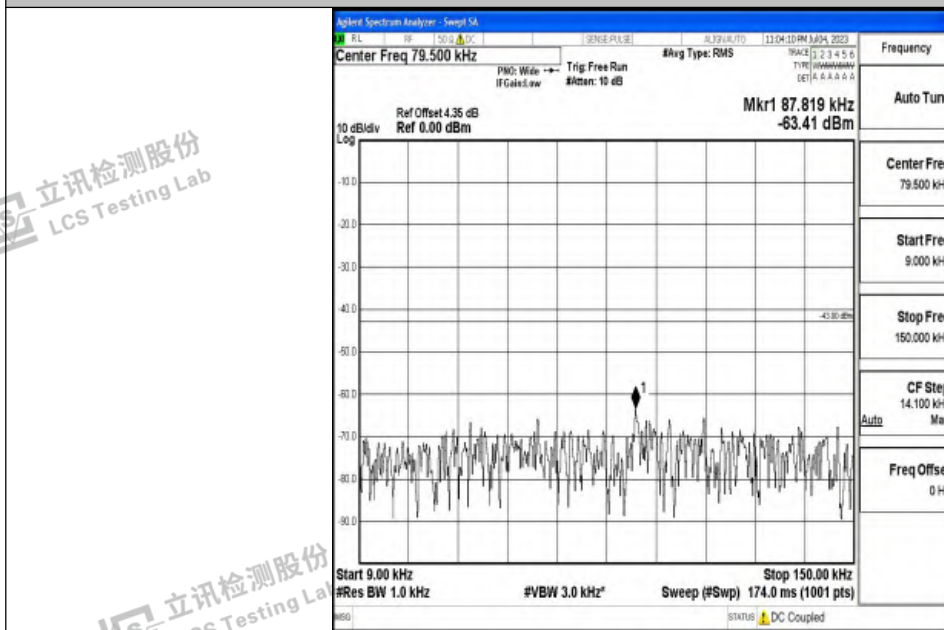
Band4_3MHz_QPSK_20175_1RB#0_0.009~0.15_0.009~0.15
