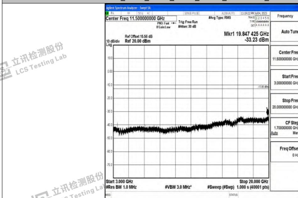
Band4_5MHz_QPSK_20175_1RB#0_3000~20000_3000~20000
