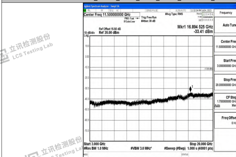
Band4_10MHz_QPSK_20000_1RB#0_3000~20000_3000~20000
