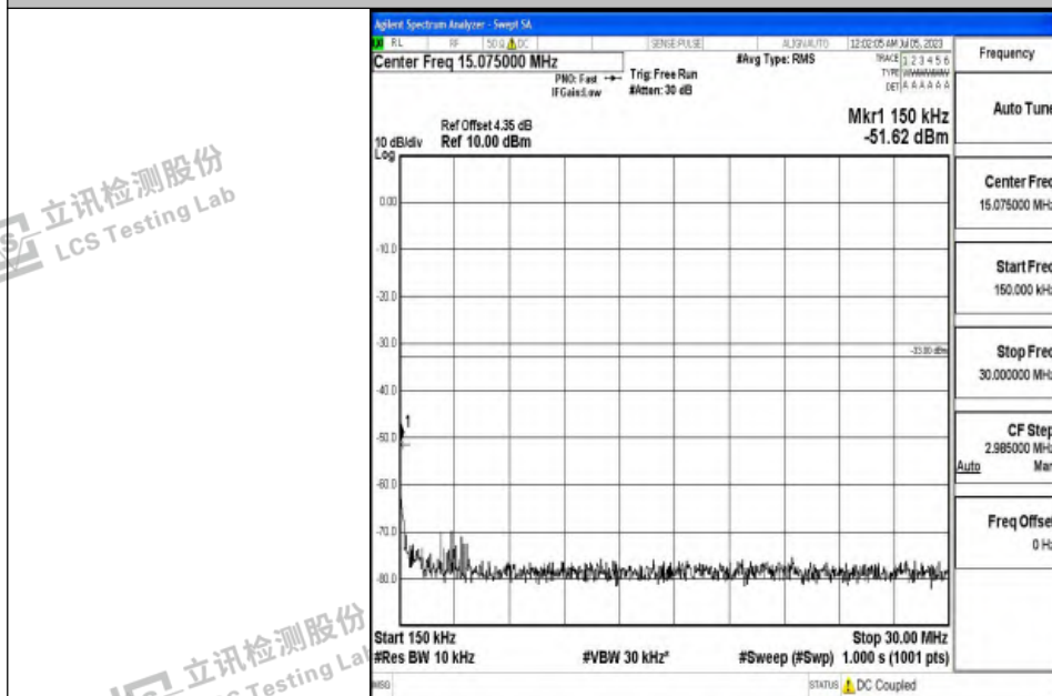
Band4_20MHz_16QAM_20300_1RB#0_0.15~30_0.15~30
