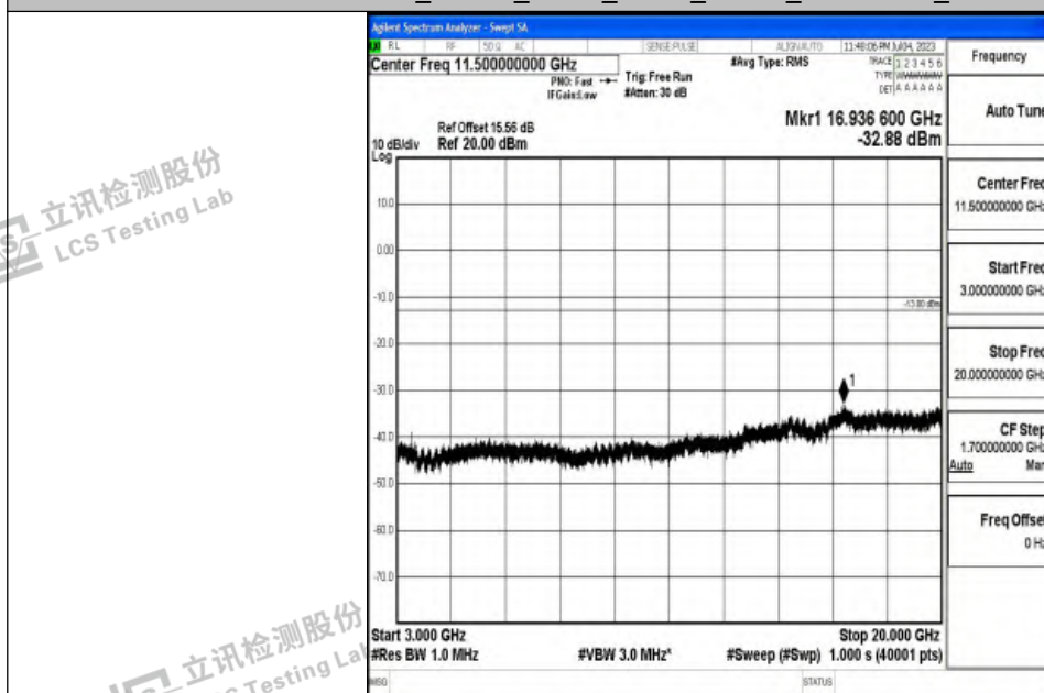
Band4_15MHz_QPSK_20325_1RB#0_3000~20000_3000~20000
