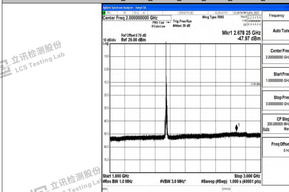
Band4_10MHz_16QAM_20350_1RB#0_1000~3000_1000~3000
