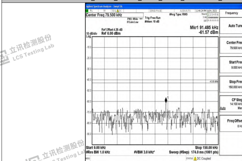
Band4_15MHz_QPSK_20175_1RB#0_0.009~0.15_0.009~0.15
