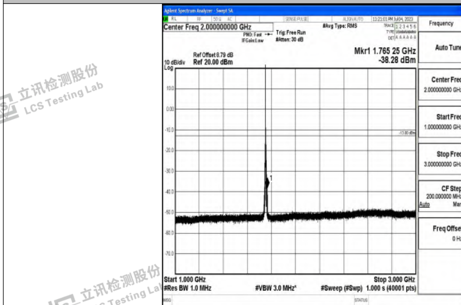
Band4_5MHz_16QAM_20375_1RB#0_1000~3000_1000~3000
