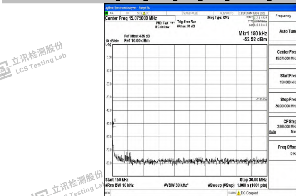
Band4_10MHz_16QAM_20350_1RB#0_0.15~30_0.15~30
