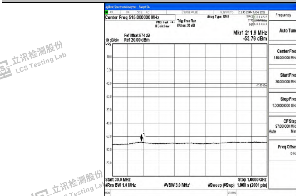
Band4_15MHz_QPSK_20025_1RB#0_30~1000_30~1000
