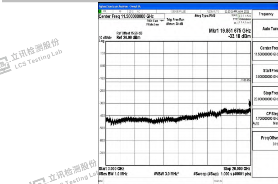
Band4_10MHz_QPSK_20175_1RB#0_3000~20000_3000~20000
