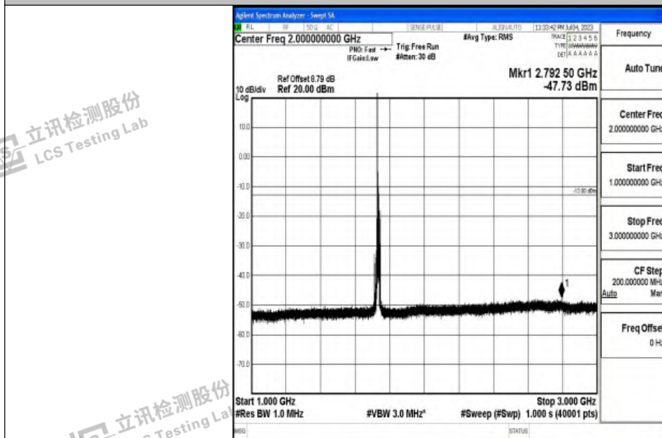
Band4_10MHz_16QAM_20175_1RB#0_1000~3000_1000~3000
