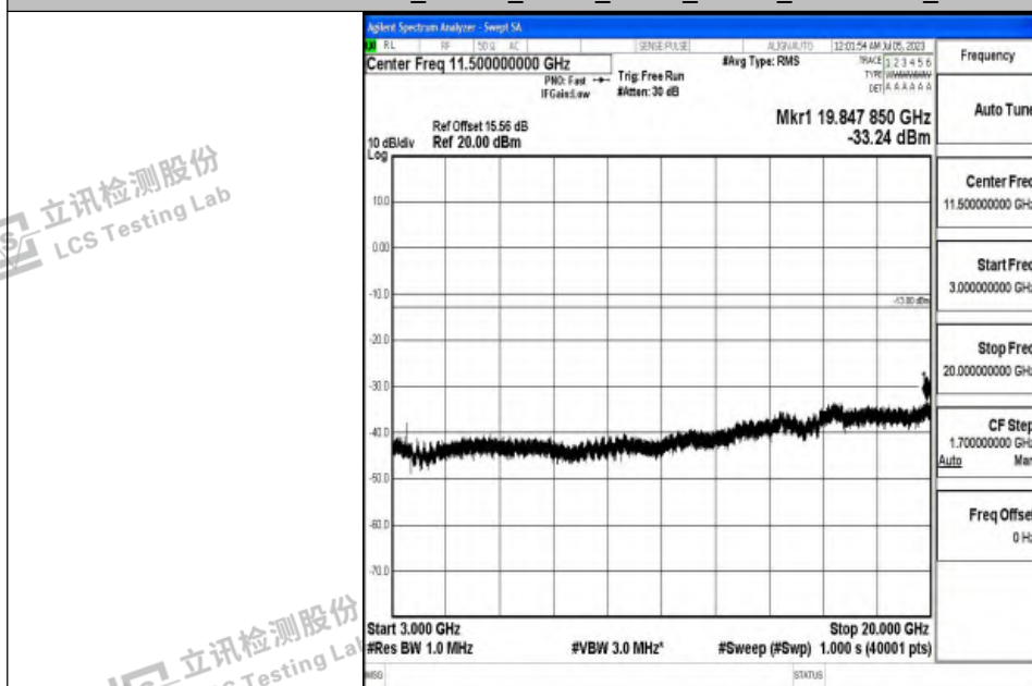
Band4_20MHz_QPSK_20300_1RB#0_3000~20000_3000~20000
