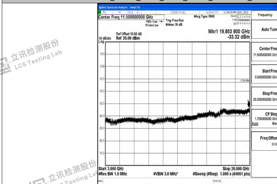
Band4_15MHz_QPSK_20175_1RB#0_3000~20000_3000~20000
