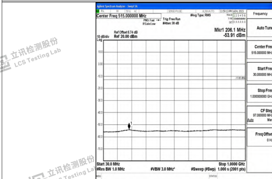
Band4_20MHz_QPSK_20050_1RB#0_30~1000_30~1000
