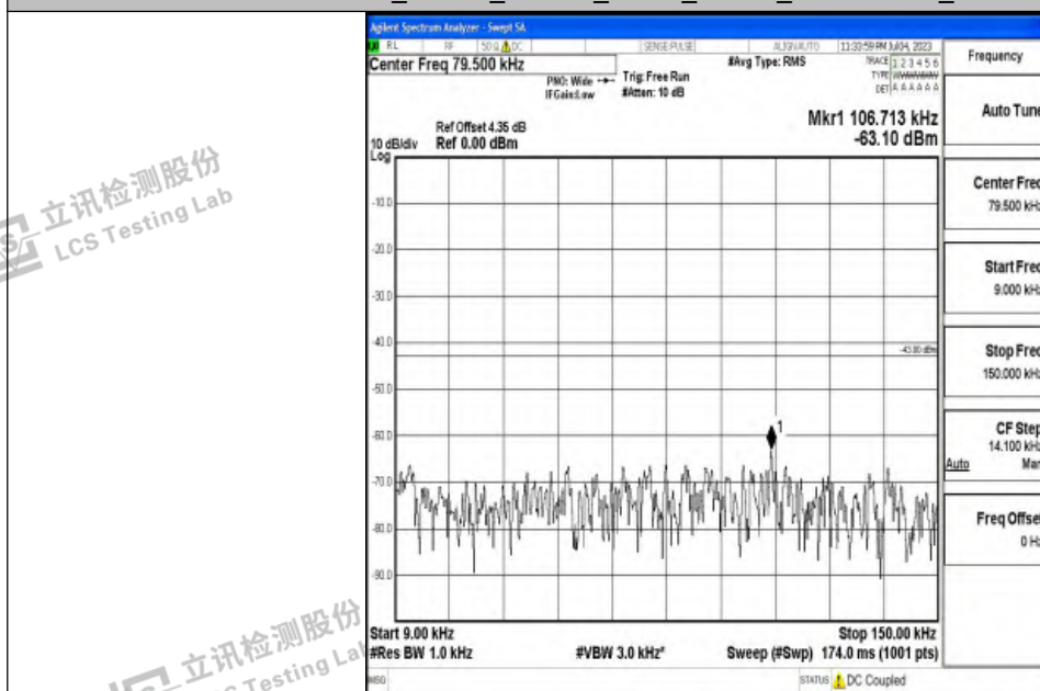
Band4_10MHz_QPSK_20350_1RB#0_0.009~0.15_0.009~0.15
