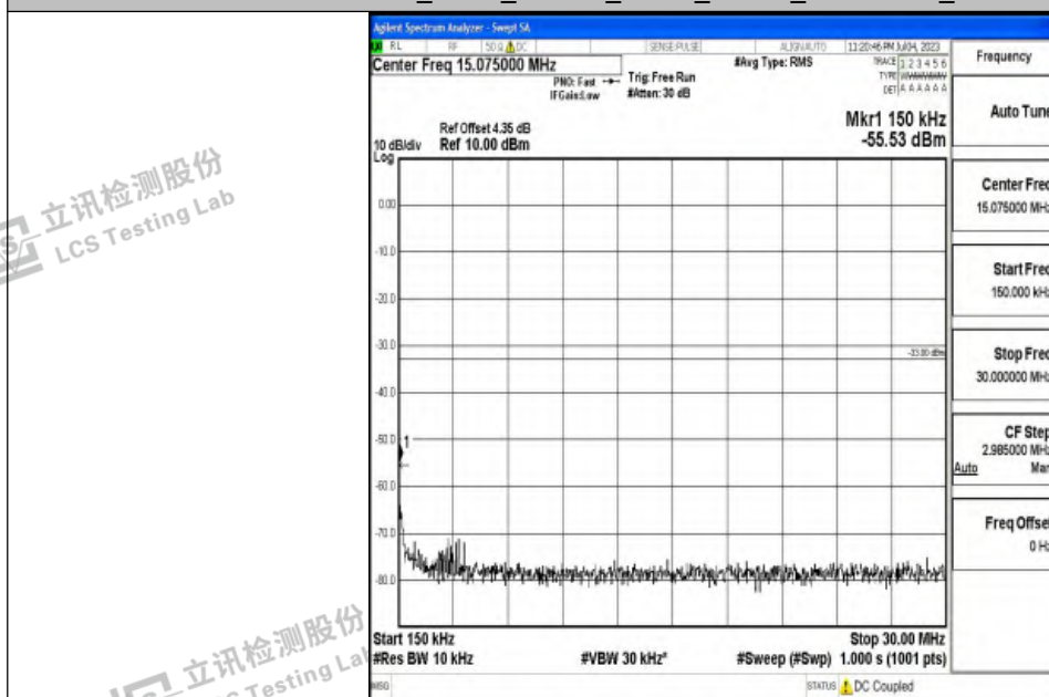
Band4_5MHz_16QAM_20375_1RB#0_0.15~30_0.15~30
