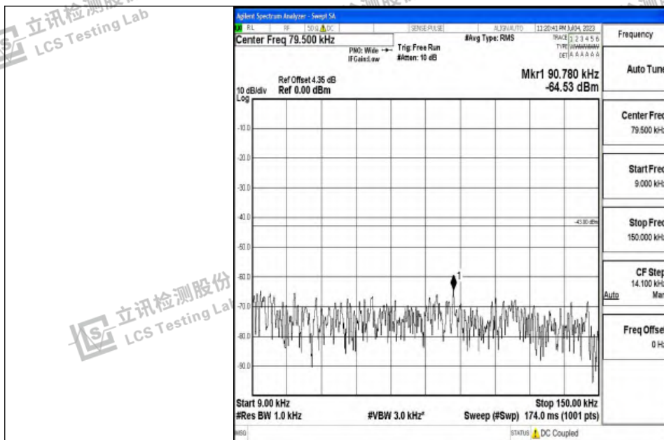
Band4_5MHz_16QAM_20375_1RB#0_0.009~0.15_0.009~0.15
