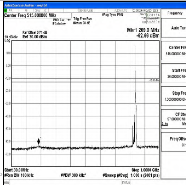
Band5_10MHz_16QAM_20600_1RB#0_30~1000_30~1000
