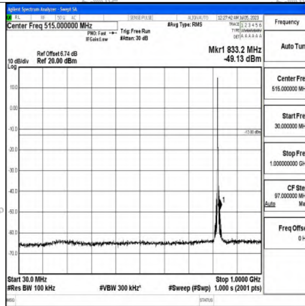
Band5_3MHz_QPSK_20415_1RB#0_30~1000_30~1000
