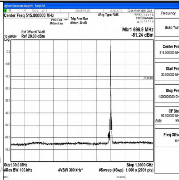
Band17_5MHz_16QAM_23790_1RB#0_30~1000_30~1000
