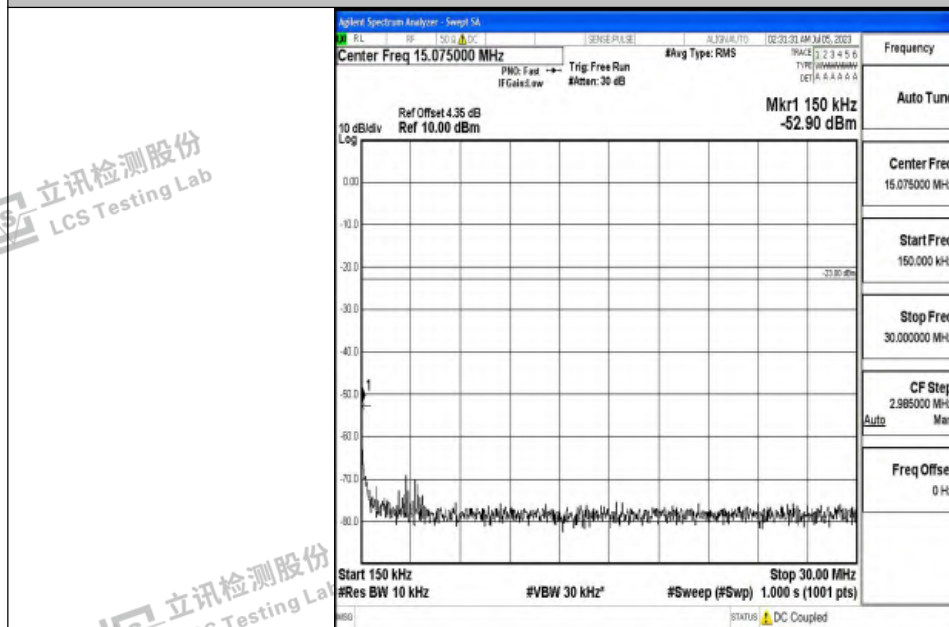
Band17_10MHz_QPSK_23790_1RB#0_0.15~30_0.15~30
