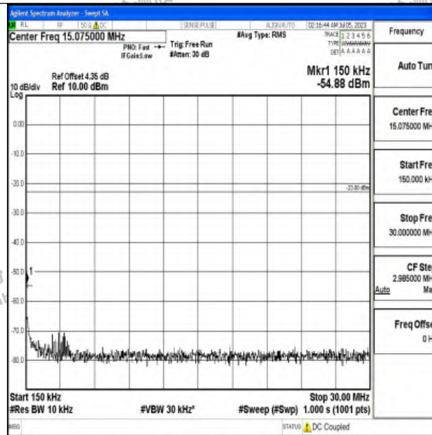
Band17_5MHz_16QAM_23790_1RB#0_0.15~30_0.15~30
