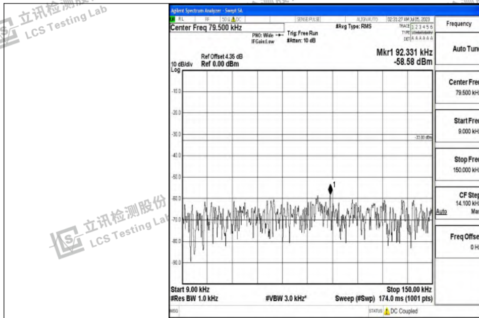
Band17_10MHz_QPSK_23790_1RB#0_0.009~0.15_0.009~0.15
