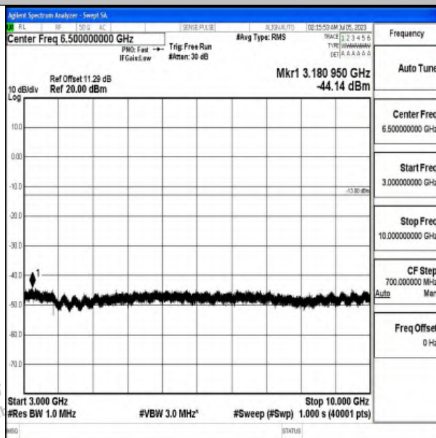
Band17_5MHz_16QAM_23755_1RB#0_3000~10000_3000~10000
