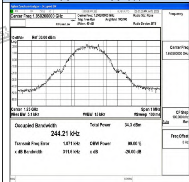
Channel 512 / 1850.2 MHz
