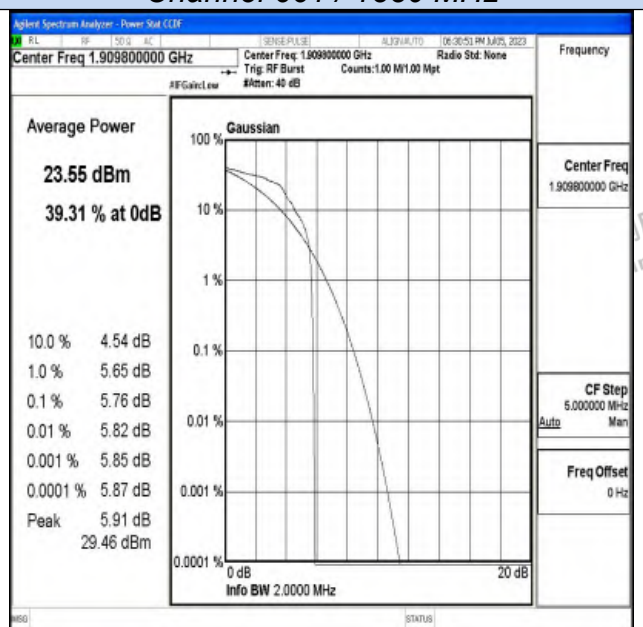
Channel 810 / 1909.8 MHz
