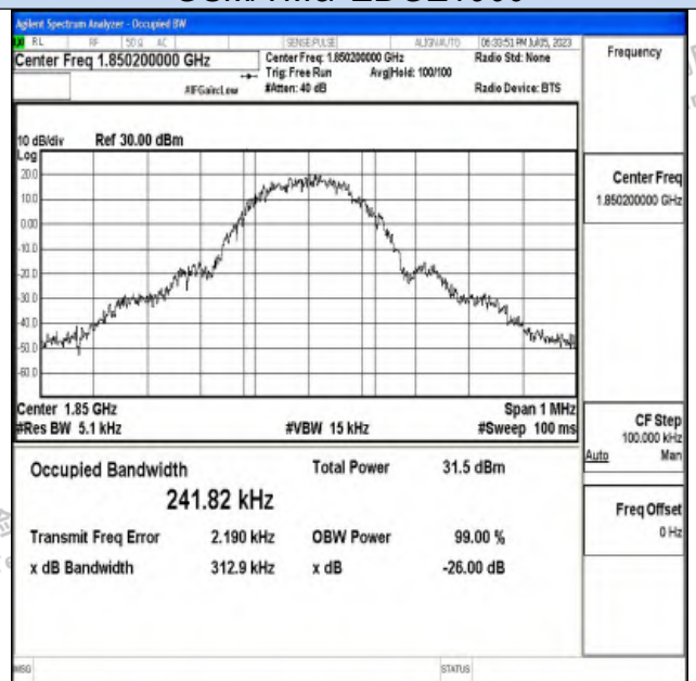
Channel 512 / 1850.2 MHz
