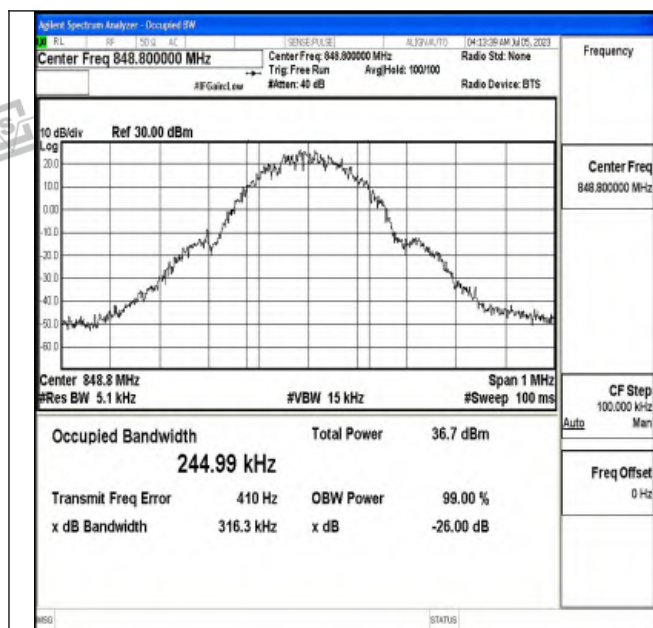
Channel 251 / 848.8 MHz
