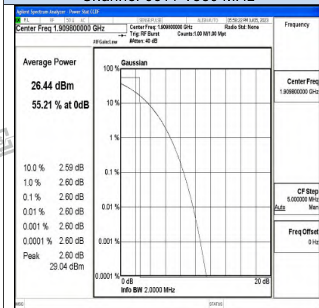
Channel 810 / 1909.8 MHz
