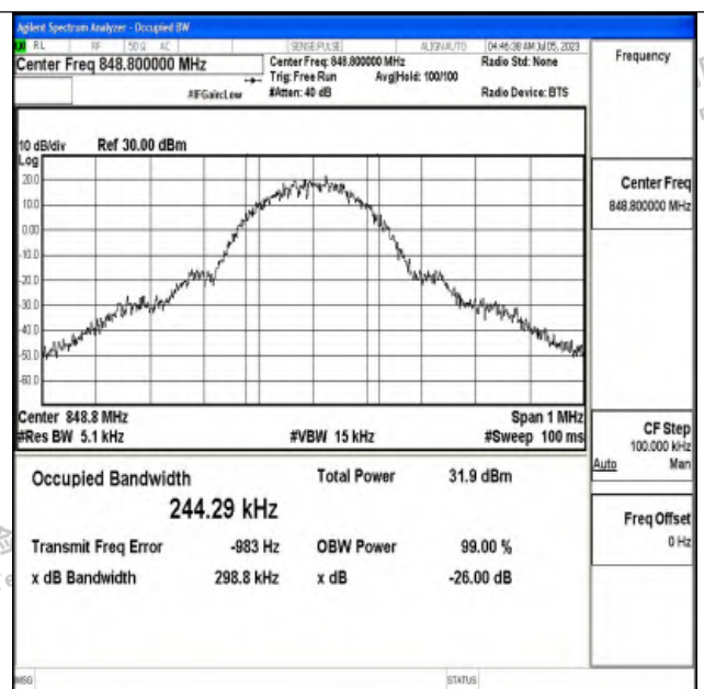
Channel 251 / 848.8 MHz
